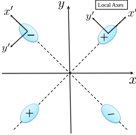
FIG. 1. The minimal model of a Weyl metal of C_{2v} crystallographic class. The Weyl nodes of opposite chiralities (shown with “+” and “-” signs) are connected by mirror reflections in the xz and yz planes. Nodes of the same chirality are connected by the time reversal symmetry. The polar C_2 axis is perpendicular to the plane of the figure.
