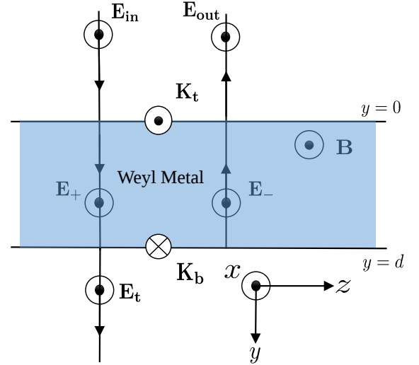
FIG. 2. Transmission of an electromagnetic wave through a slab of a Weyl metal of crystallographic class C_{4v} . The polar C_4 axis is directed along the z -axis. All waves inside and outside the slab are polarized in the x -direction. The external magnetic field \mathbf{B} is also in the x -direction. The effective surface currents on the top and bottom surfaces, \mathbf{K}_{t,b} , flow in the opposite directions.
