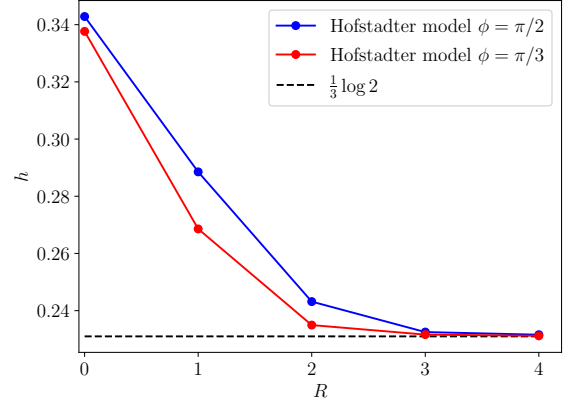
FIG. 4. h for the Hofstadter model with Chern number C = 1 . The dashed line denotes the theoretical value \frac{1}{3} \log 2 .
