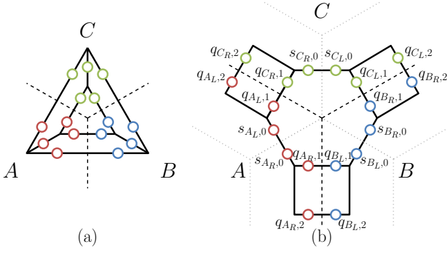
FIG. 3. (a) Toric code on a mesh covering the surface of a sphere. Degrees of freedom (0 or 1, denoted by circles) live on links, and the ground state is a uniform superposition over configurations of 0's and 1's satisfying the constraint that at each vertex, an even number of 1's must meet. (b) The configuration in (a) may be reduced to this one using local unitaries acting on A , B and C .
