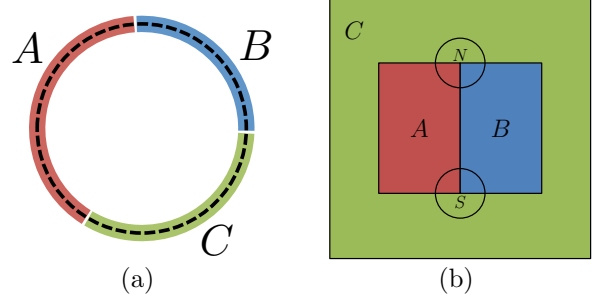
FIG. 1. (a) Tripartition of a 1D system on the circle. (b) A 2D system on a square lattice.
