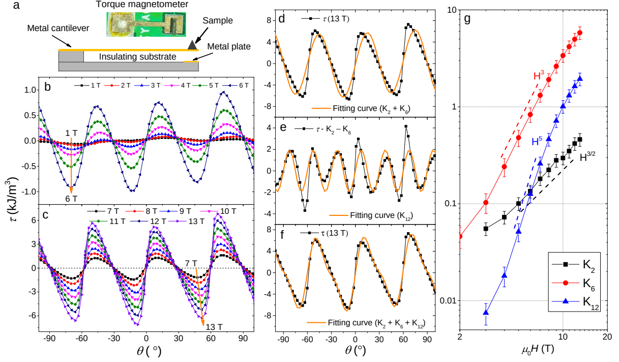
FIG. 2. Magnetic torque measurements: (a) The home-made experimental setup and its photograph (top) with a capacitive torque magnetometer, rotating the field in the xy -plane of the \text{Mn}_3\text{Sn} sample. (b) The angle dependent torque responses for magnetic fields up to 6 T. (c) The angle dependent torque responses for magnetic fields larger than 6 T. H \parallel x corresponds to 0^\circ . (d) Fit to the 13 T data with an expression, which has only a two-fold and a six-fold term ( \tau = K_2 \cdot \sin(2 \cdot (\phi + \phi_2)) + K_6 \cdot \sin(6 \cdot (\phi + \phi_6)) ). The mismatch is obvious. (e) The residual torque component after subtracting the data and the previous fit. It shows a clear twelve-fold symmetry. (f) A fit which includes an additional twelve-fold symmetry component ( K_{12} \cdot \sin(12 \cdot (\phi + \phi_{12})) ). (g) Fitting parameters K_2(H) , K_6(H) and K_{12}(H) as a function of magnetic field.
