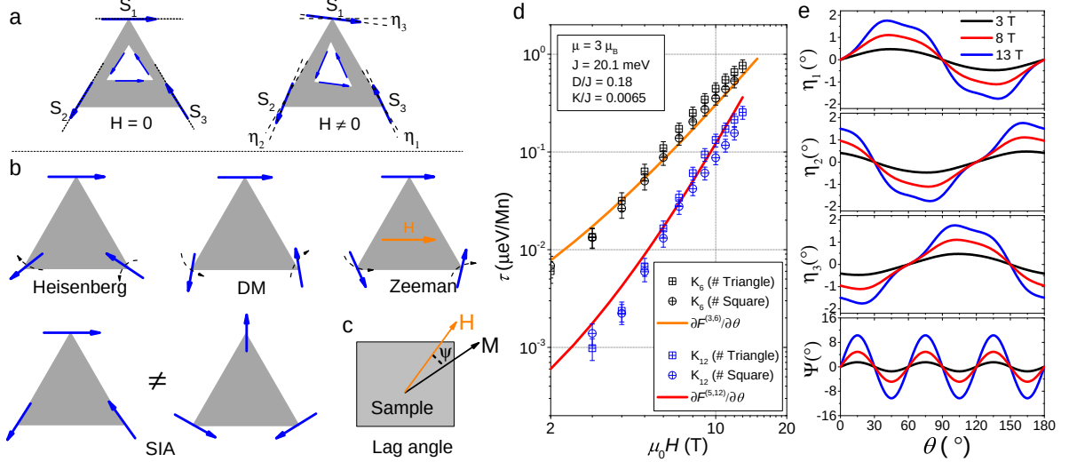
FIG. 3. Magneto-crystalline anisotropy driven by field-induced twist of non-aligned spins: (a) The magnetic field distorts the spin triangle (in white), which is no more isomorphic to the lattice triangle (in gray). The deformation angles \eta_i quantify the distortion. (b) Interaction between one spin and its immediate neighbors favor clockwise and anticlockwise twists. The Zeeman effect favors alignment of all spins with magnetic field. Single-ion anisotropy causes inequivalency between the two perpendicular orientations of the spin triangle with respect to the lattice triangle. (c) The lag angle \psi between the rotated magnetic field and the total magnetization. (d) The experimental K_6 and K_{12} (symbols) compared to theoretical expectation (solid line) using \mu = 3\mu_B , J = 20.1\text{ meV} , D/J = 0.18 , K/J = 0.0065 . (e) The deformation angles \eta_i and lag angle \psi at 3 T, 8 T and 13 T predicted by theory [32].
