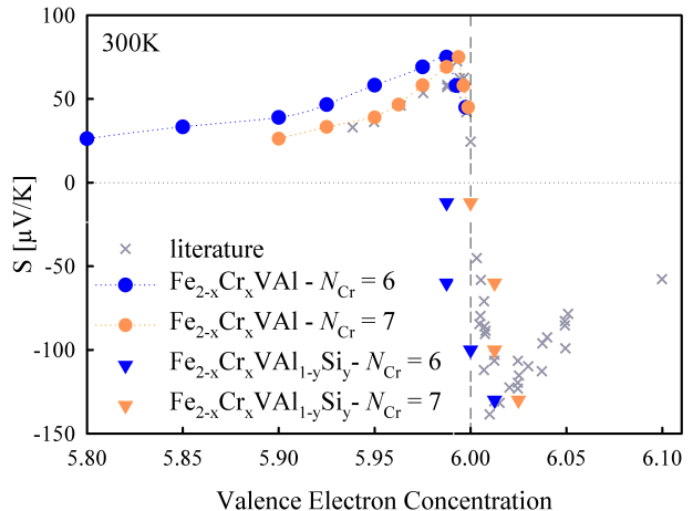
FIG. 8. Valence electron concentration dependency of the Seebeck coefficient shown for \text{Fe}_{2-x}\text{Cr}_x\text{VAL} and \text{Fe}_{2-x}\text{Cr}_x\text{VAL}_{1-y}\text{Si}_y . While an effective valence electron count N_{\text{Cr}} of 6 for Cr is conventionally expected, a count of 7 fits very well with data from other doping studies on \text{Fe}_2\text{VAL} . [9, 11, 29–40]
