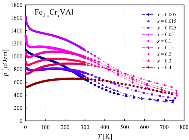
FIG. 4. Temperature-dependent electrical resistivity, \rho , of \text{Fe}_{2-x}\text{Cr}_x\text{VAI} for various concentrations x . Dashed lines are added as a visual guide.
