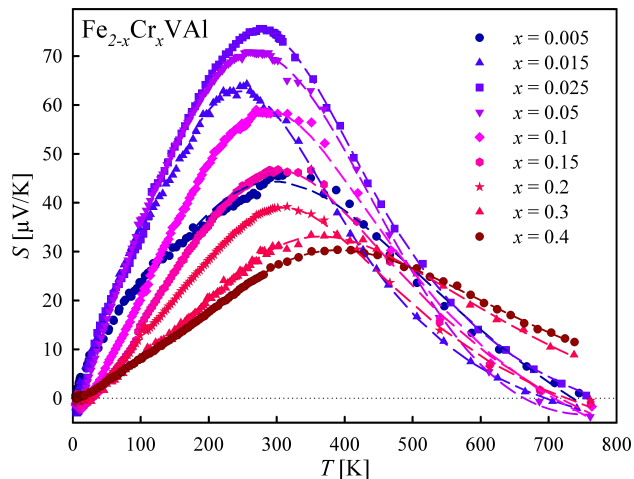
FIG. 5. Temperature dependent Seebeck coefficient measurements of \text{Fe}_{2-x}\text{Cr}_x\text{VAl} between 4 and 800 K. The dashed lines indicate a parabolic three-band model fit in the temperature range of 100 to 750 K.
