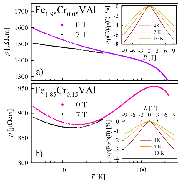
FIG. 11. Temperature dependent electrical resistivity \rho of \text{Fe}_{1.95}\text{Cr}_{0.05}\text{VAI} (a) and \text{Fe}_{1.85}\text{Cr}_{0.15}\text{VAI} (b) for external fields of 0 and 7 T. The insets show the field dependent magnetoresistance for various temperatures.
