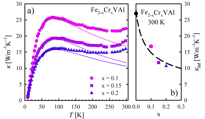
FIG. 6. (a) Temperature dependent thermal conductivity of a selection of samples of \text{Fe}_{2-x}\text{Cr}_x\text{VAl} from 4 K to room temperature. Data points in a) represent the total measured thermal conductivity. The solid lines are least squares fits as explained in the text. b) Lattice thermal conductivity for various concentrations of Cr at T = 300 K. The dashed line in b) indicates a Klemens model fit. [27] For comparison an additional data point for undoped \text{Fe}_2\text{VAl} was added.
