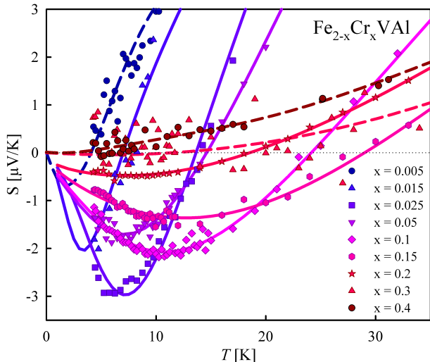
FIG. 10. Low-temperature Seebeck coefficient for \text{Fe}_{2-x}\text{Cr}_x\text{VAI} . Solid lines indicate a qualitative Kondo-model fit. Dashed lines indicate simple polynomial fits for visual clarity.
