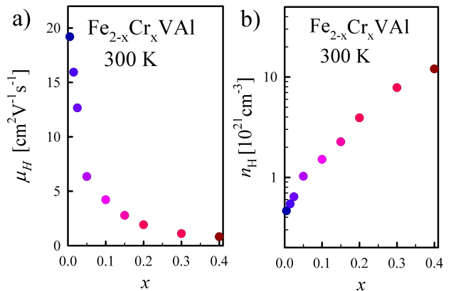
FIG. 7. Cr concentration dependence of the charge carrier mobility and density calculated from Hall-resistivity measurements at room temperature of \text{Fe}_{2-x}\text{Cr}_x\text{VAl} .
