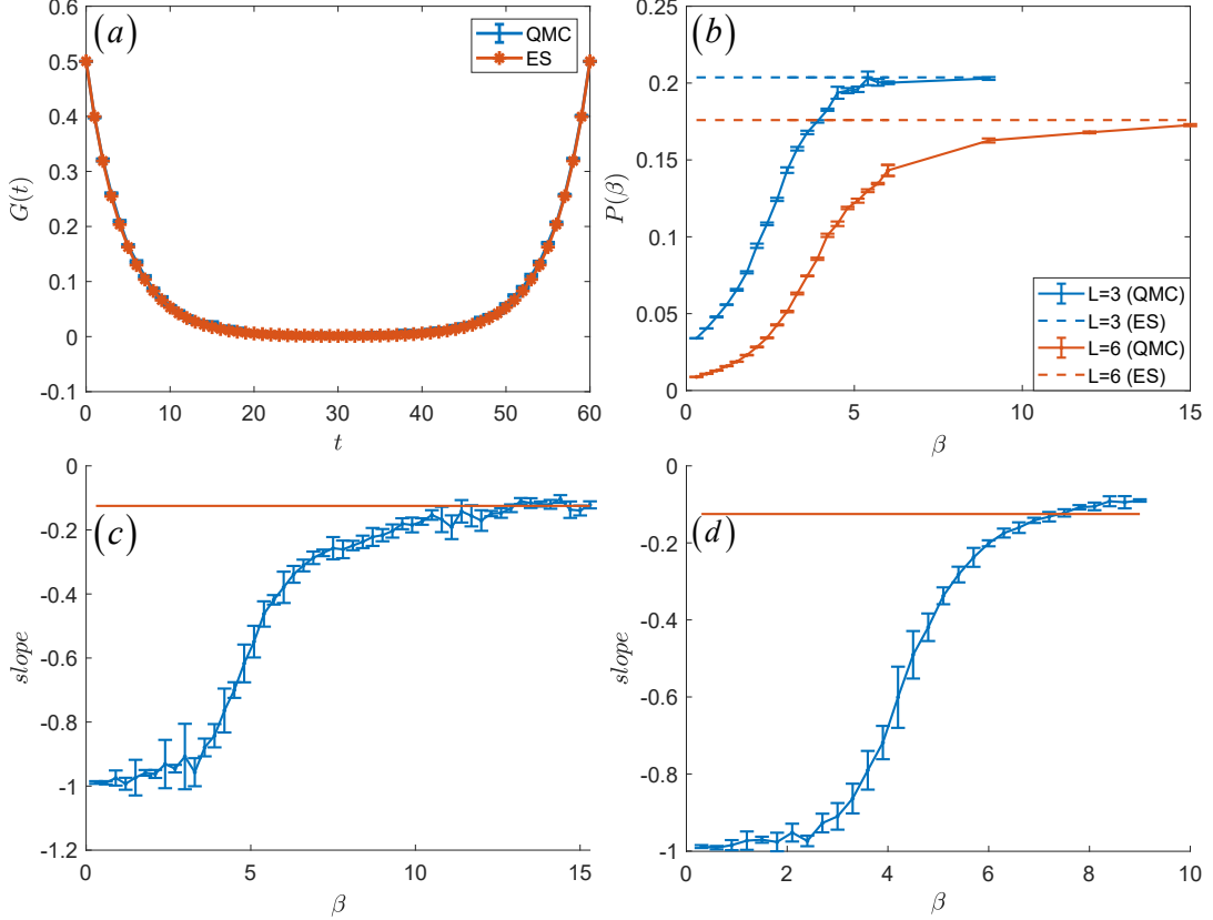
FIG. 4. Benchmark results for QMC. (a-c) are results at flat band limit, (d) is simulated with kinetic term. (a) The blue line is the single-particle Green's function for 9 \times 9 momentum mesh in mBZ with \beta = 6 at \Gamma point from QMC, while the red line is the exact solution (ES) according to Eq. (15). (b) Superconductivity pairing correlation function for 3 \times 3 and 6 \times 6 systems from QMC and ES. ES result comes from Eq. (16). (c-d) \text{slope} = \frac{d \ln(P)}{d \ln(L^2)} vs \beta at \mu = 0 . At the superconducting transition temperature, this slope shall reach -\frac{\eta}{2} = -\frac{1}{8} (the red horizontal line), in good agreement with Fig. 2(e-f) in the main text.
