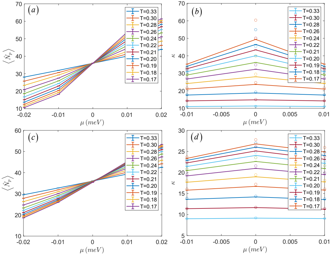
FIG. 8. Average particle number \langle \hat{N}_p \rangle versus chemical potential \mu for 6 \times 6 without kinetic term (a) and with kinetic term (c). Compressibility versus chemical potential derived from \kappa = \frac{1}{N_d} \frac{d\langle \hat{N}_p \rangle}{d\mu} (colorful lines) by numerical differentiation and \kappa = \beta \frac{\langle \hat{N}_p^2 \rangle - \langle \hat{N}_p \rangle^2}{N_d} (colorful circles) by QMC direct measurement without kinetic term (b) and with kinetic term (d).
