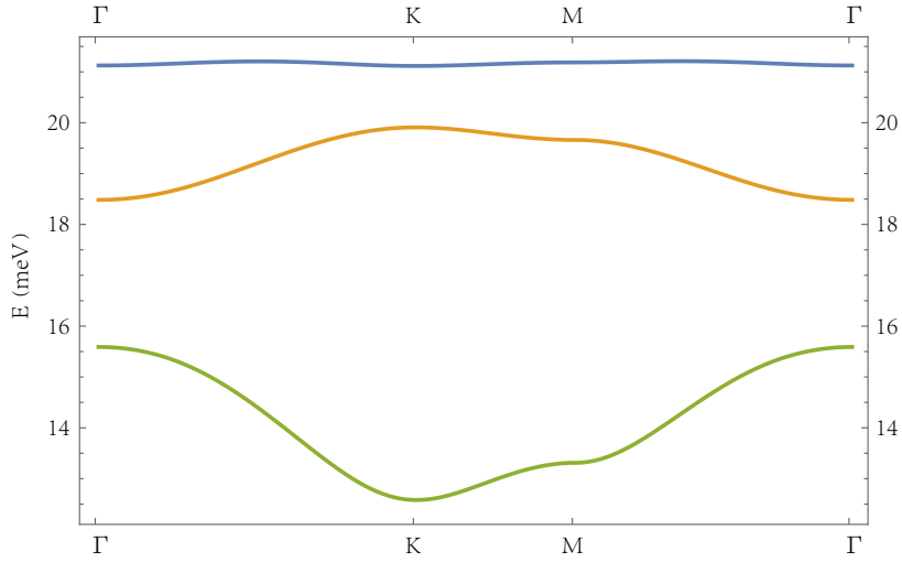
FIG. 3. Dispersion of the top three bands in mBZ.
