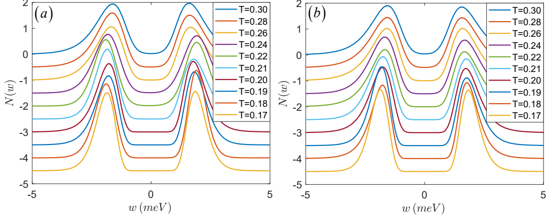
FIG. 7. DOS for 9 \times 9 at low temperature T from QMC+SAC. (a) DOS without kinetic term. (b) DOS with kinetic term.
