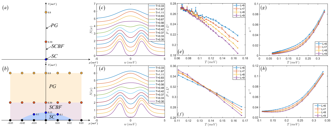
FIG. 2. QMC simulations of the flat-band limit (top row) and away from the flat-band limit (bottom row). The bandwidths of non-interacting band structures are set to 0 and 0.8meV respectively. (a-b) Phase diagrams. In the flat-band limit (a), a finite chemical potential drives the system into a trivial insulator with either empty ( \mu \ll 0 ) or complete filled ( \mu \gg 0 ) bands. In Fig. (b), the yellow/purple region is the pseudogap (PG)/ super-compressible bosonic fluid (SCBF) phase, and the blue region marks the superconducting (SC) dome. (c-d) Density of states for a 9 \times 9 system at \mu = 0 . The Cooper gap survives above the superconducting transition temperature and turns into a pseudogap above T \sim 0.3 . (e-f) Critical scaling of P \times L^\eta versus T with BKT anomalous dimension \eta = 1/4 . The crossing point of different system sizes ( L = 6, 7, 8, 9 ) marks the superconducting transition temperature: T_c \sim 0 in (e) and \sim 0.13 in (f). (g-h) Inverse of compressibility \kappa for L = 6, 7, 8, 9 at \mu = 0 . At low temperature, diverged compressibility \kappa in (g) converges in superconducting phase as shown in (h).
