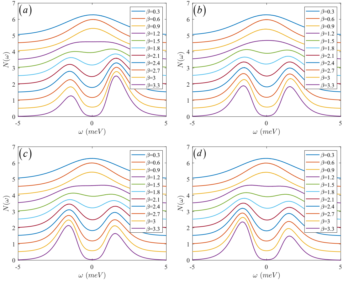
FIG. 6. DOS for 9 \times 9 with different \beta from QMC+SAC. (a)-(d) represent \mu = -0.03, 0, 0.01, 0.02 respectively.
