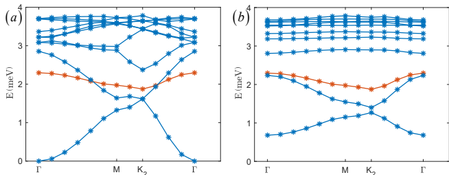
FIG. 1. Excitation spectrum for inter-valley attractive and repulsive model where the system size is 12 \times 12 and parameters come from VIA. (a) Single-particle excitation (red line) and Goldstone excitation (blue lines) along high symmetry line for inter-valley attractive model. (b) Single-particle excitation (red line) and gapped charge neutral excitation (blue lines) along high symmetry line for inter-valley repulsive model.
