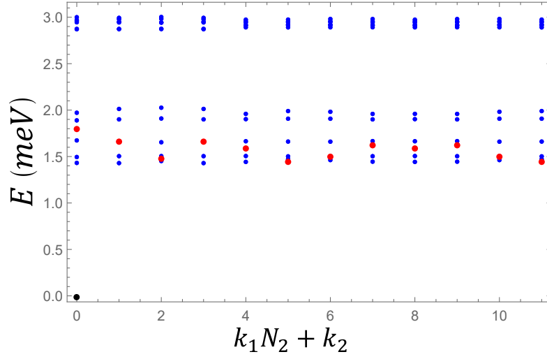
FIG. 5. ED results for 3 \times 4 system at particle number N = 12 and N = 11 . Black point represents ground state, red points are single-particle excitations and blue points are all one-charge excitations.
