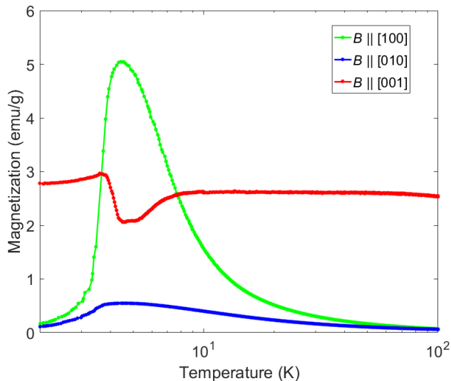
FIG. 3. Logarithmic temperature dependence of the magnetization. The measurements were performed at temperatures from 2 to 100 K after pre-cooling the sample to 2 K in zero magnetic field. At 2 K, the hysteresis was measured in fields of \pm 5 T; after that, the field was decreased to 0.01 T and the temperature dependence of the magnetization was measured. Of particular interest is the temperature range of 3.5–8 K corresponding to the spin-reorientation transition.
