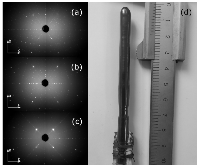
FIG. 2. (a, b, c) Lauegrams of the \text{TbFeO}_3 single crystal along different crystallographic directions corresponding to sp. gr. Pbnm with lattice parameters of a = 5.326 Å, b = 5.602 Å, and c = 7.635 Å. (d) Photograph of the single crystal obtained by optical floating zone melting.
