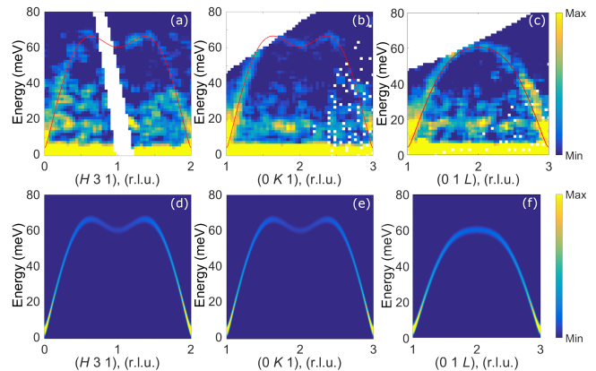
FIG. 4. Cuts along the three characteristic directions of the reciprocal space. (a-c) Experimental INS spectra recorded at a temperature of 2 K. The data were obtained by summation of the symmetric directions and smoothed with a Gaussian. The integration limit is \pm 0.1 r.l.u. The calculated dispersion curves (red) are superimposed. (d-f) Model calculation of the spectra within the selected model.
