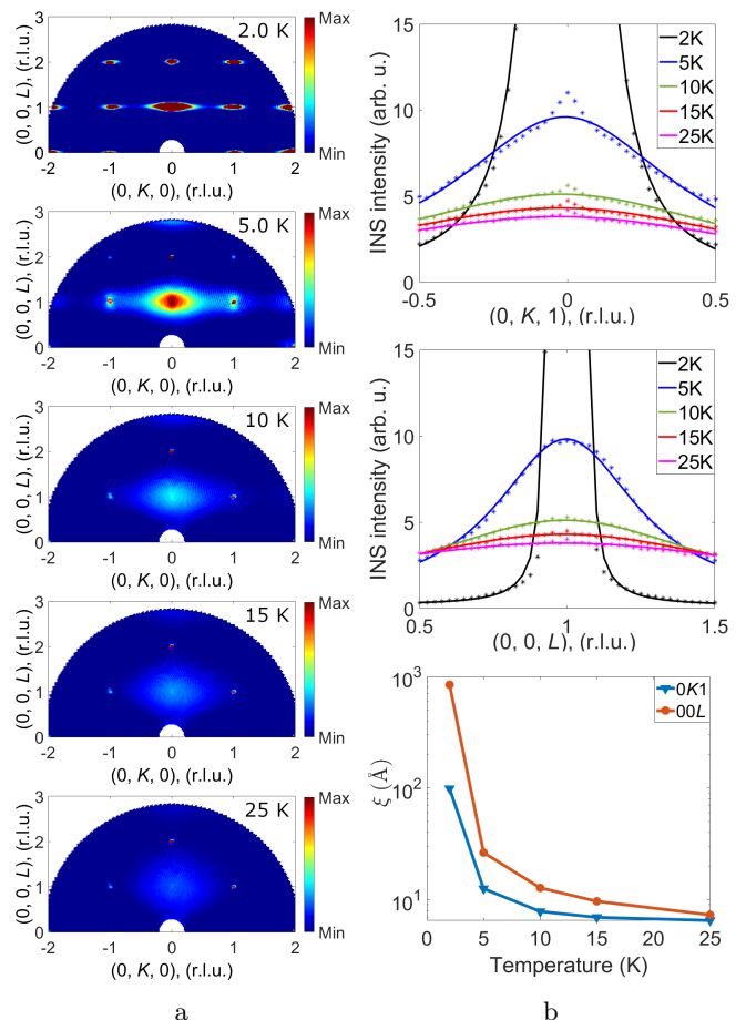
FIG. 7.(a) Experimental data integrated over the H directions of the reciprocal space in the limit \pm 0.1 r.l.u. The energy axis was integrated within \pm 0.1 meV. The cuts made at different temperatures in ascending order are arranged from up to down. (b) Experimental data integrated over the directions of the reciprocal space in the limit \pm 0.15 r.l.u. The energy axis was integrated within \pm 0.1 meV. Result of the approximation of the experimental data by the convolution of the Lorentzian and Gaussian functions. The resolution was estimated from the structural peak width using two characteristic directions of the reciprocal space. The temperature dependence of the correlation length for both directions of the reciprocal space is shown in the bottom.
