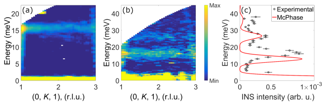
FIG. 6. (a, b) Cuts along the highly symmetric directions. The measurements were performed at 2 K. The data were obtained by summation of the symmetric directions. The integration limit is \pm 0.1 r.l.u. The spread operation was also used. The CEF level at 16–17 meV can be clearly seen in (a). In (b), there are two crystal field levels at 16–17 and 26 meV; around 34 meV, there is a hint of another CEF level, but it cannot be established with confidence. (c) Comparison of the integral CEF values with the calculation within the single-ion model in the McPhase software. The experimental data and the spin dynamics calculated using the PCM are in good agreement. The integration limit is \pm 0.25 r.l.u.
