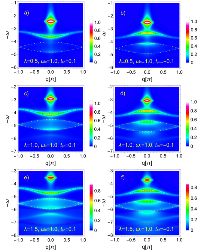
Figure 3: A(\omega, q) for different \lambda and t_{\text{ph}} as denoted in the insets. In a) through f) blue dashed lines follow single-phonon excitation and are obtained from \omega_{1\text{ph}} = -E_{q=0}^{(0,1)} + \omega_0 + 2t_{\text{ph}} \cos(q) , yellow dot-dashed lines enclose continuum of 2-phonon excitations below the polaron ground state energy: \omega_{2\text{ph}}^\pm = -E_{q=0}^{(0,1)} + 2\omega_0 \pm 4t_{\text{ph}} \cos(q/2) . In addition, red dashed lines indicate the regime of three phonon excitation continuum \omega_{3\text{ph}}^\pm , as given in the text. We have used artificial broadening \eta = 0.05 . Note that the lowest frequency (lowest |\omega| ) peaks at q = 0 are represented by the Lorentzian forms of the delta functions in q and \omega . Identical colour coding has been used in all panels.
