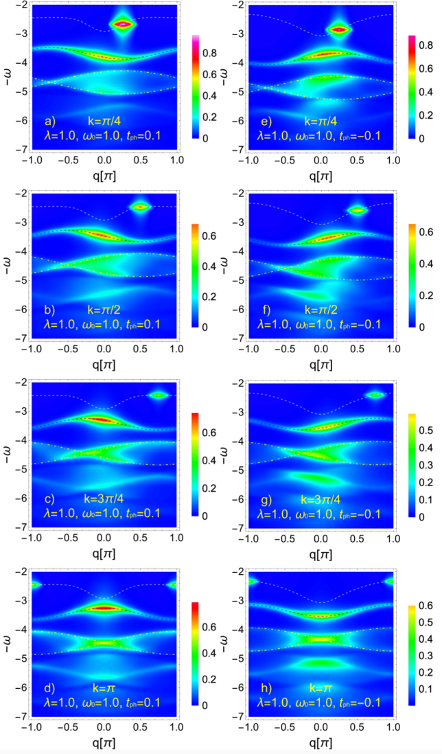
Figure 4: A(\omega, q, k) computed at t_{\text{ph}} = 0.1 from a) through d) and t_{\text{ph}} = -0.1 from e) through h), for different values of k as denoted in the insets. In a) through e) blue dashed lines follow single-phonon excitation and are obtained from \omega_{1\text{ph}} = -E_k^{(0,1)} + \omega_0 + 2t_{\text{ph}} \cos(q-k) , yellow dot-dashed lines enclose the continuum of 2-phonon excitations below the polaron ground state energy: \omega_{2\text{ph}}^\pm = -E_k^{(0,1)} + 2\omega_0 \pm 4t_{\text{ph}} \cos((q-k)/2) . White dashed lines represent the polaron dispersion relation given by \omega_{\text{pol}} = -E_k^{(0,1)} . We have used artificial broadening \eta = 0.05 . Note that the lowest frequency (lowest |\omega| ) peaks at q = 0 are represented by the Lorentzian forms of the delta functions in q and \omega . Identical colour coding has been used in all panels.
