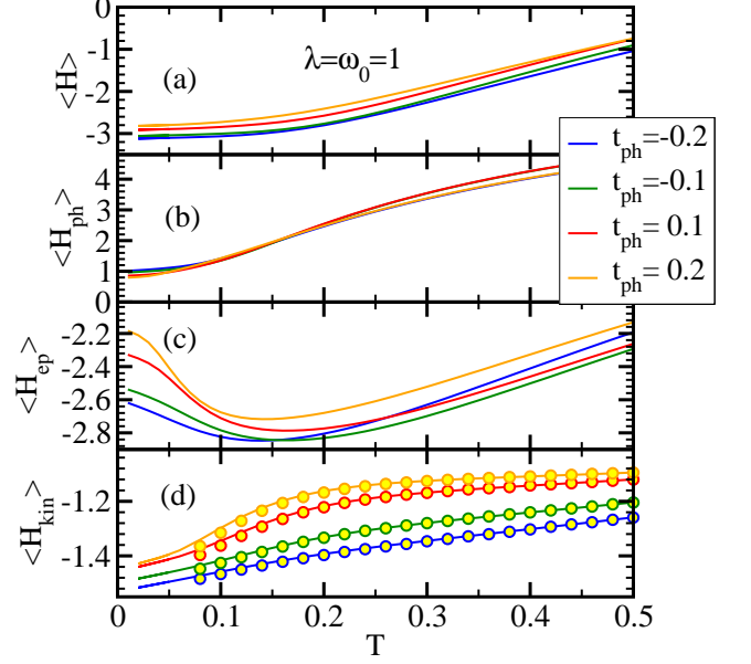
Figure 5: Temperature dependence of \langle H \rangle , \langle H_{\text{ph}} \rangle , \langle H_{\text{ep}} \rangle , and \langle H_{\text{kin}} \rangle in (a) through (d) for different values of t_{\text{ph}} as indicated in the inset. In (d) circles present results obtained from spectral function frequency sum-rules using Eqs. 9 and 10.
