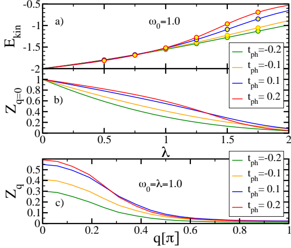
Figure 2: Full lines in a) represent E_{\text{kin}} of the polaron ground state at various t_{\text{ph}} and the total wavevector q = 0 , open circles represent the same quantity computed using E_{\text{kin}} = -2t_{\text{el}} \sum_q \bar{n}_q \cos(q) . The quasiparticle weight Z_{q=0} vs. \lambda is represented in b) and c) represents Z_q at fixed \lambda = 1 .
