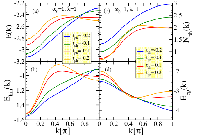
Figure A1: Zero- T results vs. k : a) the polaron dispersion relation: E(k) = \langle \psi_k^{(0,1)} | H | \psi_k^{(0,1)} \rangle , b) the kinetic energy: E_{kin}(k) = \langle \psi_k^{(0,1)} | H_{kin} | \psi_k^{(0,1)} \rangle , c) the total number of phonons in the system: N_{ph}(k) = \langle \psi_k^{(0,1)} | \sum_j a_j^\dagger a_j | \psi_k^{(0,1)} \rangle , and d) the electron-phonon coupling E_{ep}(k) = \langle \psi_k^{(0,1)} | g \sum_j n_j (a_j + a_j^\dagger) | \psi_k^{(0,1)} \rangle .
