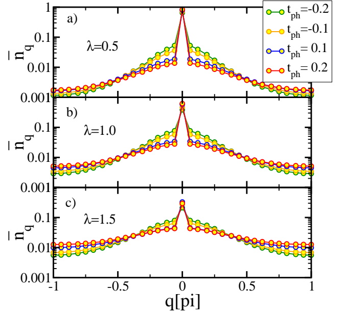
Figure 1: \bar{n}_q for different values of \lambda as denoted in insets and for different values of the phonon dispersion t_{\text{ph}} , computed in the polaron ground state. In this and in all subsequent figures unless otherwise specified we have used \omega_0 = t_{\text{el}} = 1 , N_h = 16 and the size of the system L = 32 .
