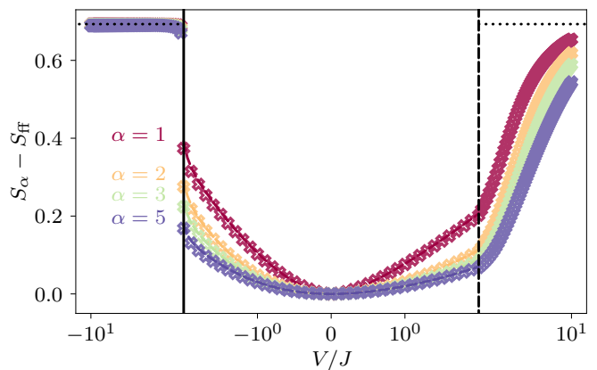
FIG. 5. One-particle Rényi entanglement entropy S_\alpha for different values of the Rényi index \alpha as a function of the interaction strength V/J where S_{\text{ff}} is the 1-particle entropy for free fermions. The crosses are obtained using DMRG for N = 51 on a lattice of L = 102 sites. Solid lines depict extrapolation to the thermodynamic limit from ED and DMRG data, and dashed horizontal lines show theory predictions for |V/J| \rightarrow \infty . Phase transitions in the J - V model are marked with vertical lines at V/J = \pm 2 .
