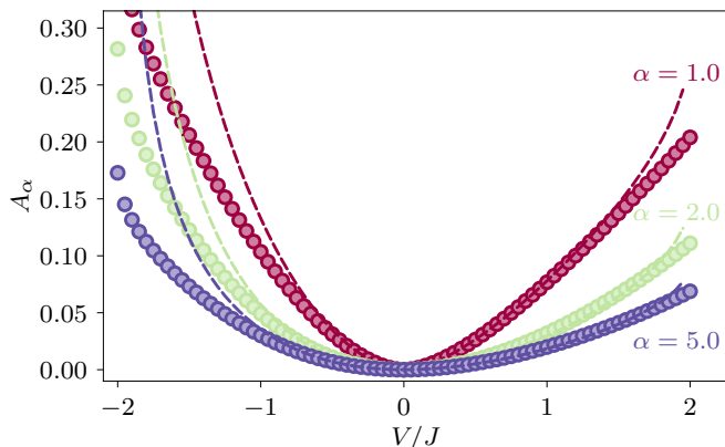
FIG. 7. Interaction strength V/J dependence of the constant contribution to the 1-particle Rényi entanglement entropies extrapolated to the thermodynamic limit A_\alpha for Rényi indices \alpha = 1, 2 , and 5 together with the prediction from bosonization for a fixed interaction cutoff \epsilon = 0.84 . We find very good agreement between the Luttinger liquid prediction and the numerical results for the J - V model in region V/J \in [-0.5, 1.5] .
