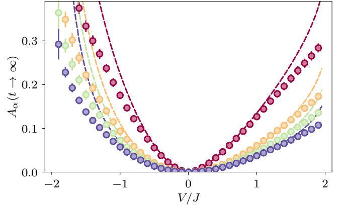
FIG. 12. 1-particle entanglement entropies extrapolated from the numerical steady state estimates to the thermodynamic limit as a function of the post quench interaction strength V/J (circles) for Rényi indices \alpha = 1 (red), \alpha = 2 (yellow), \alpha = 3 (green), and \alpha = 5 (blue). Dashed lines depict the corresponding theory predictions from the steady states after the quench in the Luttinger liquid model using a fixed interaction cutoff \varepsilon = 0.84 obtained from ground state calculations. Similar to the equilibrium case, we find good agreement between LL prediction and numerical data for moderate interaction strengths.
