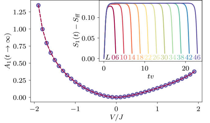
FIG. 9. Thermodynamic limit growth of the 1-particle von Neumann entanglement entropy as a function of the interaction strength V/J after the quantum quench at t = 0 obtained from the Luttinger liquid steady state limit (red, dashed line) in Eq. (76). Blue circles show the result of finite size scaling of the plateau values shown in the inset. The inset depicts the first plateau of the entanglement entropy obtained by numerical integration from the time dependent one body density matrix in Eq. (74) for several system sizes L = 2N . We observe that the plateau size increases linearly with L while the region where the entropy increases to the plateau and the time scale where it drops from the plateau is independent of the system length. In the thermodynamic limit, the average of the entropy and the plateau values agree with each other. The main panel demonstrates that the plateau value of the entropy coincides with the entropy obtained from the steady state result for the 1-RDM in the thermodynamic limit.
