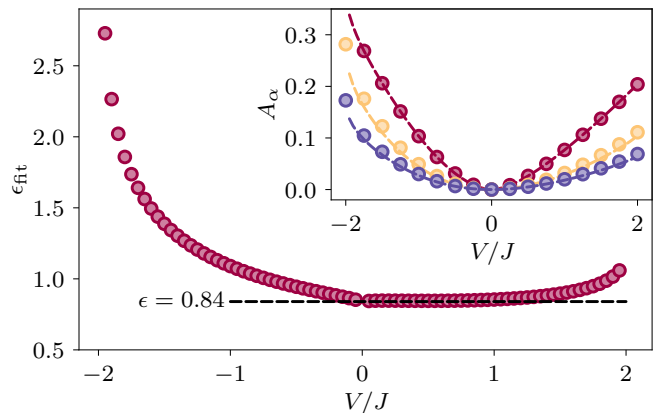
FIG. 8. Effective interaction cutoff \epsilon_{\text{fit}} as a function of the interaction strength V/J (red circles) obtained by fitting the Luttinger liquid prediction for the one-particle von Neumann entanglement entropy for each interaction strength individually to the numerical data of the J - V model. We find an extended flat region of the effective cutoff \epsilon = 0.84 (dashed, black line) that is nearly independent of interaction strength. The inset depicts numerical results for the Rényi entropies with \alpha = 1 (red circles), \alpha = 2 (yellow circles), and \alpha = 5 (blue circles) together with the field theory prediction using the fitted interaction dependent cutoff \epsilon_{\text{fit}} .
