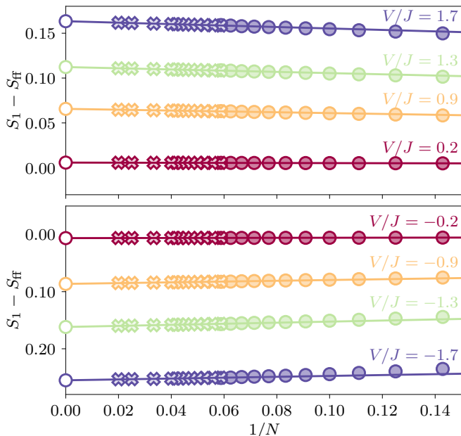
FIG. 6. Finite size scaling of the equilibrium one-particle von Neumann entanglement entropy S_1 for various interaction strengths V/J where the free fermion contribution S_{\text{ff}} has been subtracted. Results obtained with DMRG (crosses) and ED (circles) are shown together along with a linear extrapolation to the thermodynamic limit 1/N \rightarrow 0 . ED provides access to lattices at half filling with up to N = 19 fermions and using DMRG lattices with more than N = 51 fermions can be studied.
