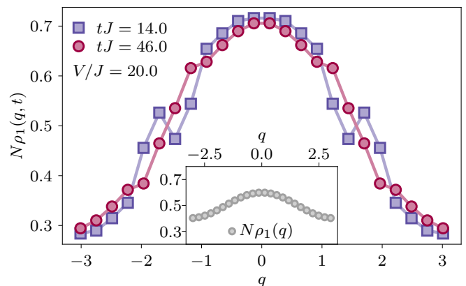
FIG. 16. Momentum distribution function at two different times, after a quantum quench at t = 0 to a final interaction strength V/J = 20 deep in the density wave phase. The system consists of N = 12 fermions on a ring of L = 24 sites. The inset shows the equilibrium ground state distribution function for the same interaction strength. Lines are a guide to the eye.
