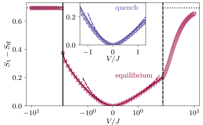
FIG. 1. Interaction dependence of one particle von Neumann entanglement entropy S_1 obtained numerically from the J - V model and from an effective low energy Luttinger liquid calculation (dashed lines) with a fixed interaction cutoff. Here, S_{\text{ff}} is the entropy for free fermions. The main panel depicts the equilibrium ground state entropy with numerical data from DMRG for a system of L = 102 lattice sites at half filling (crosses). The solid line represents finite size scaling of numerical data to the thermodynamic limit. The excellent agreement with the finite size DMRG data shows that the system with N = 51 fermions is large enough to describe the thermodynamic limit accurately in the whole LL phase. The inset depicts finite size exact diagonalization results for N = 12 fermions on L = 24 sites after an interaction quantum quench (circles) in the asymptotic steady state. The solid line shows the thermodynamic limit of the numerical data obtained from finite size scaling the time averaged one particle entropy (circles) after the interaction quench. The dashed line is the result of non-equilibrium bosonization using the same value of the interaction cutoff as in the main panel.
