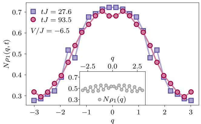
FIG. 3. Momentum distribution function at two different times, after a quantum quench at t = 0 to a final interaction strength V/J = -6.5 deep in the phase separated clustered solid. The system consists of N = 12 fermions on a ring of L = 24 sites. The inset shows the equilibrium ground state distribution function which demonstrates pronounced oscillations due to the existence of a short momentum scale resulting from large clusters of N fermions. Lines are a guide to the eye.
