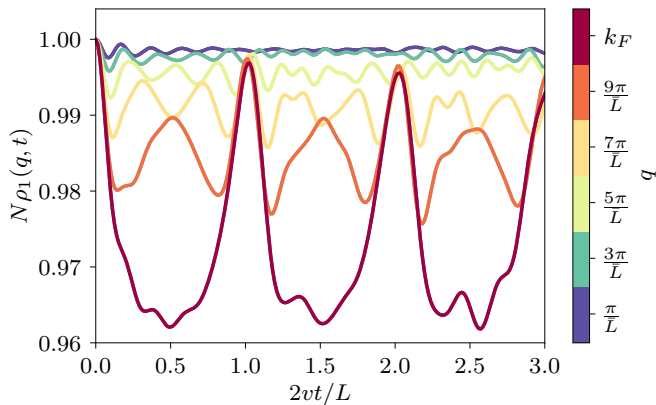
FIG. 2. Dependence of eigenvalues of the one body density matrix \rho_1 on the rescaled waiting time 2vt/L after the quantum quench computed via exact diagonalization for a final interaction strength V/J = -0.5 . We show a quarter of the spectrum with 0 < q < k_F for a system of N = 12 fermions on L = 24 lattice sites. The largest contributions to the one particle entanglement entropy come from the eigenvalues close to the Fermi levels which show the largest oscillation amplitude and the recurrence time L/(2v) that appears in the entropy.
