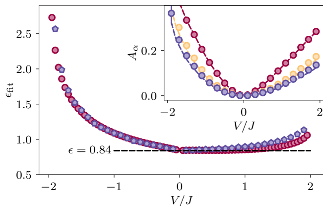
FIG. 13. Interaction dependence of the effective cutoff \varepsilon_{\text{fit}} (blue pentagons) obtained by fitting the steady state of the Luttinger liquid model at each interaction strength V/J individually to the numerical data of the von Neumann entanglement entropy. For comparison, we show again the effective cutoff obtained from the ground state case (red circles) and find very good agreement with a quasi-plateau in the region 0 < V/J < 1 . The inset depicts numerical data for Rényi entropies with \alpha = 1 (red circles), \alpha = 2 (yellow circles), and \alpha = 5 (blue circles) together with the fitted field theory steady state predictions for the effective cutoff \varepsilon_{\text{fit}} .
