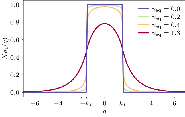
FIG. 4. Distribution function N\rho_1(q) , Eq. (39), obtained from the x/L \ll 1 limit of the one body reduced density matrix in the Luttinger liquid model for a fixed interaction cutoff \varepsilon = 0.84 and various interaction strengths V/J . Without interactions, \gamma_{\text{eq}} = 0 , the distribution function is a step function up at the Fermi momenta k_F = \pm\pi/2 .
