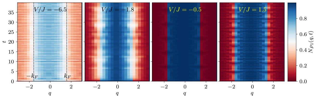
FIG. 14. Exact diagonalization results for the time evolution of distribution function N\rho_1(q, t) after a quantum quench for different values of the post quench interaction strength V/J . The initial state at t = 0 is the ground state of N = 12 non-interacting fermions hopping on a ring of L = 24 sites. The dashed vertical lines mark the Fermi momenta, around which the fluctuations are more pronounced. Increasing the interaction strength increases the amplitude of fluctuations.
