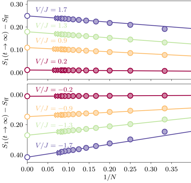
FIG. 11. Finite size scaling of the steady state one-particle von Neumann entanglement entropy S_1(t \rightarrow \infty) for various values of the post quench interaction strength V/J obtained with ED (filled circles) and with DMRG (filled crosses). We estimate the thermodynamic limit values of the entropy (empty circles) using linear extrapolation to 1/N \rightarrow 0 .
