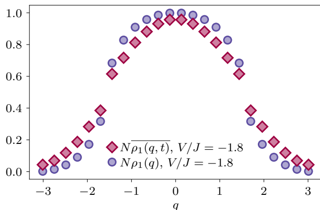
FIG. 15. Comparison between the time average of the distribution function N\rho_1(q, t) (red diamonds) after a quench to interaction strength of V/J = -1.8 and the distribution function N\rho_1(q) (blue circles) for the corresponding equilibrium case. The ED data is for a system of N = 12 fermions at half-filling.
