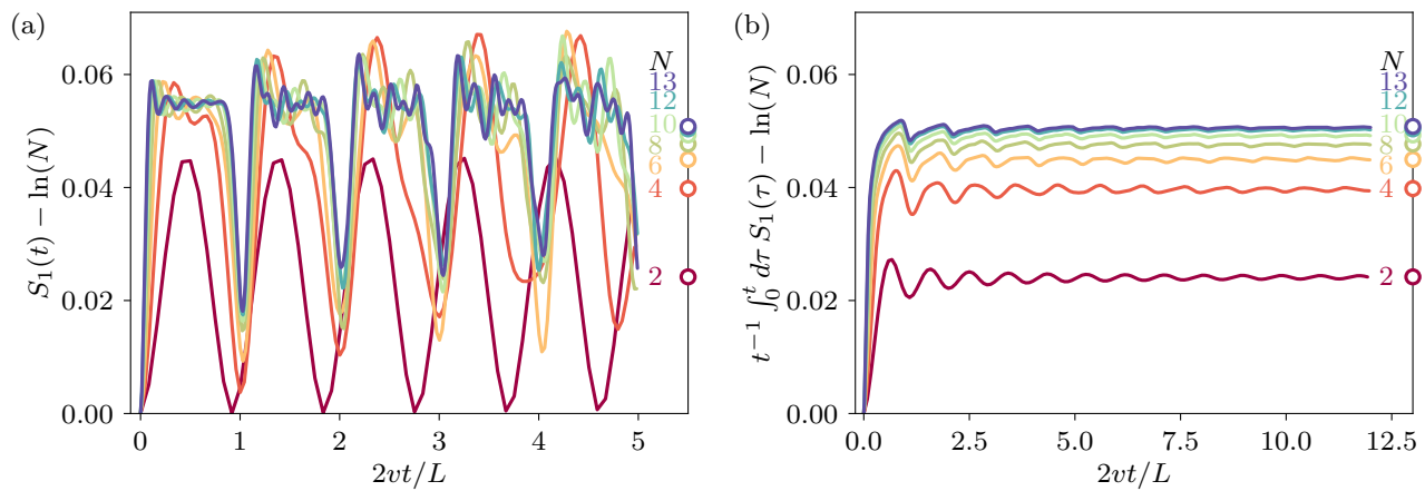
FIG. 10. Evolution of the one-particle entanglement entropy after the quantum quench at t = 0 for systems with L = 2N sites at an interaction strength of V/J = -0.5 . (a) Rescaled waiting time 2vt/L dependence of the von Neumann entanglement entropy. (b) Running average of the von Neumann entanglement entropy depicting the convergence to the steady state entropy. We observe a steep increase of the entropy on a very short time scale after the quench and then recurrences with length N where the entropies oscillate around a constant steady state value (empty circles). The fast decrease in the distance between the steady state values with N suggests fast convergence to the thermodynamic limit.
