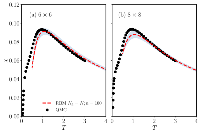
FIG. 5. Magnetic susceptibility of the 2D Heisenberg model comparing results obtained with restricted Boltzmann machines and quantum Monte Carlo for two system sizes (a) 6 \times 6 and (b) 8 \times 8 with n = 100 initial random states n and N_h = N hidden variables. The shaded area represents the error for the dashed variables.
