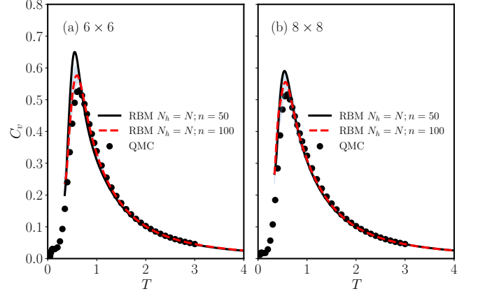
FIG. 3. Specific heat of the 2D Heisenberg model comparing results obtained with restricted Boltzmann machines and quantum Monte Carlo for two system sizes (a) 6 \times 6 and (b) 8 \times 8 with varying number of initial random states n and N_h = N hidden variables. The shaded area represents the error for the dashed curve.
