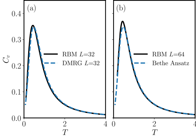
FIG. 2. Specific heat of the Heisenberg chain comparing results obtained with restricted Boltzmann machines and other methods: (a) DMRG for L = 32 , (b) L = 64 and Bethe Ansatz. We use N_h = 3N hidden variables and n = 50 random initial states.
