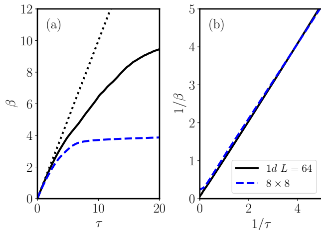
FIG. 6. (a) Actual inverse temperature \beta versus projected imaginary time \tau . We show results for both 1d and 2d lattices. The dotted line corresponds to a 1:1 perfect scaling. The differences arise from projecting on the variational manifold (see text). (b) Same data as panel (a), but showing the physical temperature T = 1/\beta .
