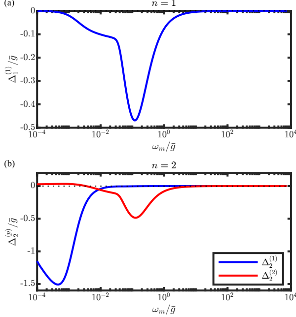
FIG. 5. Eigenfunctions corresponding to the negative eigenvalues of the kernel matrix \mathcal{K}_{\omega, \omega'} for (a) n = 1 and (b) n = 2 . We set \gamma = 0.8 .
