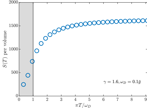
FIG. 2. Entropy per volume S(T) as a function of \pi T/\omega_D , where we take the parameters \omega_D = 0.1\bar{g} and \gamma = 1.6 . A cutoff \Lambda \sim 15\bar{g} is used to regularize the ultra-violet divergence. The grey region highlights the Fermi liquid regime where \pi T \ll \omega_D .
