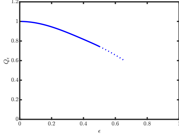
FIG. 8. The series for Q_\epsilon given by Eq. (69). The series converge for \epsilon \leq 0.5 . The dashed line is an extrapolation to somewhat larger \epsilon .
