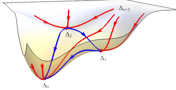
FIG. 1. A schematic plot of the free energy configuration in the functional space and the saddle points corresponding to the gap function \Delta_n(\omega_m) . The n > 0 solution is a saddle point of the free energy, which has n unstable principle axes connected with the n' < n solutions, as illustrated by the flows in the plot. The n = 0 solution is a stable minimum.
