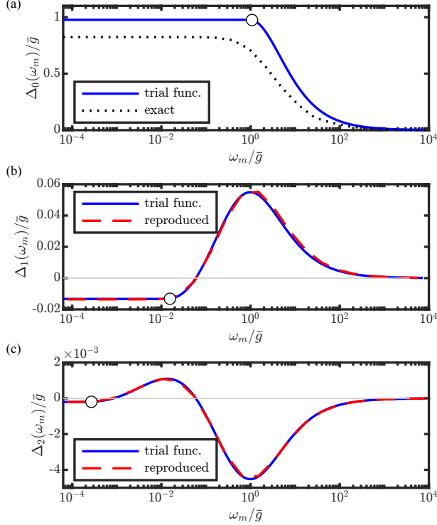
FIG. 3. Trial gap function (blue solid line) of (a) n = 0 , (b) n = 1 , and (c) n = 2 solutions, where \gamma = 0.8 . Exact gap function of n = 0 solution is shown by the black dotted line. In panels (b),(c), the reproduced gap function by substituting the trial gap function back to the gap equation is shown by red dashed lines. Circles indicate \omega_c , below which the trial gap function \Delta_n(\omega_m) becomes a constant.
