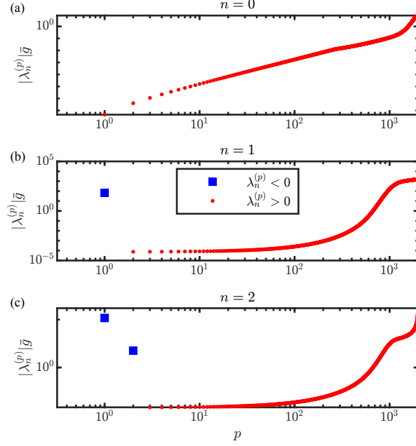
FIG. 4. Eigenvalues of the kernel matrix \mathcal{K}_{\omega, \omega'} for (a) n = 0 , (b) n = 1 , and (c) n = 2 solutions, where \gamma = 0.8 .
