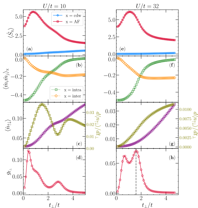
Figure 10. ED results of observables in a \sqrt{8} \times \sqrt{8} bilayer at U/t = 10 vs. interplane hybridization: (a) the expectation value of the staggered charge and spin-structure factor; (b) intra- and interplane spin-spin nearest neighbor correlations; (c) double occupancy and (d) the fidelity susceptibility. (e–h), the same for U = 32t ; vertical dashed line in (h) depicts the Heisenberg result from Ref. [2, 20] J_\perp^c/J = 2.52181(3) converted to t_\perp^c/t = 1.58802(1) via their correspondence in the strongly interacting regime, J \propto t^2/U .
