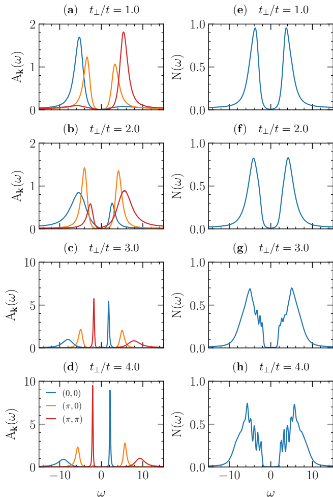
Figure 5. The spectral function A_{\mathbf{k}}(\omega) (a-d) and the single-particle density of states N(\omega) (e-h) for various interplane hoppings as marked. For values t_{\perp}/t \gtrsim 2 the gap turns indirect, connecting the two bands at (\pi, \pi) and (0, 0) , respectively. The density of states at large t_{\perp}/t 's displays a collection of features connected to the incoherent superposition of interplane singlet-states. Data is obtained for U/t = 10 , T/t = 1/20 in an L = 12 bilayer.
