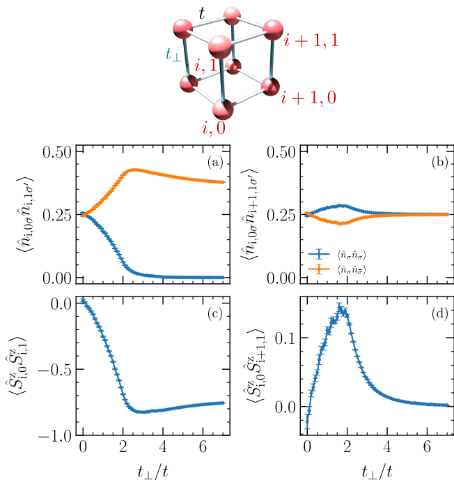
Figure 8. (Top): Cartoon depicting the different sites (i, l) where the two-point correlations are computed as displayed in the lower panels. (Bottom): The interlayer (a-b) density-density correlations for same (\sigma = \sigma') and different spin components (\sigma \neq \sigma' = -\sigma) within the same unit-cell (a) and nearest-neighbor unit cells (b). (c) and (d) display the equivalent for the spin-spin correlations. All data are extracted at U/t = 10 for L = 14 and T/t = 1/20 . Spin summation is implicitly assumed for the density correlations.
