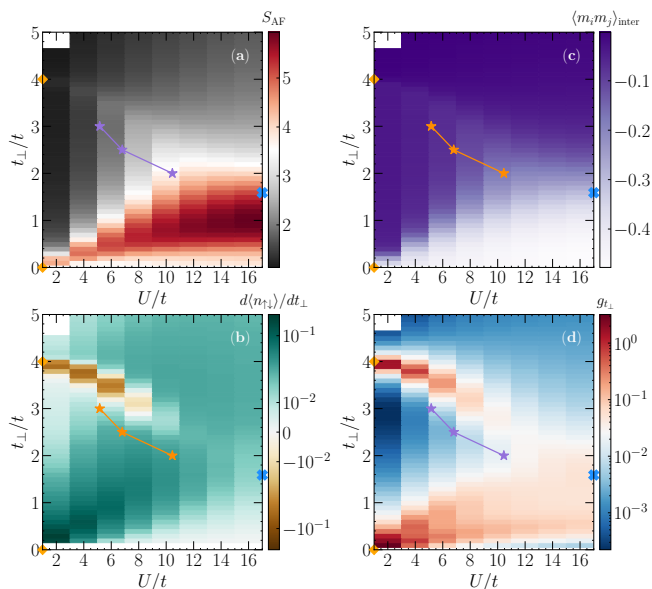
Figure 11. Color maps of several quantities in the space of parameters t_{\perp} vs. U for the 2 \times 8 -sites bilayer lattice. (a) Expectation value of the antiferromagnetic spin-structure factor, (b) derivative of the double occupancy in respect to t_{\perp} , (c) interplane spin-spin nearest neighbor correlations, and (d) the fidelity susceptibility g_{t_{\perp}} . Star markers depict the magnetic transition at T = 0 obtained using QMC in much larger lattices in Ref. [15]; cross marker on the right (large U ) panel edge denotes the Heisenberg limit [2, 20]; and diamond-shaped ones mark the nesting conditions in the noninteracting regime for this cluster size.
