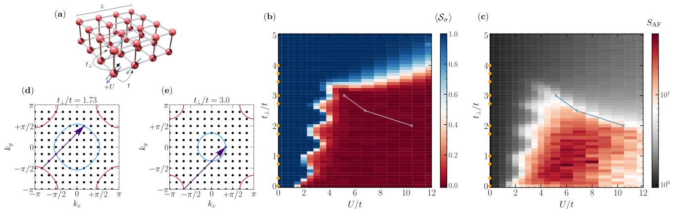
Figure 1. (a) Schematic illustration of the Hamiltonian, with relevant parameters annotated. (b) The contour plot of the average spin resolved sign \langle S_\sigma \rangle in the space of parameters (t_\perp, U) ; (c) the equivalent for the antiferromagnetic structure factor S_{AF} . All data are extracted at temperatures T/t = 1/20 in a 12 \times 12 bilayer. Markers along the U/t = 0 axis in (b) and (c) depict the values of t_\perp/t that result in a nesting condition with a wavevector (\pi, \pi) for this lattice size. Examples of such nestings are shown in (d) and (e) for t_\perp/t = 1.73 and 3.0 , respectively. Lines in (b) and (c) depict the results of Ref. 15 marking the magnetic transition obtained via the scaling of the antiferromagnetic order parameter at T = 0 .
