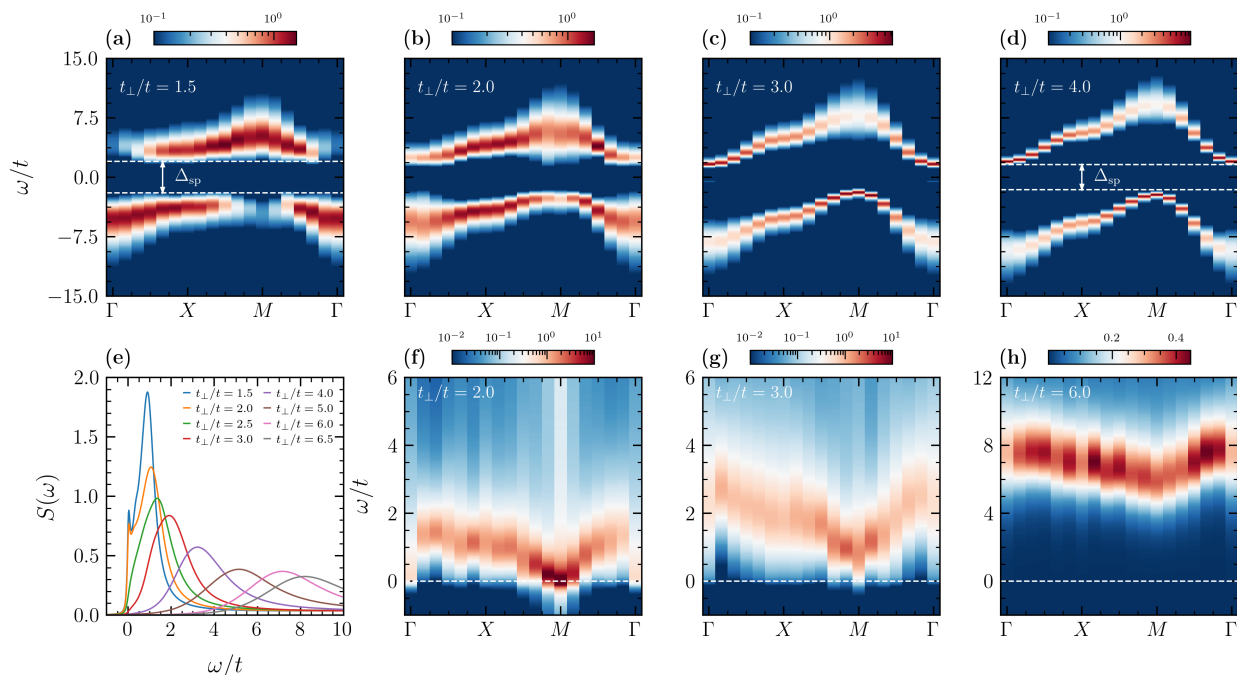
Figure 2. (a–d) The single-particle excitation spectrum A_{\mathbf{k}}(\omega) across a path connecting high-symmetry points ( \Gamma - X - M - \Gamma ) in the Brillouin zone, for the indicated hybridization amplitudes. In (a), t_{\perp}/t = 1.5 , and (d), t_{\perp}/t = 4.0 , the single-particle gap \Delta_{\text{sp}} is marked, exhibiting, respectively, a direct and indirect behavior. (f–h) dynamical spin structure factor S(\mathbf{k}, \omega) at different t_{\perp}/t as marked, with a momentum integrated version shown in (e). Data are obtained at temperatures T/t = 1/20 in an L = 12 bilayer with U/t = 10 .
