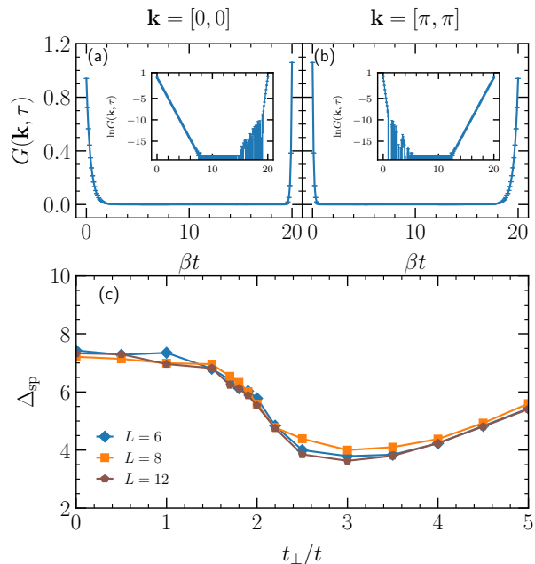
Figure 6. (a-b) The imaginary-time ( \tau ) dependent Green's function G(\mathbf{k}, \tau) at U/t = 10 , t_{\perp}/t = 4.5 for L = 12 . Inset: G(\mathbf{k}, \tau) on semi-logarithmic scales. (c) The single-particle gap \Delta_{\text{sp}} extracted by the minimum gap of fitting \ln G(\mathbf{k}, \tau) \sim \pm \omega_{\mp}(\mathbf{k})\tau across the whole Brillouin zone (see text).
