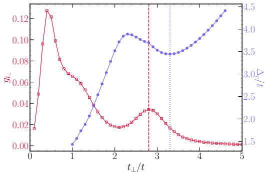
Figure 12. The charge gap \Delta_c (right-axis) vs. interplane hybridization for a \sqrt{8} \times \sqrt{8} bilayer, computed via ED with U/t = 10 . For comparison, we also show the fidelity susceptibility (left-axis) at the same interaction strength. The local minimum (maximum) of \Delta_c ( g_{\perp} ) is marked via a dotted (dashed) vertical line at t_{\perp}/t = 3.3 ( t_{\perp}/t = 2.8 ).
