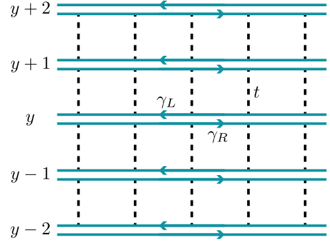
FIG. 7. Pattern of interchain emergent-fermion tunnelings encoded in the second line of Eq. (53). The left-mover originating from chain y couples to the right-mover from chain y + 1 , gapping the interior but leaving unpaired chiral Majorana edge modes at the top and bottom chains. In the 2D Rydberg setup, the resulting phase is a non-Abelian spin liquid with Ising topological order.
