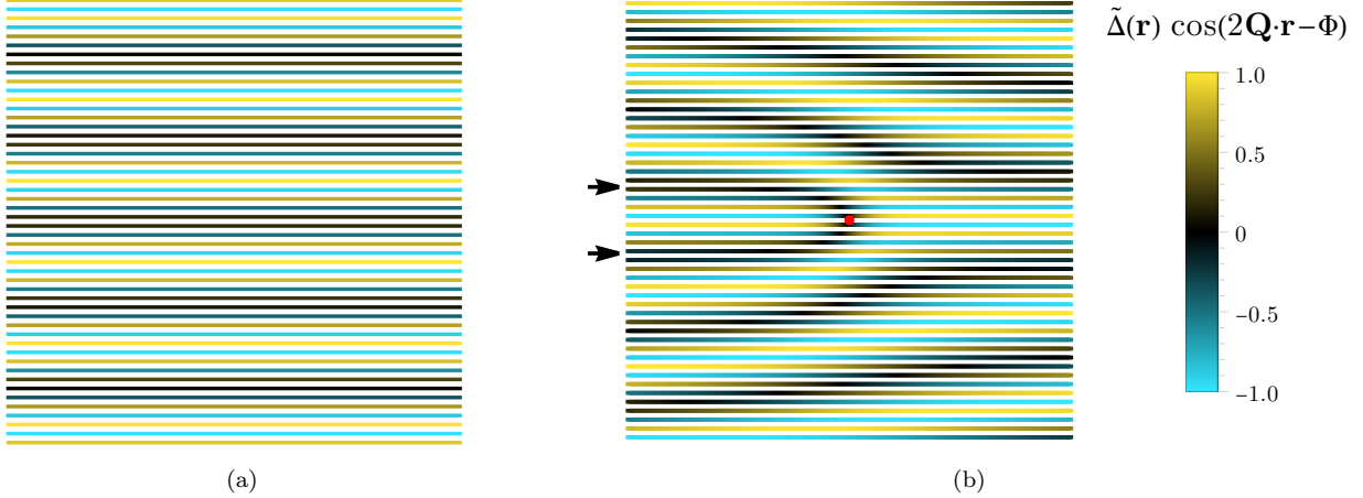
FIG. 5. (a) Spatially modulated detuning pattern that generates toric-code topological order by explicitly breaking inter-chain translation symmetry \mathbb{T}_y . (b) Modified detuning pattern that yields a non-Abelian defect (centered at the red dot) in the toric-code phase. The color represents the detuning shift \tilde{\Delta}(\mathbf{r}) \cos[2\mathbf{Q}\cdot\mathbf{r} - \Phi(\mathbf{r})] from Eq. (50) with \mathbf{Q} = (0, 1.4) in both panels. In (a), we use uniform \tilde{\Delta}(\mathbf{r}) and \Phi(\mathbf{r}) . In (b), we instead take \Phi(\mathbf{r}) to wind by 2\pi around the red dot and set \tilde{\Delta}(\mathbf{r}) \propto \tanh(r/\xi) (with \xi^{-1} \approx 1/3 ) to introduce a vortex core. The colorbar is normalized such that \pm 1 correspond to the maximum and minimum values of the detuning shift—which should reflect small perturbations to the microscopic Hamiltonian.
