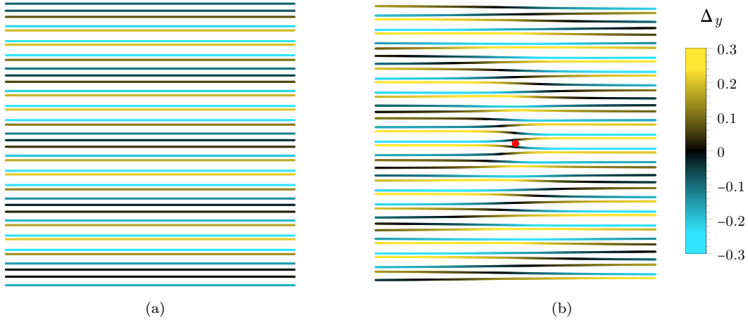
FIG. 6. Variation of Fig. 5 that accesses toric-code topological order by breaking inter-chain translation symmetry \mathbb{T}_y via small shifts in the Rydberg-chain positions [leading to Eq. (51)]. Panel (a) realizes the defect-free toric code, while panel (b) hosts a non-Abelian defect centered at the red circle. Chains are colored according to their displacement \Delta_y away from their original positions (exaggerated for clarity and in units of interchain spacing). The positions were calculated by assuming \Delta_{y+1} - \Delta_y \propto -A(\mathbf{r}) \cos[2\mathbf{Q}\cdot\mathbf{r} - \Phi(\mathbf{r})] with \mathbf{Q} = (0, 1.4) as in Fig. 5. In (a) both A(\mathbf{r}) and \Phi(\mathbf{r}) are uniform, while in (b) \Phi(\mathbf{r}) winds by 2\pi around the red circle and A(\mathbf{r}) = \tanh(r/\xi) with \xi^{-1} \approx 1/3 .
