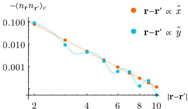
FIG. 4. Power-law behavior of the connected correlation function \langle n_{\mathbf{r}} n_{\mathbf{r}'} \rangle_c predicted for the gapless \mathbb{Z}_2 spin liquid [Eq. (46)]. Data were obtained with non-universal example parameters \vartheta = 0 , v_x = v_y = 1 , C_0 = -1 , C_{2\mathbf{Q}} = -0.5 , and \mathbf{Q} = (0, 1.4) (though the vanishing of Q_x is generic provided R_x and R_y reflection symmetries are preserved). The orange curve corresponds to separations \mathbf{r} - \mathbf{r}' along a chain, while the blue curve corresponds to separations perpendicular to the chains; additional oscillations in the latter reflect power-law correlations at momentum 2\mathbf{Q} .
