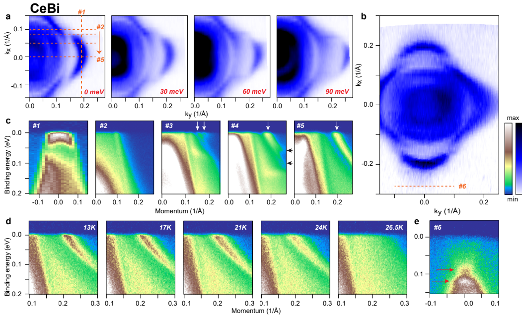
FIG. 3. Dispersion of the surface states in CeBi in the first magnetically ordered state (AFM1) at T=13.5 K. a , Constant energy plots at binding energies from 0 to 90 meV. b , Fermi surface map for a domain with different orientation of magnetic ordering. c , Band dispersion along the directions marked with the dashed lines in a . Here, white arrows indicate the location of the surface state dispersions. d , Temperature dependence of the band dispersion along cut #5 in a . e , Band dispersion along the directions marked with the dashed line in b .
