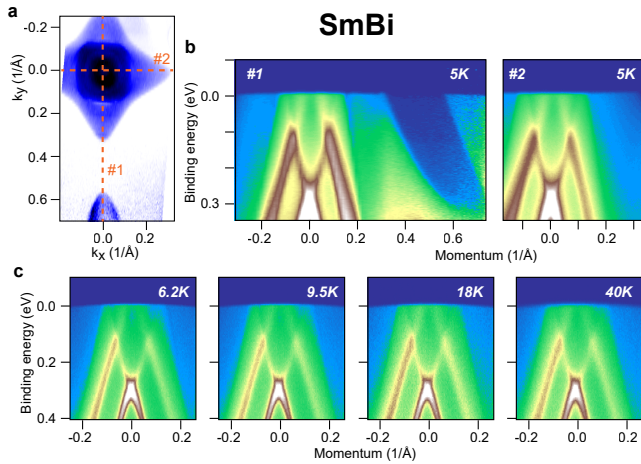
FIG. 8. Additional data from SmBi. a Fermi surface of SmBi in the AFM state (the same as Fig.1f). b Band dispersions along the directions marked with the dashed line in (a). c Temperature dependence of the band dispersions along \Gamma - X direction.
