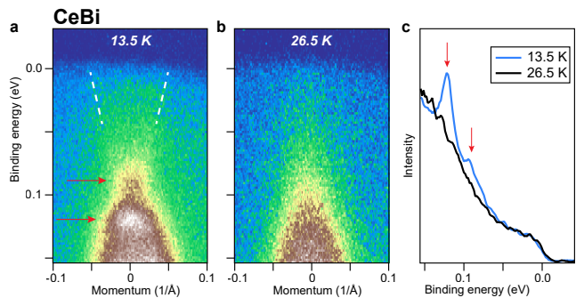
FIG. 7. Band dispersion below and above T_N in CeBi. a Spectrum measured in the AFM state (the same as Fig.3e). b The same spectrum as in (a) but measured in the PM state. c EDCs taken through the band center from (a) and (b)
