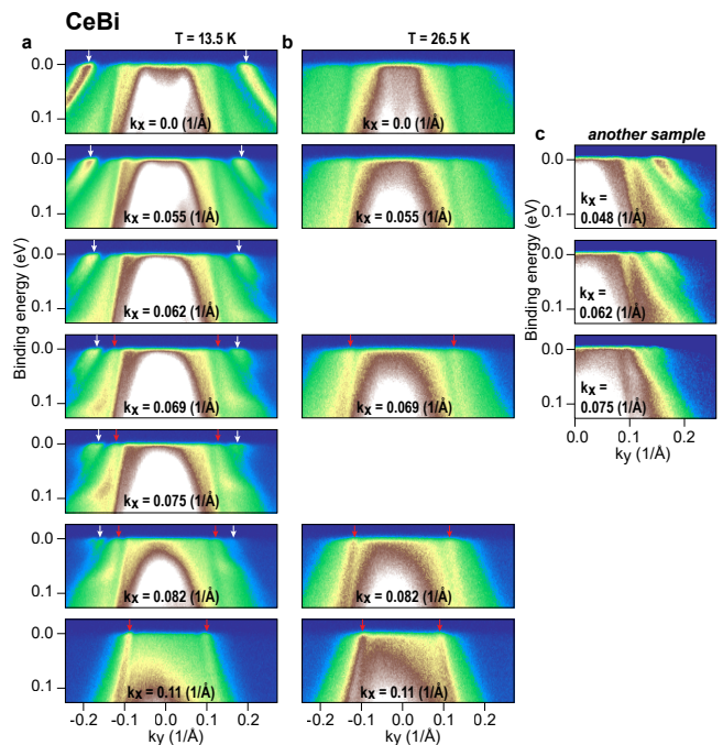
FIG. 6. Band dispersion in the AFM and PM states of CeBi. a Band dispersions along several cuts parallel \Gamma - X direction measured in the AFM state. Here, white and red arrows indicate the location of the surface state and bulk dispersions, respectively. b The same band dispersions as in (a) but measured in the PM state. c Band dispersions measured in the AFM state from another sample.
