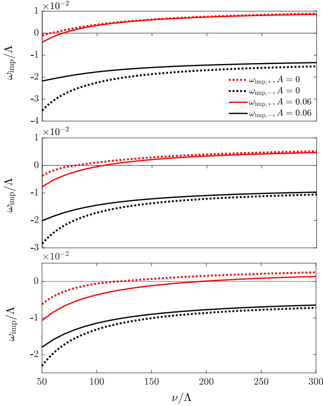
FIG. 3. Exact numerical result for the impurity energy E_{\text{imp}} for graphene in equilibrium \mathcal{A} = 0 and irradiated with light \mathcal{A} = 0.06 in the AB Armchair case as a function of the effective potential \nu . The upper, middle and lower panels correspond to impurity distances R = 31a, 43a, 64a respectively.
