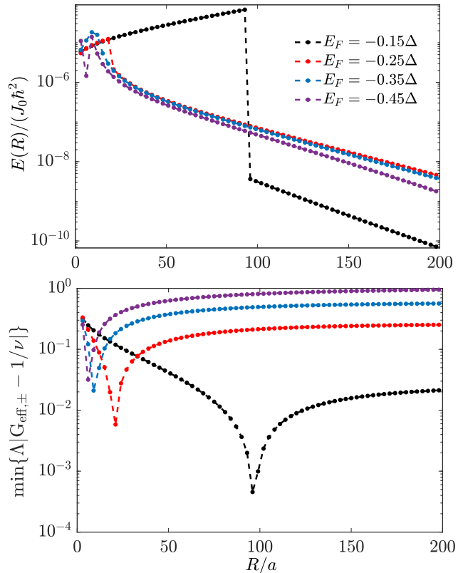
FIG. 7. The upper panel shows the time-averaged exchange energy E/(J_0\hbar^2) versus impurity separation R/a for impurities situated at sublattices AA and along the armchair direction with negative Fermi energy. The driving field strength is \mathcal{A} = 0.06 . The lower panel plots the magnitude of the difference G_{\text{eff},\pm} - 1/\nu , with its minimum giving the position of the resonance feature in the exchange energy.
