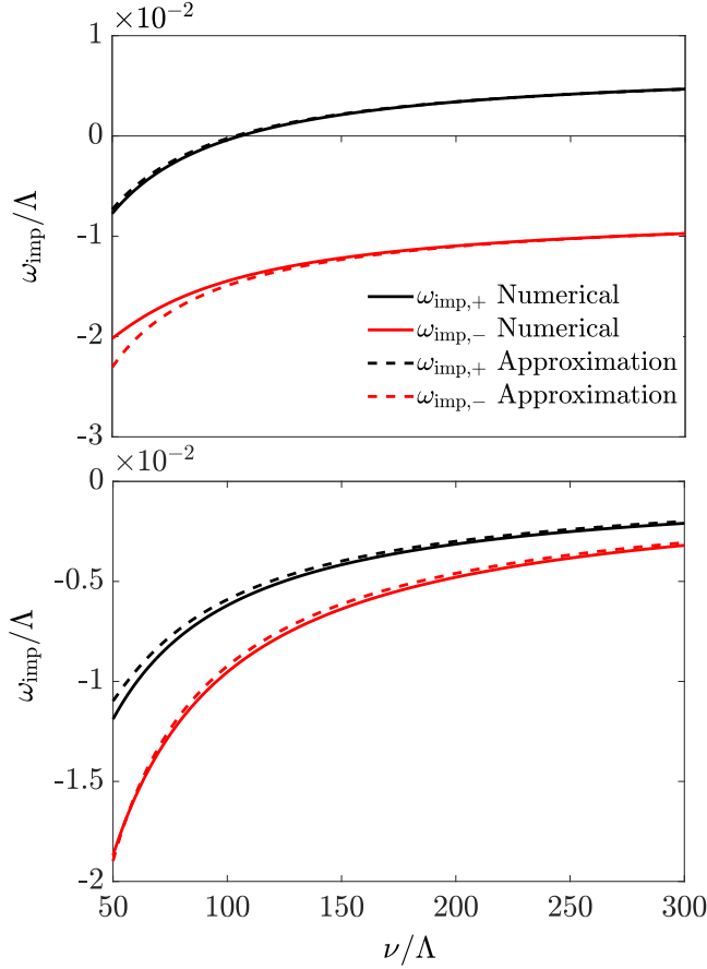
FIG. 4. Comparison of the exact numerical result and analytical approximation for the impurity energy \omega_{\text{imp}} for graphene irradiated with light \mathcal{A} = 0.06 as a function of the effective potential \nu . The upper and lower panels correspond to the AB armchair case with R = 43a and AA armchair case with R = 39a .
