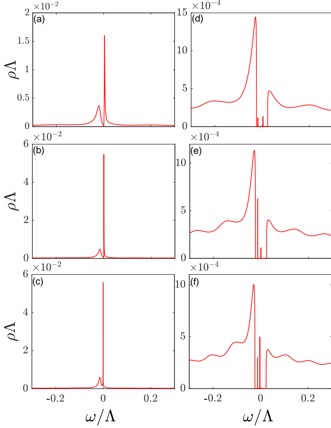
FIG. 1. Time-averaged local density of states of graphene evaluated at the impurity sublattice site A in equilibrium [panels (a)-(c)] and under irradiation with \mathcal{A} = 0.06 [panels (d)-(f)]. The impurities are located at A and B separated along the armchair direction with u = 100\Lambda . The upper two, middle two and lower two panels correspond to the values of impurity separation R = 31a, 43a, 55a , respectively.
