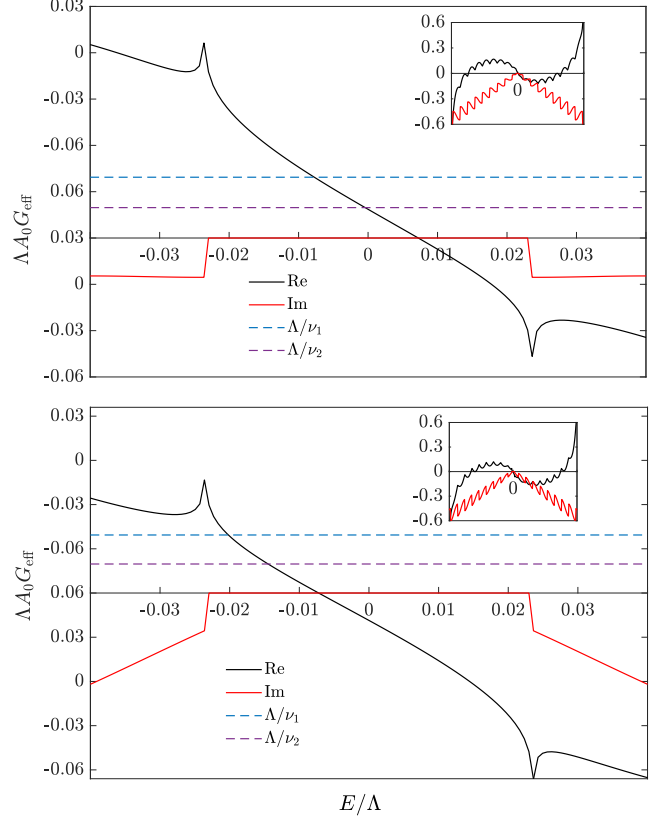
FIG. 2. Real and imaginary parts of the effective Green's function G_{\text{eff},+} (upper panel) and G_{\text{eff},-} (lower panel) for irradiated graphene with \mathcal{A} = 0.06 in the AB armchair case. The impurity separation is R = 43a and effective potentials are \nu_1 = 50\Lambda , \nu_2 = 100\Lambda .
