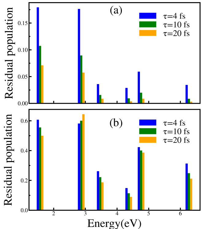
FIG. 5. Residual population of conduction band levels. The pulse amplitude is 0.5 V/Å. The corresponding dephasing times are marked in each panel. The frequency of the pulse is \hbar\omega_0 = 1 eV (a) and \hbar\omega_0 = 2 eV (b).
