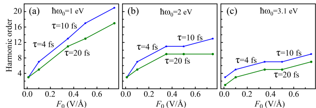
FIG. 9. Harmonic cutoff versus the amplitude of the optical pulse. The frequency of the pulse is \hbar\omega_0 = 1 eV (a), 2 eV (b), and 3.1 eV (c). The relaxation time is shown next to the corresponding line in each panel. The first data point in all panels correspond to the field amplitude of 0.01 V/Å.
