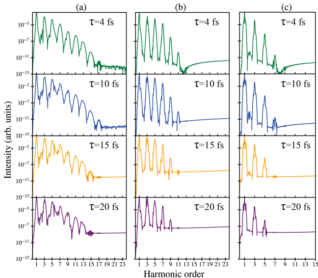
FIG. 6. Emission spectrum of graphene QD. High harmonics with well-defined cutoffs are clearly visible in the spectrum. The corresponding relaxation times are marked for each graph. The frequency of the pulse is \hbar\omega_0 = 1 eV in column (a), \hbar\omega_0 = 2 eV in column (b), and \hbar\omega_0 = 3.1 eV in column (c). With increasing the relaxation time, the emission spectrum becomes more noisy with less defined high harmonic peaks. The pulse amplitude is F_0 = 0.4 V/Å.
