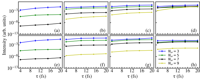
FIG. 8. Intensity of the first four high harmonics ( N_\omega = 3, 5, 7, and 9 ) versus the relaxation time. The frequency of the pulse is \hbar\omega_0 = 1 eV in panels (a)-(d) and 2 eV in panels (e)-(h). The pulse amplitude is 0.1 V/Å (a) & (e), 0.35 V/Å (b) & (f), 0.5 V/Å (c) & (g), and 0.75 V/Å (d) & (h).
