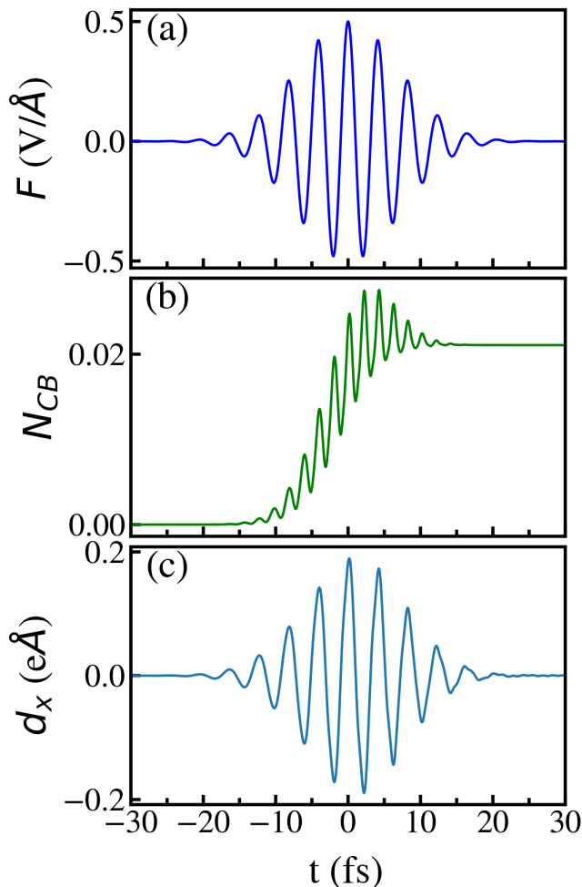
FIG. 3. Panel (a): profile of a linearly polarized pulse. The pulse amplitude is 0.5 V/Å and the frequency of the pulse is \hbar\omega_0 = 1 eV. Panel (b): conduction band population N_{CB} as a function of time. The QD is in the field of the pulse shown in panel (a). The conduction band population is normalized by the number of electrons, i.e., it is divided by 12. The corresponding dipole moment is shown in panel (c). Only x component of the dipole moment is nonzero. The dipole moment roughly follows the profile of the electric field shown in panel (a).
