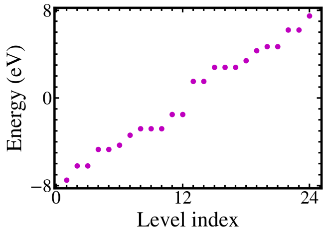
FIG. 2. Energy spectrum of graphene QD shown in Fig. 1. The spectrum consists of singly, doubly, and triply degenerate levels. Levels with the negative energy correspond to the valence band while the levels with the positive energy correspond to the conduction band. Before the pulse, all valence band levels are occupied.
