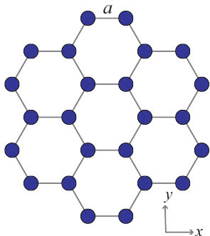
FIG. 1. Graphene quantum dot consisting of 24 carbon atom. The incident laser pulse is linearly polarized along the x -direction. The distance between the nearest neighbor atoms is a = 1.42\text{\AA} .
