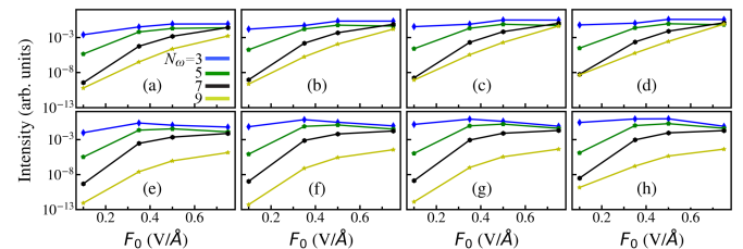
FIG. 7. Intensity of the first four high harmonics ( N_\omega = 3, 5, 7 , and 9) versus the amplitude of the optical pulse, F_0 . The frequency of the pulse is \hbar\omega_0 = 1 eV in panels (a)-(d) and 2 eV in panels (e)-(h). The relaxation time is 4 fs (a) & (e), 10 fs (b) & (f), 15 fs (c) & (g), and 20 fs (d) & (h).
