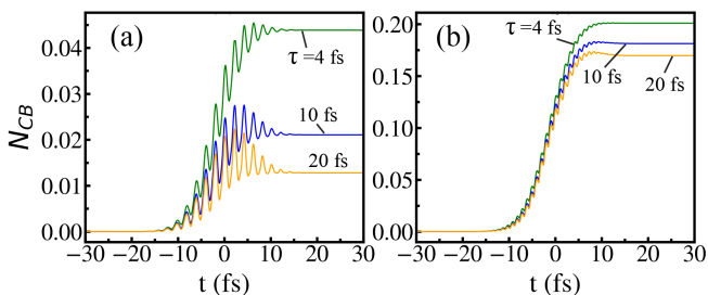
FIG. 4. Conduction band population as a function of time. The conduction band population is normalized by the number of electrons, i.e., it is divided by 12. The corresponding relaxation times are shown next to the lines. The frequency of the pulse is \hbar\omega_0 = 1 eV (a) and \hbar\omega_0 = 2 eV (b). The pulse amplitude is 0.5 V/Å.
