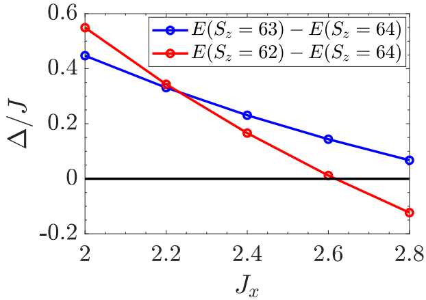
Figure 8. Excitation energy \Delta for S_z = 63 and S_z = 62 excitations from the ferromagnetic state S_z = 64 for J_z = -1 and J_x > 0 . The results are essentially size independent and were checked up to 128-site periodic cluster.
