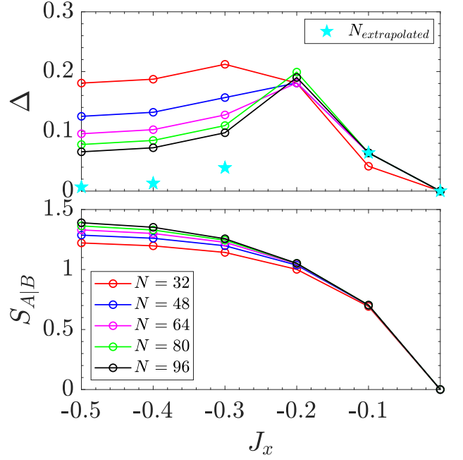
Figure 5. Energy gap \Delta and entanglement entropy S_{A|B} vs. J_x for J_z = 1 and J_x < 0 . In the power-law XY FM phase |J_x| > 0.2 , the extrapolated energy gap closes and the entanglement entropy grows logarithmically with size. The energy gap is finite and nearly size independent in the spin-liquid phase.
