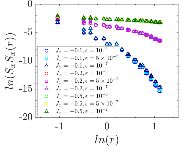
Figure S3. The logarithm of spin-spin correlation \ln(S_x S_x(r)) vs. the logarithm of sites distance \ln(r) on a 96-sites pyrochlore lattice. J_z = 1 and the value of J_x is shown in the legend. Different truncation error cutoff \epsilon curves are on top of each other, indicating \epsilon = 10^{-6} we use in the main text is small enough to capture the physics.
