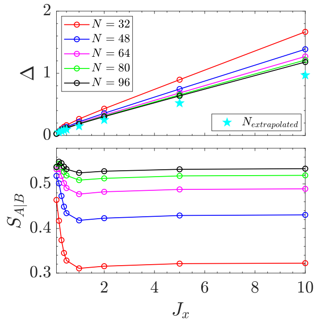
Figure 7. Energy gap \Delta and entanglement entropy S_{A|B} v.s. J_x for J_x > 0 and J_z = 1 . A robust energy gap is observed for all J_x values and entanglement entropy saturates ultimately when lattice size increases.
