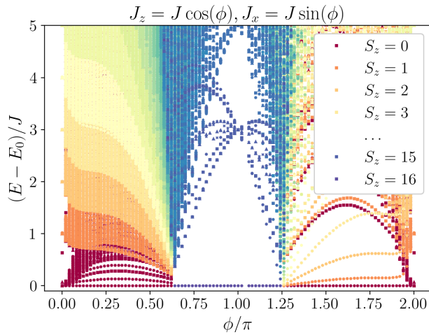
Figure 3. Low-lying spectrum of an L = 2 periodic cluster with 32 spins obtained by Exact Diagonalization (ED). The states are characterized by their S_z quantum numbers. Three classes of ground-state regimes are evident from the figure. A high- S_z ground-state phase in the middle, which corresponds to an Ising ferromagnet ( 0.63\pi \lesssim \phi \lesssim 1.25\pi ), and two S_z = 0 ground-state regimes on the sides ending at the highly degenerate spin ice states at \phi = 0 or 2\pi . Energy levels at S_z = \pm k are degenerate due to spin flip symmetry.
