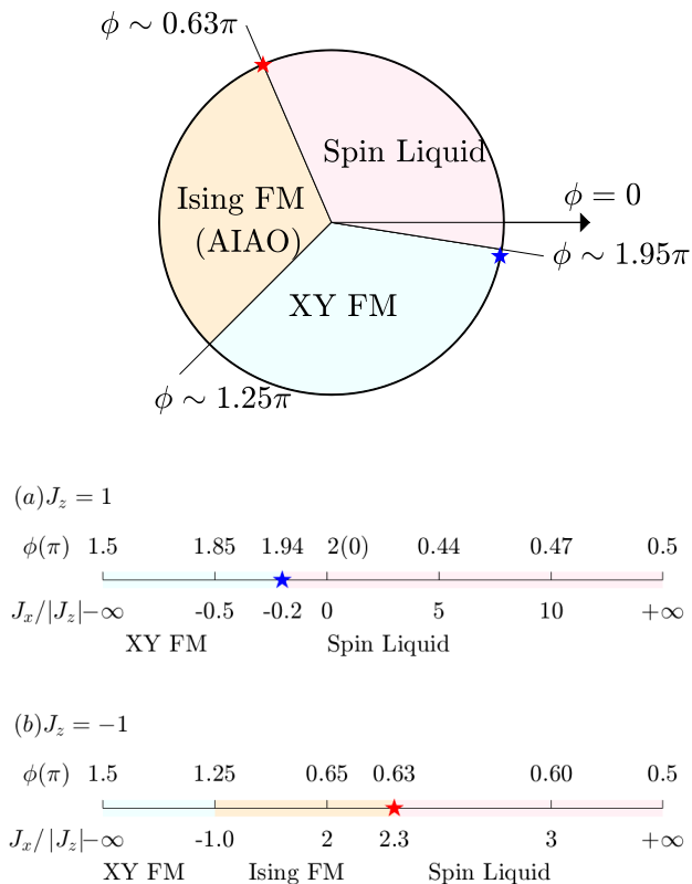
Figure 2. The upper panel shows the three primary ground state regimes of the model as a function of \phi defined by the relations J_z = J \cos \phi , J_x = J \sin \phi : (i) Ising ferromagnet (FM) also called all-in-all-out (AIAO) phase (see text), (ii) XY ferromagnet and (iii) spin liquid. The nature of the spin liquid phase and whether there are multiple phases within the spin liquid region is a primary focus of our study. The lower panels show the phases with |J_z| = 1 . The phase transition points are inferred from the spectra of the 32-site cluster with periodic boundary conditions obtained by Exact Diagonalization (ED) as well as from a DMRG or ED calculation on a 96-site or 128-site cluster discussed in Sec. 4
