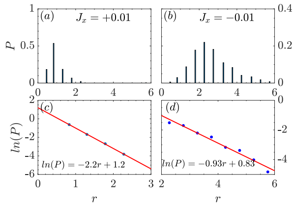
Figure 10. (a)(b)Probability of monopole-antimonopole pair separations P v.s. pair separations r (c)(d)logarithm of the probability \ln(P) v.s. separation r
