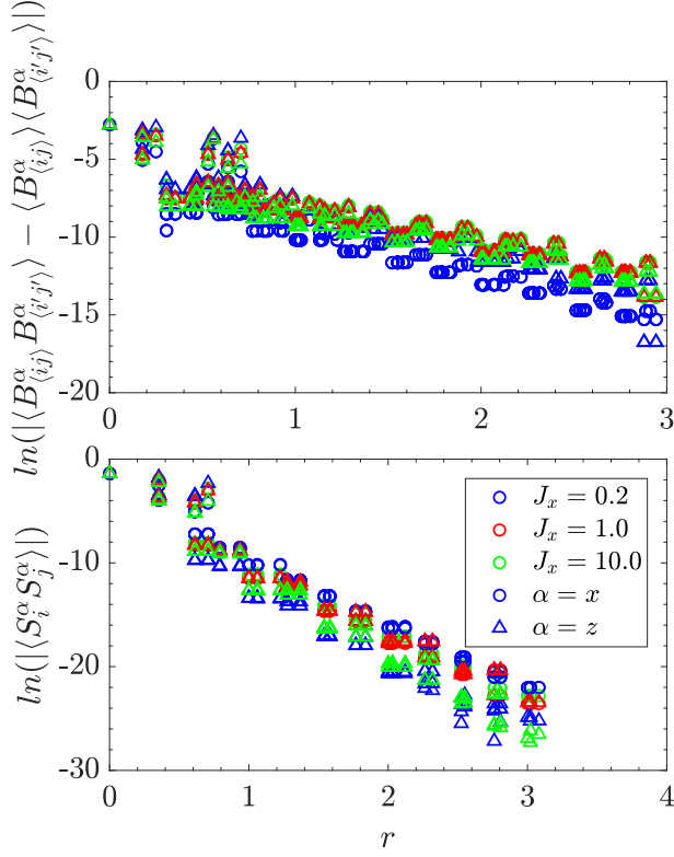
Figure S4. Exponential decay of spin-spin and bond-bond correlations on a 96-site pyrochlore lattice with J_z = 1 , J_x > 0 . \alpha is the spin index. Spin x and z are symbolized by circles and triangles respectively. J_x = 0.2, 1.0, 10.0 data are represented by different colors.
