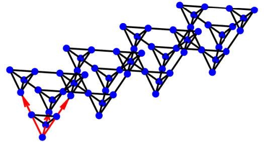
Figure 1. A pyrochlore tube lattice with length L = 4 (cubic unit cells) in the long direction. There are four tetrahedra in each cube and the total number of sites N = 4 \times 4 \times L = 64 . The side length of the cube is set to be 1 and hence the distance between the nearest neighbour sites of the pyrochlore lattice is \sqrt{2}/4 . Primitive translational vectors for the 3D pyrochlore lattice (0, 1/2, 1/2) , (1/2, 0, 1/2) and (1/2, 1/2, 0) are represented by red arrows in the figure.
