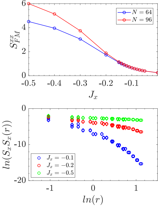
Figure 4. Upper: Ferromagnetic structure factor in the x -component as a function of coupling strength J_x for N = 64 and N = 96 systems for J_z = 1 and J_x < 0 . Lower: the logarithm of spin-spin correlations as a function of the logarithm of site distance. A linear relationship for J_x = -0.2 and J_x = -0.5 indicates a power law decay of spin-spin correlations. N = 96 and N = 64 data are represented by circle and diamond symbols respectively.
