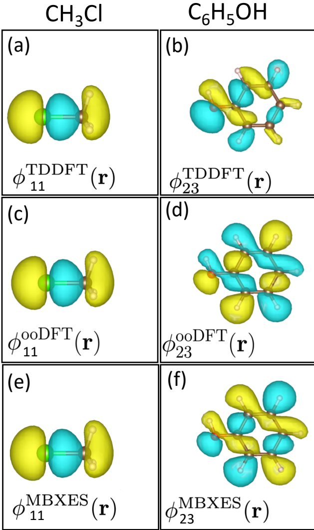
FIG. 4. Panel (a), (c) and (e) display the auxiliary orbital, evaluated using respectively LR-TDDFT, ooDFT and MBXES associated with the 11-th de-excitation in the Cl K -edge of CH 3 Cl. Panels (b), (d) and (f) plot the same for the 23-rd de-excitation in the O K -edge of C 6 H 5 OH. These plots demonstrate that MBXES effectively approximates ooDFT while, for phenol, LR-TDDFT exhibits errors associated with the adiabatic approximation.
