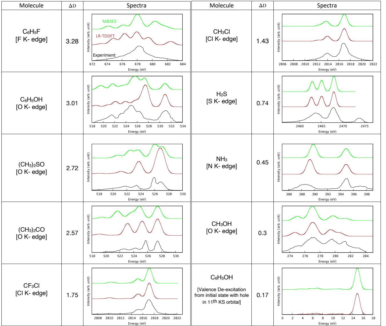
FIG. 2. Table showing experimental 32,33,45–48 (black) adiabatic LR-TDDFT (brown) and MBXES (green) spectra of different molecules. The second column shows the change in the electrostatic dipole moment, in Debye units, of the remaining electrons following the relevant core-ionization.
