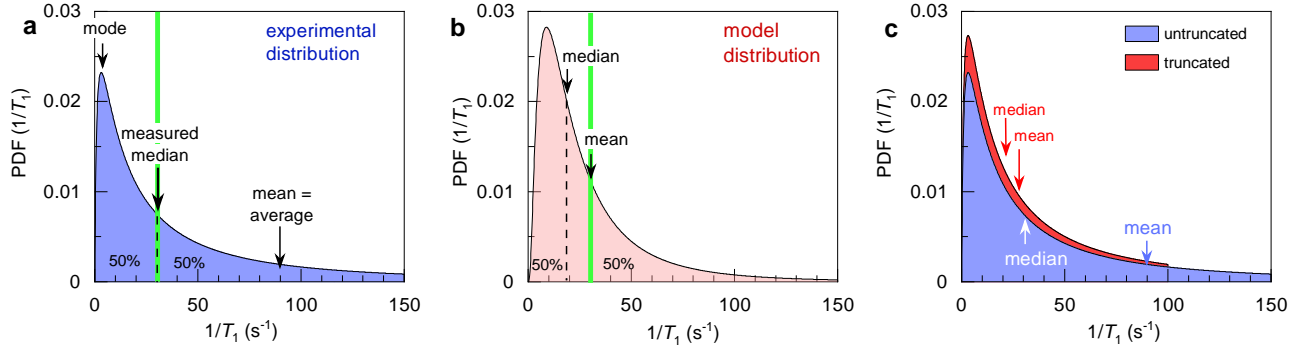
FIG. 15: Situation where the model distribution of relaxation rates (panel b) has a smaller asymmetry than the experimental distribution (panel a) such that \frac{1}{T_1}_{\text{mean, model}}(T) = \frac{1}{T_1}_{\text{median, experimental}}(T) (thick vertical line). The model distribution is "wrong" since its median relaxation rate differs from the experimental median. (c) Regular (untruncated) and truncated log-normal probability distribution functions of the relaxation rate \frac{1}{T_1} . The regular log-normal distribution has a median value of 30 \text{ s}^{-1} and a much larger mean. For the truncated distribution ( 1/T_1(\text{max}) = 100 \text{ s}^{-1} ) the mean decreases strongly, so one finds \text{median}_{\text{trunc}} \sim \text{mean}_{\text{trunc}} . After truncation the distribution is normalized again, so the integrated area is conserved.
