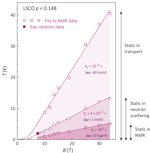
FIG. 8: Regions of the field B – T phase diagram where spin fluctuations are frozen at the timescale of transport ( 10^{-13} s), neutron scattering ( 4 \times 10^{-12} s) and NMR ( 10^{-8} s) measurements (the corresponding frequency values \omega = \tau_c^{-1} are also indicated). The open symbols correspond to the intersections between experimental \tau_c values determined from BPP fits and the horizontal grey bars in Fig. 5a (see the symbol correspondence). Solid lines are linear fits to the data. Filled point: experimental onset (7.5 T at 2 K) of quasi-elastic intensity in neutron scattering [46], that nicely matches the low-field extrapolation of the estimate based on NMR fits. Linear extrapolation of the upper line ( \tau_c = 10^{-13} s) up to 55 T yields a temperature of 70 K, approximately matching the onset of the resistivity upturn at this field [67]. Magenta and black dashes represent linear and nonlinear extrapolation of the data at low fields, with and without an onset field.
