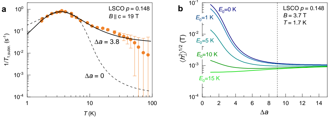
FIG. 14: (a) Relaxation rate after background subtraction fitted by T_{1,\text{BPP dist.}}^{-1}(T) without distribution of a = \ln \tau_{\infty} (dashed line) and with \Delta a = 3.8 (where \tau_{\infty} is in \text{s}^{-1} , black line). Notice that the distribution of a is assumed to be uncorrelated from that of E_0 (see Eq. 7). (b) Simulated \Delta a dependence of \langle h_{\perp}^2 \rangle^{1/2} based on Eq. 7 for an experimentally determined value T_1^{-1} = 0.018 \text{ s}^{-1} at T = 1.7 \text{ K} and B = 3.7 \text{ T} . For small \Delta a , E_0 affects \langle h_{\perp}^2 \rangle strongly but above \Delta a \sim 9 , the \langle h_{\perp}^2 \rangle value is essentially independent of E_0 . This allows to determine \langle h_{\perp}^2 \rangle from a single T_1^{-1} value at low T .
