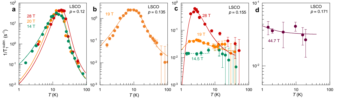
FIG. 13: T_1^{-1} data (symbols) from which a superconducting background has been subtracted as described in ref. [5] for different doping levels and the corresponding fits (continuous lines) with the distributed BPP model described in the text.
