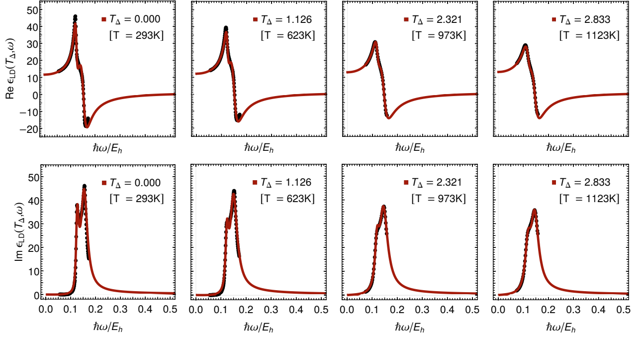
FIG. 3. We present the analog of Fig. 1 for the LD as opposed to the CM fitting procedure. Again, real (top row) and Imaginary (bottom row) parts of the dielectric function \epsilon_{LD}(T_{\Delta}, \omega) are plotted as functions of frequency \omega , for monocrystalline silicon for various temperatures, but here, for the LD fitting procedure. Experimental data 13,23 (dotted) are found to be in agreement with the LD fit (red) defined in Eq. (5) for temperature-dependent parameters given in Eq. (15) and coefficients in Table VI. For the LD fit, eight additional temperatures, between T_{\Delta} = 0 and T_{\Delta} = 2.83 , namely, the values T_{\Delta} = 0.273, 0.444, 0.614, 0.785, 1.126, 1.297, 1.468, and 1.638 , are considered in the Supplementary Material 45 .
