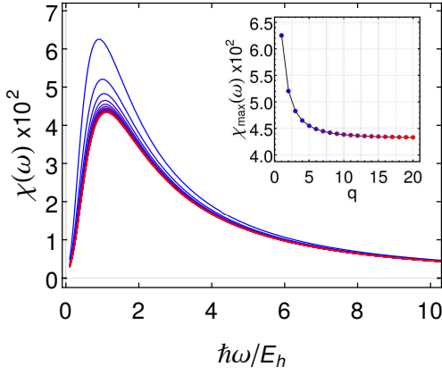
FIG. 8. The relative difference \chi(\omega) , described in Eq. (B13), between the exact expression for the dynamic polarizability of hydrogen given in Eq. (B8) and the discrete model given in Eq. (B2), is plotted as a function of the driving frequency. Here q is the number of discrete oscillator strengths included in the discrete model, as given in Table IX.
