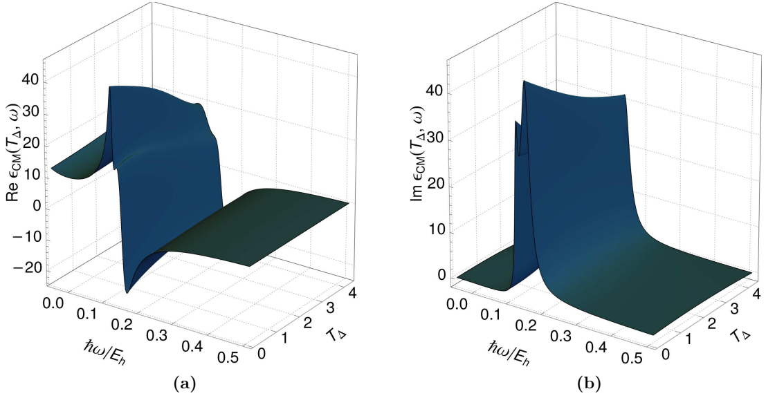
FIG. 2. Real [panel (a)] and Imaginary [panel (b)] parts of the Clausius-Mossotti dielectric function \epsilon_{\text{CM}}(T_{\Delta}, \omega) as described by Eq. (4) are plotted as functions of the reduced temperature T_{\Delta} and driving frequency \omega , for monocrystalline silicon with parameters given in Eq. (11) and coefficients in Table III. This plot shows agreement between the CM fit shown here and the LD fit shown in Fig. 4.
