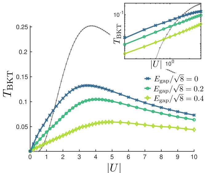
FIG. 1. BKT temperature computed for the square lattice (gray) and for the Lieb lattice with a half-filled flat band (blue, green and yellow) with different values of the hopping staggering (see Fig. 2). Inset: BKT temperature at interactions 0.2 \leq |U| \leq 3 . The flat band is isolated from the other bands by a band gap E_{\text{gap}} = \sqrt{8}\eta . The highest BKT temperatures are obtained when \eta = 0 , which corresponds to the situation where the gap between the flat band and dispersive bands closes, resulting in a linear band touching. The BKT temperature for the square lattice (gray) is exponentially suppressed at low interactions, whereas T_{BKT} on the isolated flat band is proportional to |U| . All energies are given in units of the average inter-lattice-site hopping energy t .
