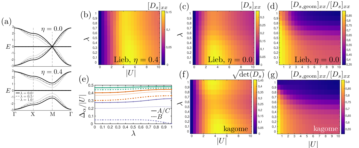
FIG. 5. (a) Band structure of the tunable Lieb model for different values of \lambda , at \eta = 0 , i.e. in the presence of a band touching, and at \eta = 0.4 . The band touching can be tuned from linear ( \lambda = 0 ) to quadratic ( \lambda = 1 ) at \eta = 0 . At \eta = 0.4 , the dispersive bands are modified without changing the quantum metric of the flat band. (b) Superfluid weight [D_s]_{xx} for \eta = 0.4 in the Lieb model, when the flat band is separated from the other bands by a gap. At low |U| , D_s is independent of \lambda , but at intermediate |U| , the limit \lambda = 0 , corresponding to a linear touching, has a more pronounced maximum. (c) Superfluid weight [D_s]_{xx} and (d) ratio [D_{s,\text{geom}}]_{xx}/[D_s]_{xx} in the tunable Lieb lattice. The off-diagonal components of the superfluid weight are zero. The superfluid weight is largest in the linear model. (e) Order parameters \Delta_\alpha/U in the tunable Lieb lattice as a function of \lambda at interaction strengths U = -1 (blue), U = -4 (orange) and U = -8 (green). The order parameters in the A/C orbital (full line) are always equal, and are larger than the order parameter in the B orbital (dashed line). The dotted line shows the average of all order parameters. (f) \sqrt{\det(D_s)} and (g) [D_{s,\text{geom}}]_{xx}/[D_s]_{xx} in the tunable kagome model. In this case, the off-diagonal components are not always zero. A similar behavior of the ratio [D_{s,\text{geom}}]_{ij}/[D_s]_{ij} is observed for all components. The maximum of \sqrt{\det(D_s)} is slightly more pronounced in the linear model, but the superfluid weight at low |U| is largest in the quadratic model.
