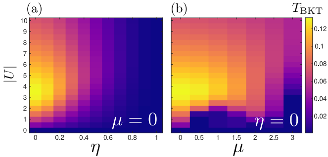
FIG. 4. BKT temperature in the Lieb lattice (a) as a function of the hopping staggering \eta and the interaction |U| , and (b) as a function of the chemical potential \mu and the interaction. The largest BKT temperature occurs around interaction U \approx -3.5 with no hopping staggering, i.e. when the flat band is not isolated.
