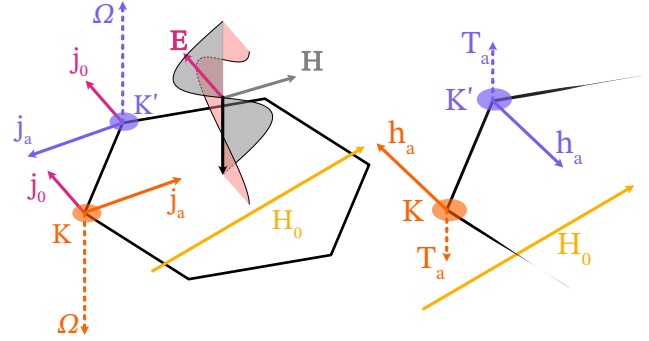
FIG. 1. (Color online) Left : Electron dipole spin resonance driven by an electromagnetic wave. The regular, \mathbf{j}_0 \propto \mathbf{E} , and anomalous, \mathbf{j}_a \propto \boldsymbol{\Omega} \times \mathbf{E} , currents at the K (orange) and K' (purple) points in the Brillouin zone, induced by the electric field \mathbf{E} of the incident electromagnetic wave. Here, \boldsymbol{\Omega} is the valley-staggered Berry curvature. Right : Anomalous fields and torques. Spins are initially polarized along the Zeeman field \mathbf{H}_0 . The anomalous current-induced effective Rashba fields, \mathbf{h}_a \propto \alpha_R \mathbf{e}_z \times \mathbf{j}_a , produce valley-specific torques \mathbf{T}_a \propto \mathbf{H}_0 \times \mathbf{h}_a , thus exciting the valley-staggered spin mode with an intensity proportional to |\mathbf{E} \times \mathbf{H}| .
