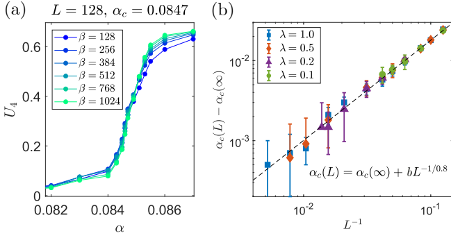
FIG. 3. Panel (a) shows U_4 for fixed \lambda = 1.0 , L = 128 , with a series of \beta , giving \alpha_c(L = 128) = 0.0847(5) . For a given \lambda , \nu and \alpha_c(\infty, \lambda) are then found by fitting the values of \alpha_c(L, \lambda) to the scaling relation L^{-1} \sim (\alpha_c(L, \lambda) - \alpha_c(\infty, \lambda))^\nu , rearranged from Eq. (10). Panel (b) shows the fits for multiple \lambda performed simultaneously, giving \nu = 0.80(5) .
