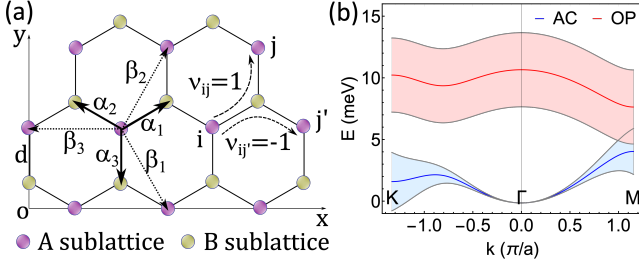
FIG. 1. (a) Ferromagnetic honeycomb lattice. \alpha_n and \beta_n are the NN and NNN bond vectors, respectively. \nu_{ij} = 1 and \nu_{ij'} = -1 label the sign of counterclockwise and clockwise DMI, respectively. (b) Spin-wave dispersions with broadening along a representative path ( \Gamma - K - M ) in the first Brillouin zone. The blue and red lines indicate the real spectra of the acoustic (AC) and optical (OP) mode, respectively. The light blue and light red shadows represent the band broadenings \Delta E_{ac} and \Delta E_{opt} , respectively. Here a = \sqrt{3}d is the distance between A-A (B-B) sublattices, where d is the NN A-B distance.
