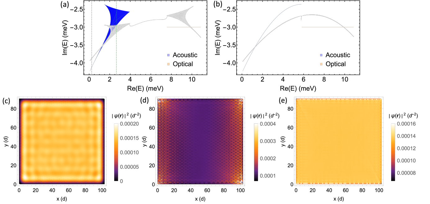
FIG. 2. (a,b) PBC spectra of the acoustic (blue) and optical (orange) modes. The OBC eigenenergies of a nanoribbon with 60 \times 60 lattice sites are shown in light gray dots. (a) For D = 0.8J/\sqrt{3} . (b) For D = 0 . (c-e) Spatial distribution of the density of the first N right eigenstates (12), (c) For D = 0.8J/\sqrt{3} and N = 79 , which corresponds to the energy \text{Re}E = 0.247 meV. This energy is indicated by the dashed red line in Fig. 2(a), up to which the acoustic spectrum is (approximately) a line. The skin effect is absent. (d) For D = 0.8J/\sqrt{3} and N = 2771 , which corresponds to the energy \text{Re}E = 2.665 meV. This energy is indicated by the dashed green line in Fig. 2(a), around which the acoustic spectrum acquires a finite effective area. The skin effect appears. (e) For D = 0 and N = 2771 there is no skin effect as the acoustic spectrum reduces to the arc shown in Fig. 2(b).
