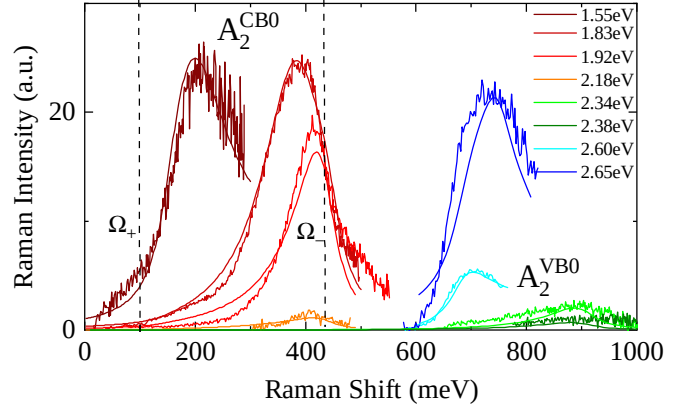
FIG. 3. The A_2 Raman excitations overlaid with calculations of the A_2 Raman response. The A_2 Raman excitations for \omega_i = 1.55 -2.65 eV are labeled as A_2^{CB0} and A_2^{VB0} to denote which Rashba continua they are originate from. The A_2^{CB0} Raman excitations are colored red and the A_2^{VB0} Raman excitations are colored green and blue. The calculated bounds of the A_2^{CB0} Rashba continuum, \Omega_{\pm} , are indicated by the dotted lines. The A_2 Raman response is calculated for \omega_i that coincides with the laser photon energy. A decay width of \gamma = 15 meV is used for the energy states.
