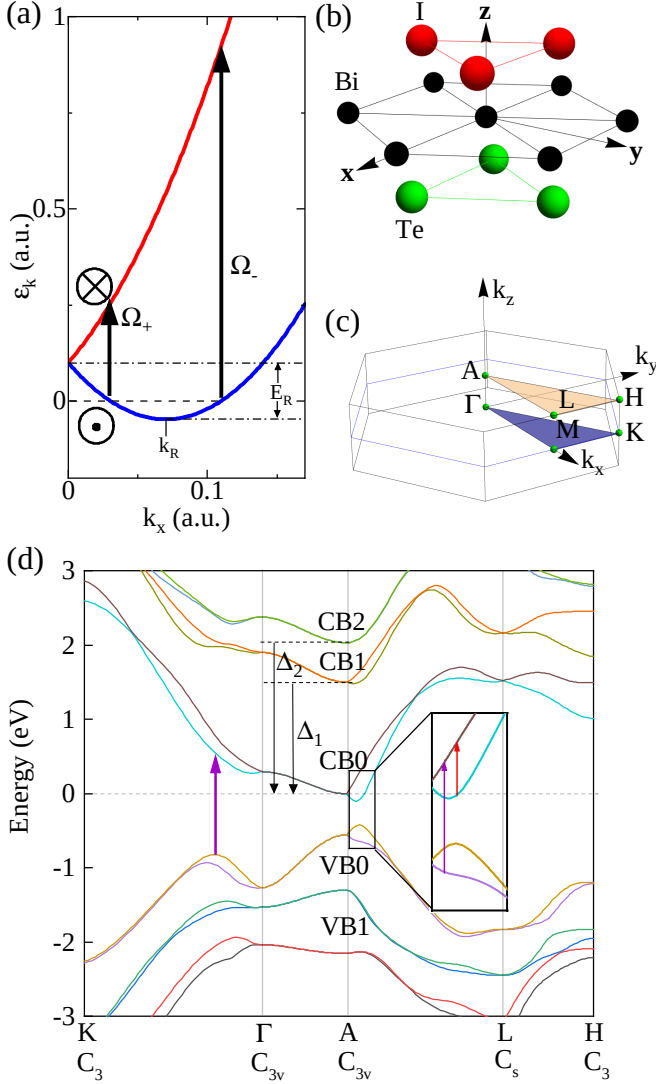
FIG. 1. Basic features of BiTeI. (a) The Rashba dispersion of a quasi-2D Rashba system. The lower sub-band reaches a minimum at k_{xy} = k_R . The energy difference between the k_{xy} = 0 and k_R points is E_R . In this example, the spin-orientation of the lower sub-band is directed out-of-page and the upper sub-band is directed in-page. The bounds of the Rashba continuum are indicated by arrows with the indices \Omega_+ and \Omega_- . (b) The crystal structure of BiTeI. (c) The Brillouin zone of P3m1 space group. (d) DFT calculation of the electronic band dispersion for BiTeI along the K- \Gamma -H-A-L directions of the Brillouin zone. The different electronic continua that are spectroscopically observed are indicated using the red and violet arrows.
