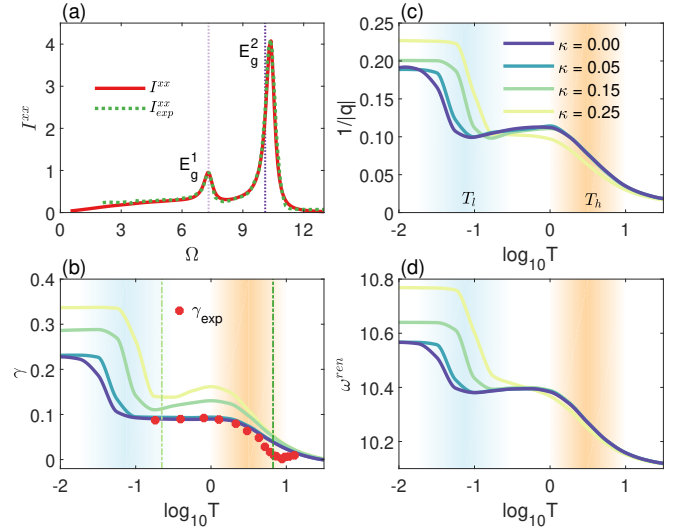
FIG. 2. Panel (a): I^{xx} and I_{\text{exp}}^{xx} are, respectively, the strMC simulated Raman intensity and the experimental intensity from Ref. [23] at T = 0.22 and \kappa = 0 . By fitting I^{xx} to the experimental intensity I_{\text{exp}}^{xx} , the best-fit model parameters are obtained: \omega_{\Gamma} = [7.31, 10.10] , \lambda_{\Gamma} = [0.25, 0.52] , \mu_{\Gamma} = [0.38, 1.00] , \nu = -0.63 . Panels (b-d): The temperature dependence of the E_g^2 peak curve parameters obtained from the asymmetric Lorentzian fitting: 1/|q| , \gamma and \omega^{\text{ren}} . T_l and T_h are two crossover temperatures. In panel (b), the computed \gamma has been offset by a background line width obtained at T = 10^{1.5} . This background line width mainly originates from the artificial broadening \delta_{\text{ph}} as shown in Sec. D of SM [49]. The red dots are experimental line width \gamma_{\text{exp}} , obtained from Ref. [23]. The two green vertical dashed lines in (e) indicate T = 5 K and 150 K. The unit conversion we use here is J \approx 23 K.
