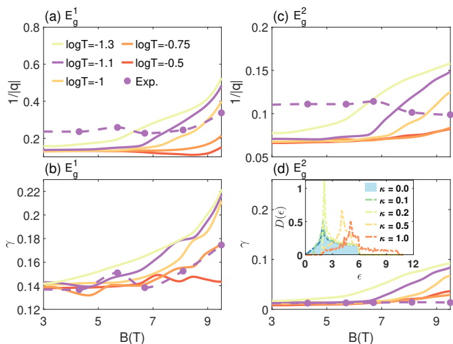
FIG. 3. The magnetic field dependence of curve parameters 1/|q| and \gamma of two phonon peaks E_g^1 and E_g^2 in the computed Raman spectrum are shown in (a,b) and (c,d), respectively. The purple dots denote experimental data from Ref. [25] measured at T = 2 K, i.e. \log T = -1.1 . The corresponding theoretical curve is also colored purple. The line width \gamma has been offset by the background contribution (see caption of Fig. 2 for the reasoning). The inset of (b) shows the density of state of Majorana fermions at various \kappa [53]. The conversion from \kappa in the unit of J to magnetic field B in the unit of Tesla follows from [29]: \kappa = \frac{(\mu_B B)^3}{\Delta_{\text{flux}}^2} , \mu_B is the Bohr magneton and \Delta_{\text{flux}} = 0.27J is the flux energy, and J \approx 23 K.
