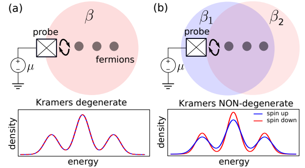
FIG. 1. (a) A fermionic system (three small circles) coupled to an environment (big circle) in thermal equilibrium at temperature \beta^{-1} has a Kramers' degeneracy. (b) The same system (three small circles) coupled to two baths (two big circles) at different temperatures \beta_1^{-1} , \beta_2^{-1} will not be Kramers'-degenerate. This leads to a spin splitting of the Green's function (13), which can be experimentally detected using, e.g. spin-resolved tunneling spectroscopy (bottom panels). For both (a) and (b), the system-bath Hamiltonian obeys TRS: [H_{SB}, T] = 0 .
