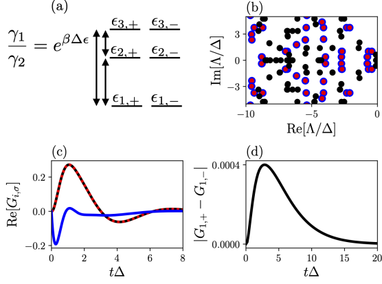
FIG. 2. (a) Three doubly degenerate energy levels ( N = 3 ) labeled by \epsilon_{i,\pm} . TRS-respecting dissipators cause jumps between energy levels at a rate consistent with detailed balance in thermal equilibrium at temperature \beta^{-1} . (b) Lindblad spectrum for the model described in the main text (for states with 0, 1, or 2 occupied fermions) at a temperature \beta\Delta = 1 , with N = 3 , \Delta_d/\Delta = 0.1 , and g/\Delta = 1 . The odd-superparity sector (blue and red dots) is twofold degenerate, while the even sector (black dots) is not. (c) Real part of the retarded Green's function for same parameters as in (b). The Kramers' degeneracy ensures that G_{i,\sigma} = G_{i,-\sigma} in the expectation value of the thermal steady state with one occupied fermionic mode: black line and red dashed line correspond to \text{Re}[G_{1,+}] and \text{Re}[G_{1,-}] , respectively. In general, Green's function pairs other than G_{i,\pm} are non-degenerate: blue line corresponds to \text{Re}[G_{2,+}] . (d) A system that is coupled to two thermal baths g_1/\Delta = 1, g_2/\Delta = 0.4 at different temperatures: \beta_1\Delta = 1, \beta_2\Delta = 10 [otherwise same parameters as in (b)]. Microreversibility is broken, hence the Green's functions for i, + and i, - split.
