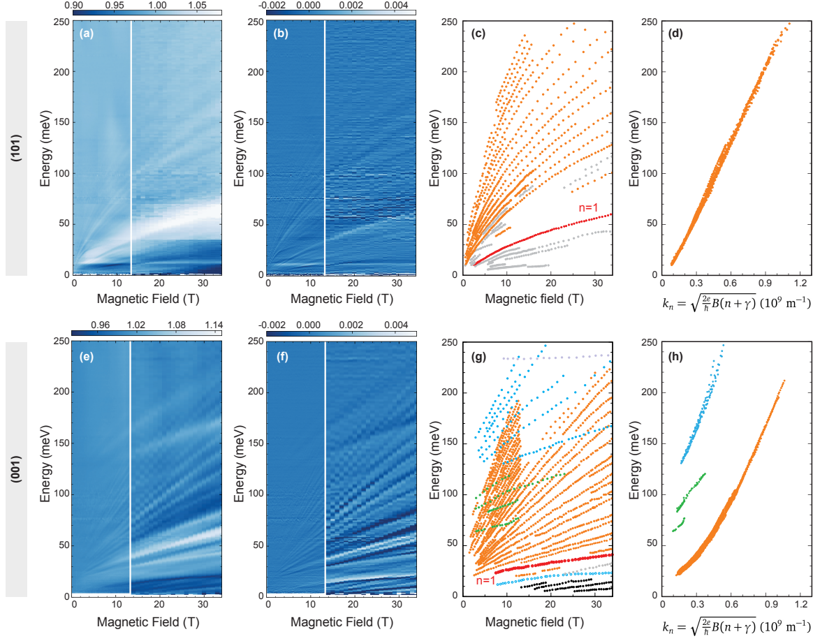
Figure 2. Inter Landau-level transitions in (101) (top) and (001) planes (bottom). Relative magneto-reflectance R_B/R_0 is shown in panels (a) and (e), and its derivative in (b) and (f). The inter-LL transitions are isolated in (c) and (g). They are plotted in (d) and (h) as a function of momentum k_n = \sqrt{2eB(n+\gamma)}/\hbar , with \gamma = 0 .
