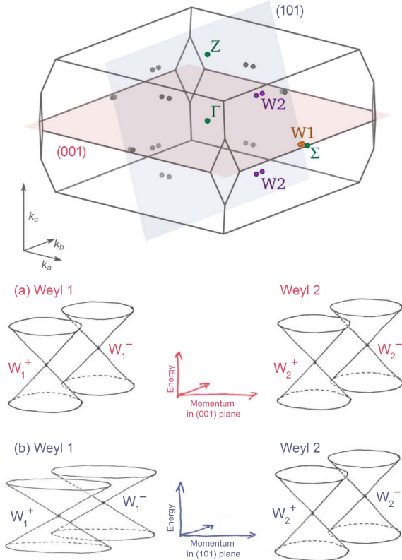
Figure 1. Top: Brillouin zone of TaAs, with (001) and (101) planes shown in red and blue, respectively. Following the band structure calculations [12], we sketch the W_1 and W_2 Weyl cones (a) in the (001) plane, and (b) in the (101) plane.
