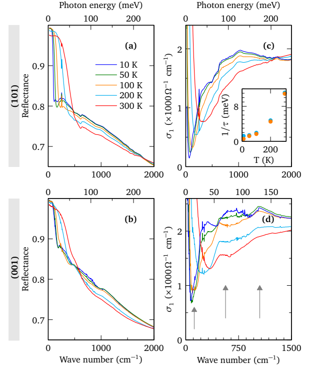
Figure 3. Zero-field optical properties of TaAs, for (101) (top) and (001) plane (bottom panels). Far-infrared reflectance is shown in (a) and (b) as a function of photon energy, at different temperatures. The real part of optical conductivity, \sigma_1 , is shown in (c) and (d). Grey arrows indicate the 15 meV absorption onset, and van Hove peaks at 70 meV and 128 meV. Inset shows the temperature dependence of scattering rate 1/\tau for the two planes.
