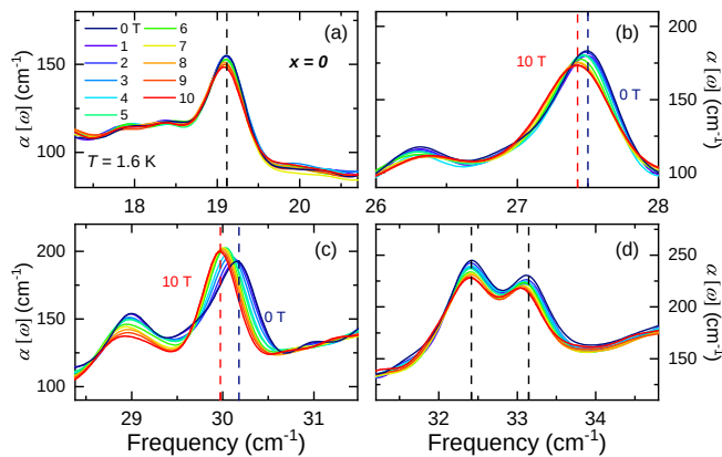
FIG. 5. (a-d) Evolution of the frequency-dependent absorption coefficient \alpha(\omega) under external magnetic field for \text{Cu}_5\text{V}_2\text{O}_{10}(\text{CsCl}) at T = 1.6 K. The black dashed lines indicate those modes which do not shift in field, but only modify their intensity. The ones with both intensity and frequency shifts are marked at the center frequency at zero field (blue) and 10 T (red) with dashed lines [panel (b,c)].
