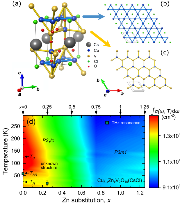
FIG. 1. Crystal structure of the Averievite \text{Cu}_{5-x}\text{Zn}_x\text{V}_2\text{O}_{10}(\text{CsCl}) . The P\bar{3}m1 structure is found for x = 0 only for T > 310 K while for x = 1 in the entire temperature range. (a) A single unit cell representation. Two different in-plane ( ab ) sheets are stacked along the c -direction. One is the kagome structure (b) comprised of Cu atoms and the other is a honeycomb lattice (c) consisting of V and Cu. Overall, Averievite crystallizes in alternating kagome and two honeycomb lattices. (d) Structural and magnetic properties of Averievite, T_S = 127 K: structural transition, T_{SR} \approx 60 K: onset of short-range correlations, T_N = 24 K: long-range order. False-color plot is based on the integrated absorption coefficient \int \alpha(\omega, T) d\omega obtained for different Zn concentrations (indicated by vertical arrows at the top). Dark green points: Onset of magnetic THz resonances.
