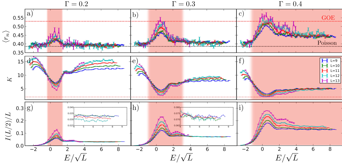
FIG. 2. Energy-dependence of localization via three metrics: (a-c) level statistic \langle r_n \rangle , (d-f) Kullback-Leibler divergence (KLd), and (g-i) half-system mutual information ( I(L/2) ). The shaded red color indicates the approximate region of delocalization, based on finite-size crossings of the KLd. Inset plots show magnification of I(L/2)/L for higher energy data.
