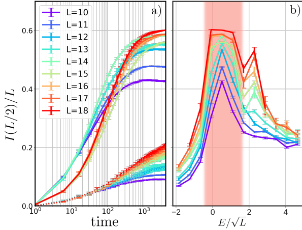
FIG. 3. (a) Dynamics of I(L/2) obtained using Krylov time evolution starting from a product state. Dashed curves correspond to the MBL regime ( E/\sqrt{L} = -1.26 \pm 0.024 ) and solid lines correspond to the delocalized regime ( E/\sqrt{L} = 0.51 \pm 0.024 ). (b) Energy dependence of I(L/2) at late time, t = 3900 . All data are for \Gamma = 0.3 . In this plot, the finite size effect is strong as going from L = 14 to L = 15 the form of plot changes significantly.
