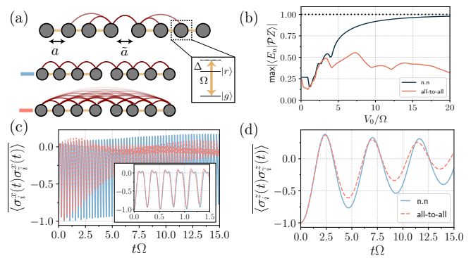
FIG. 4. Dynamical signature in a chain of interacting Rydberg atoms. (a) Depiction of a non-uniformly spaced Rydberg chain. (b) Maximum overlap of |Z\rangle projected into the sub-sector absent of neighboring Rydberg states for different interaction strengths. Nearest-neighbor (all-to-all) interactions is denoted by blue(red). (c) Dynamics of the average expectation value between inversion pairs, \langle \sigma_i^x(t) \sigma_j^x(t) \rangle prepared in |Z\rangle . Inset: Short time dynamics for t\Omega \sim 1.5 . (d) Néel state dynamics for the correlator, \langle \sigma_i^z(t) \sigma_j^z(t) \rangle . Parameters used in (b), (c) and (d): \Omega/2\pi = 2\text{MHz} , V_0 = 12\Omega , \Delta_{\text{opt}} = V_0/2\tilde{a}^6 with \tilde{a} \sim 1.51 and 2N = 16 .
