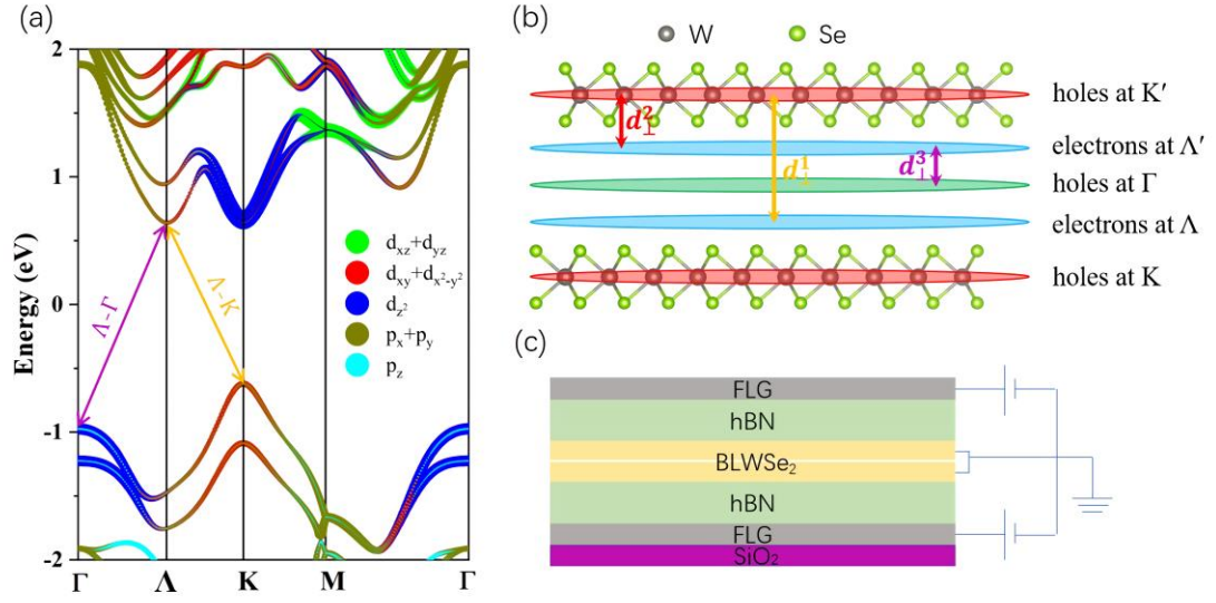
FIG. 1. (a) Orbital projected band structures of bilayer WSe 2 . Symbol size is proportional to its population in corresponding state. (b) Schematic image of the equivalent positions of spin-up wavefunctions at K/K' (red ellipses), \Lambda/\Lambda' (blue ellipses) and \Gamma points (green ellipse) in real space. d_{\perp}^{1-3} denote vertical distances between different wavefunctions. (c) Schematic of h -BN encapsulated bilayer WSe 2 device.
