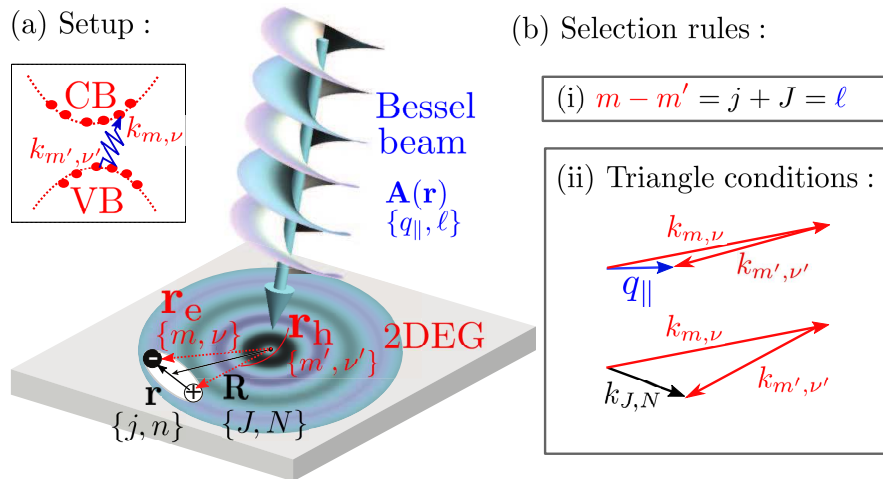
FIG. 1. (a) A Bessel light beam \mathbf{A} with photon momentum/angular momentum (q_{\parallel}, \ell) creates an electron-hole pair in a 2D electron gas (2DEG). The electron [hole] is characterized by quantum numbers (m, \nu) [ (m', \nu') ] for angular momentum/momentum. The pair can form a bound state, and the degrees of freedom of such an exciton are the center-of-mass motion, characterized by angular momentum/momentum quantum numbers (J, N) , and the relative motion, characterized by quantum numbers (j, n) for angular momentum and energy. (b) The selection rules for optical transitions and exciton formation reflect (i) conservation of angular momentum, and (ii) conservation of linear momentum, reflected by the illustrated triangle conditions.
