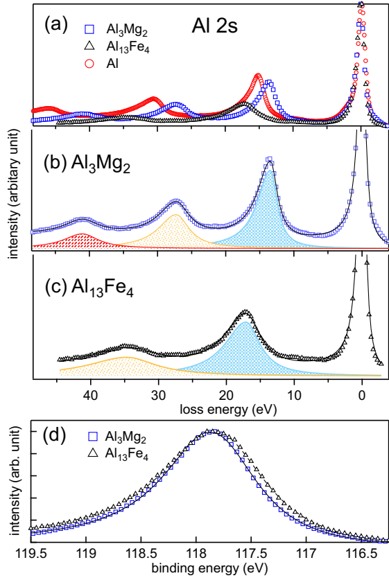
FIG. 7. (a) Al 2s HAXPES core-level spectra showing the plasmon loss region for \beta -Al 3 Mg 2 , Al 13 Fe 4 and Al metal taken with 6 keV. The spectra are normalized to the same intensity at the main peak that is aligned to zero in the energy loss scale. The least square fitting (black curve) of the plasmon loss region of (b) \beta -Al 3 Mg 2 and (c) Al 13 Fe 4 . The 1\omega_p , 2\omega_p , and 3\omega_p plasmon peaks are shaded by cyan, yellow and red colors, respectively. (d) The Al 2s main peak of \beta -Al 3 Mg 2 and Al 13 Fe 4 along with the fitted solid and dashed curves, respectively.
