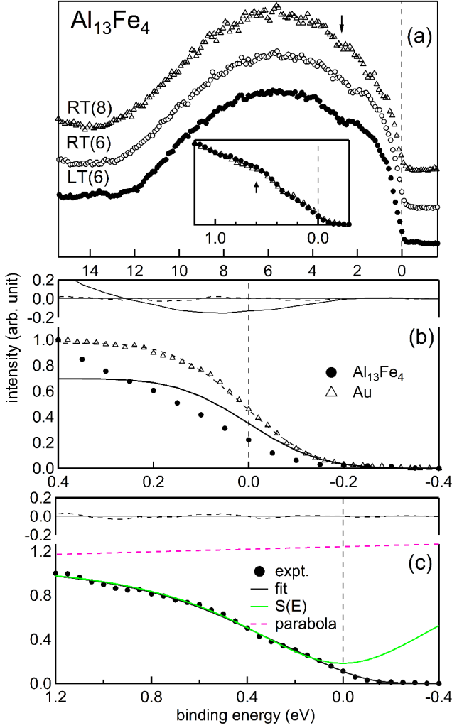
FIG. 4. (a) HAXPES VB spectrum of \text{Al}_{13}\text{Fe}_4 taken at RT and LT, the photon energy in keV is given within the brackets. Inset shows the near- E_F region. (b) The near- E_F region of \text{Al}_{13}\text{Fe}_4 and Au at LT. The fitted curves (and residuals in the upper region) are shown by continuous and dashed lines for \text{Al}_{13}\text{Fe}_4 and Au, respectively. (c) The near E_F region of \text{Al}_{13}\text{Fe}_4 fitted using S(E) (green curve), which is given by an inverted Lorentzian function multiplied by a free electron parabola (Equation 1). The residual (black dashed curve) is shown in the upper region.
