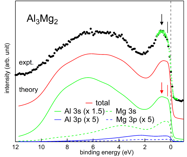
FIG. 3. The calculated VB (red curve) of \beta\text{-Al}_3\text{Mg}_2 along with the partial contributions compared with the HAXPES VB spectrum (black filled circles) taken at LT. The spectra are staggered along the vertical axis for clarity of presentation. The near- E_F region of the HAXPES VB spectrum (green open circles) recorded with smaller step size at LT is overlaid on the wide range VB spectrum. The experimental VB spectra are shifted by the 95 meV towards E_F to compensate for the recoil effect that is not considered in the calculation.
