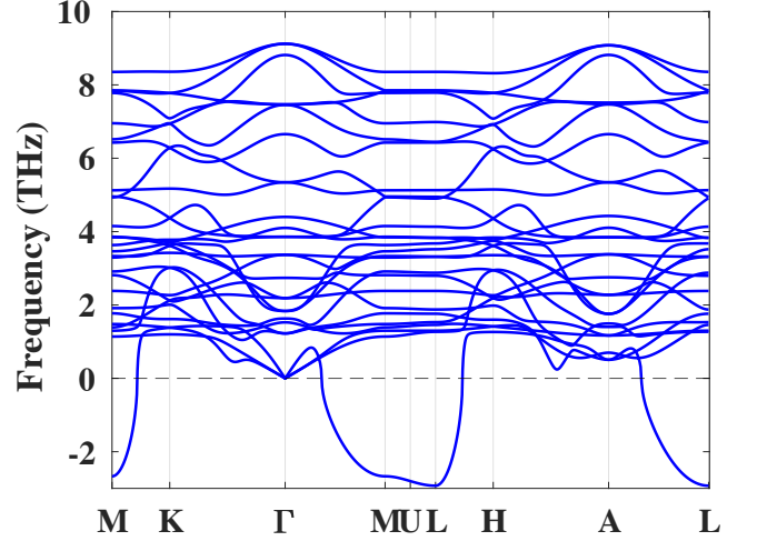
FIG. 15. DFT calculation of phonon dispersion in the whole Brillouin zone for the high-temperature phase of \text{CsV}_3\text{Sb}_5 .
