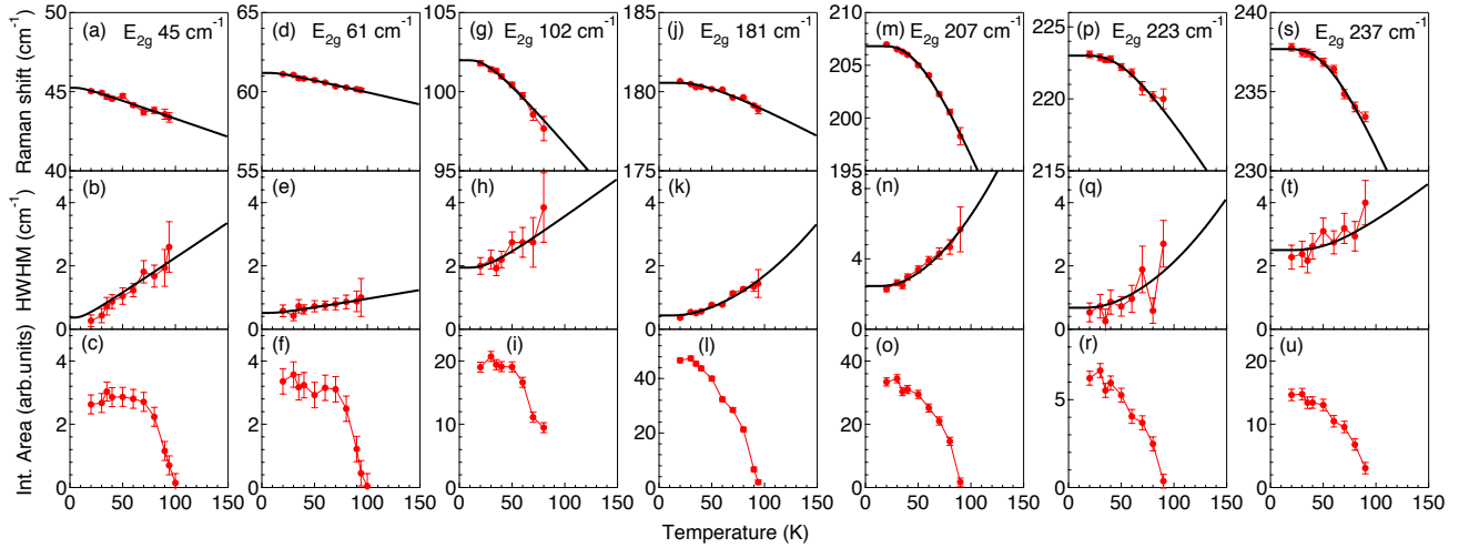
FIG. 13. T -dependence of the peak position, HWHM and integrated intensity for the new E_{2g} phonon modes below T_S for \text{CsV}_3\text{Sb}_5 . (a)-(c) is for the mode at 45\text{ cm}^{-1} . (d)-(f) is for the mode at 61\text{ cm}^{-1} . (g)-(i) is for the mode at 102\text{ cm}^{-1} . (j)-(l) is for the mode at 181\text{ cm}^{-1} . (m)-(o) is for the mode at 207\text{ cm}^{-1} . (p)-(r) is for the mode at 223\text{ cm}^{-1} . (s)-(u) is for the mode at 237\text{ cm}^{-1} . The error bars represent one standard deviation. For fitting of the phononic self-energy T -dependence for the modes at 45\text{ cm}^{-1} , 61\text{ cm}^{-1} , and 102\text{ cm}^{-1} , Eq. F1 and Eq. F2 are used; For the modes at 181\text{ cm}^{-1} , 207\text{ cm}^{-1} , and 223\text{ cm}^{-1} , Eq. F1 and F2 are used.
