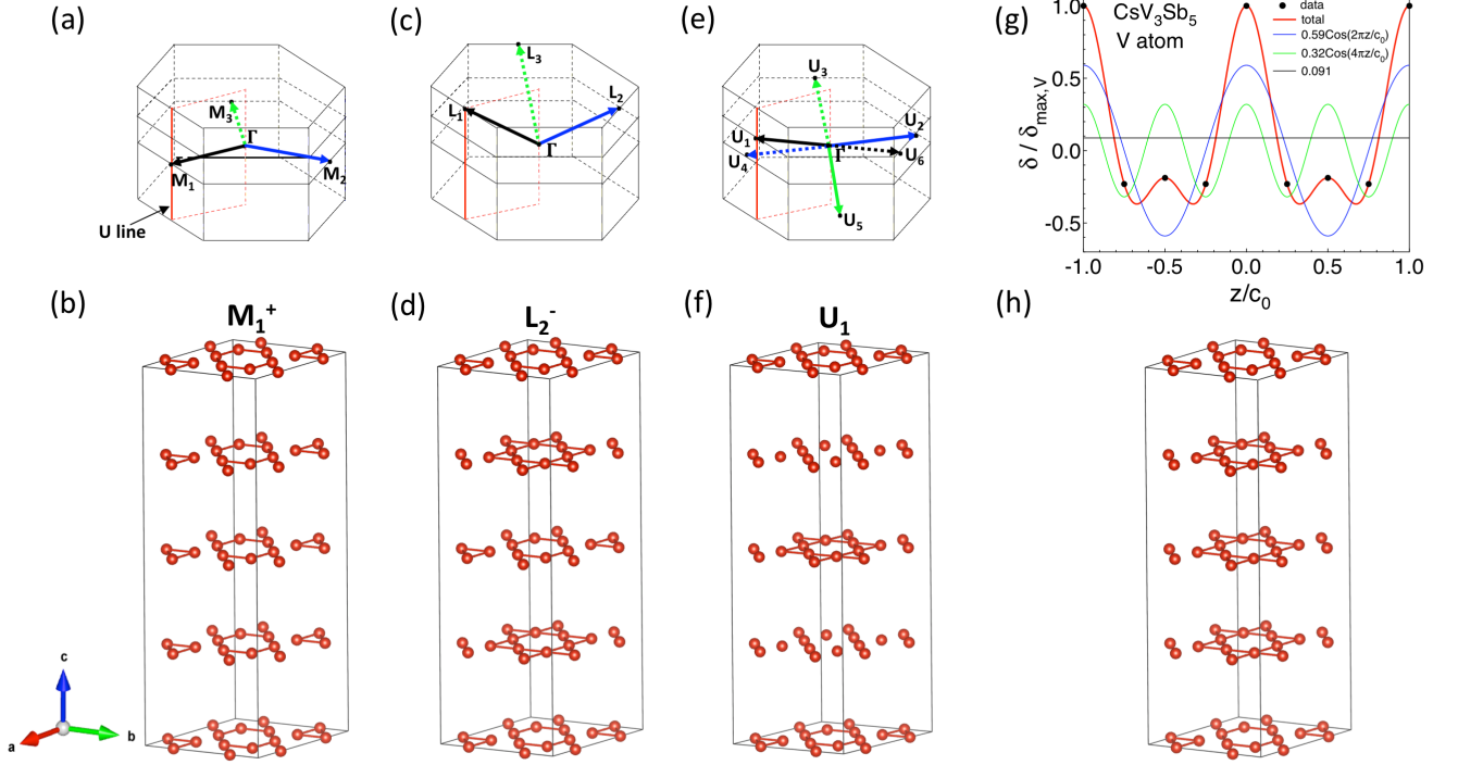
FIG. 3. The 3D hexagonal Brillouin zone (BZ) corresponds to the space group P6/mmm with M , L , and U points highlighted, as well as the U -line connecting M and L shown in red. (a) The three vectors in the stars of M points, leading to 2 \times 2 \times 1 CDW ordering shown as bond patterns in (b). (c) The three vectors in the stars of L points, contributing to 2 \times 2 \times 2 CDW ordering shown as bond patterns in (d). (e) The six vectors in the stars of U points, which give rise to 2 \times 2 \times 4 CDW ordering shown as bond patterns in (f). For these vectors shown in (a), (c), and (e), the solid arrows are pointing to the front faces while the dashed arrows are pointing to the back faces. (g) The normalized in-plane amplitude of V-displacements at 6j site \delta/\delta_{\max,V} in the kagome layer as a function of the normalized coordinate ( z/c_0 ) for the 2 \times 2 \times 4 structure of \text{CsV}_3\text{Sb}_5 at 15 K. c_0 is the c -axis lattice constant for the four-layer structure. The solid red, blue, and green lines represent the total fitted curve, the c_0 -cosinusoidal modulation component, and the c_0/2 -cosinusoidal modulation component, respectively. (h) Illustration of the 2 \times 2 \times 4 structure for Vanadium lattice [36]. In (b), (d), (f), and (h), the Cs and Sb atoms are omitted for simplification.
