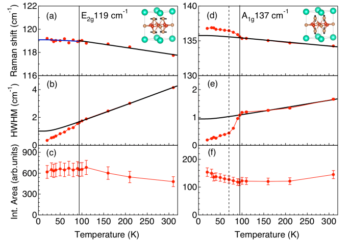
FIG. 11. T -dependence of the peak position (a), HWHM (half width at half maximum) (b) and integrated intensity (c) for the main E_{2g} phonon at 119 cm -1 for CsV 3 Sb 5 . (d)-(f) Same as (a)-(c) but for the main A_{1g} phonon at 137 cm -1 . The error bars represent one standard deviation. The solid black and blue lines represent the fitting of the phononic self-energy T -dependence above T_S and below T_S by anharmonic decay model, respectively [Eq. F1 and F2]. The solid vertical lines represent T_S while the dashed black lines represent T^* . The insets of (a) and (d) show the lattice vibration patterns for the E_{2g} phonon and A_{1g} phonon, respectively.
