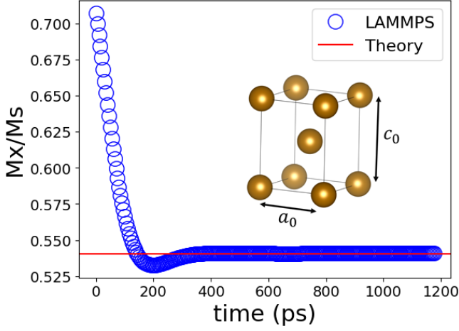
FIG. 13. Test for the correct implementation of the anisotropy field. Simulated dynamics of the x-component of the normalized magnetization M_x/M_S with (blue circles) the SPIN package 52 of LAMMPS 46 for BCC Fe under a tetragonal deformation \tau = c_0/a_0 = 1.02 , where a_0 = 2.83023 \text{ \AA} . The red line represents the theoretical equilibrium x-component of the normalized magnetization M_{x,eq}/M_S given by Eq.C9. The initial direction of the normalized magnetization is M_x(0)/M_S = 1/\sqrt{2} , M_y(0)/M_S = 0 , and M_z(0)/M_S = 1/\sqrt{2} , while the applied magnetic field is \mu_0\mathbf{H} = (0.05, 0, 0) \text{ T} . In this test we used the parameters given in Section II B, but we don't include the quadrupole term ( q(r_{ij}) = 0 ) in order to be consistent with the theoretical derivation of Eq.C9. Moreover, we perform only spin dynamics (frozen lattice) with high LLG damping to speed up the convergence to the equilibrium state.
