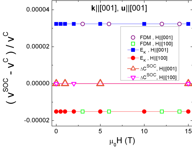
FIG. 8. Fractional change in velocity of BCC Fe versus the magnitude of the applied magnetic field along \mathbf{H} \parallel [100] and \mathbf{H} \parallel [001] for a longitudinal wave propagating along \mathbf{k} \parallel [001] with polarization \mathbf{u} \parallel [001] . Open green squares and purple circles stand for the calculations with spin-lattice simulations obtained from the FDM for the cases \mathbf{H} \parallel \mathbf{M} \parallel [100] and \mathbf{H} \parallel \mathbf{M} \parallel [001] , respectively. Red points and blue squares stand for the calculations with spin-lattice simulations obtained from the oscillation of the kinetic energy for the cases \mathbf{H} \parallel \mathbf{M} \parallel [100] and \mathbf{H} \parallel \mathbf{M} \parallel [001] , respectively. Open orange and pink triangles represent the calculations using the corrections to the elastic constants given by Eq.A24 for the cases \mathbf{H} \parallel \mathbf{M} \parallel [100] and \mathbf{H} \parallel \mathbf{M} \parallel [001] , respectively.
