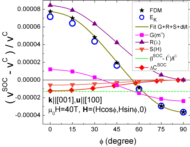
FIG. 6. Fractional change in velocity of BCC Fe versus the direction of the applied magnetic field \mathbf{H} = (H \cos \phi, H \sin \phi, 0) on the plane XY for transverse wave propagating along \mathbf{k} \parallel [001] with polarization \mathbf{u} \parallel [100] . The magnitude of the applied field is \mu_0 H = 40 T. Black stars represent the calculations with spin-lattice simulations obtained from the FDM, while brown solid line is the fitting of these data to the summation of functions G , R , S and (l^{SOC} - l^C)/l^C in Eq.23. Blue circles stand for the calculations with spin-lattice simulations obtained from the oscillation of the kinetic energy ( E_K ). Each function G , R , S and (l^{SOC} - l^C)/l^C in Eq.23 is plotted with pink squares, purple triangles, orange triangles and green dash line, respectively. Red diamonds correspond to the calculations using the corrections to the elastic constants given by Eq.A22.
