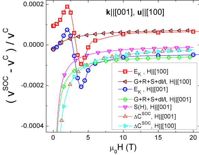
FIG. 7. Fractional change in velocity of BCC Fe versus the magnitude of the applied magnetic field along \mathbf{H} \parallel [100] and \mathbf{H} \parallel [001] for a transverse wave propagating along \mathbf{k} \parallel [001] with polarization \mathbf{u} \parallel [100] . Blue points and red squares stand for the calculations with spin-lattice simulations obtained from the oscillation of the kinetic energy for the cases \mathbf{H} \parallel [100] and \mathbf{H} \parallel [001] , respectively. Brown triangles and green diamonds correspond to the summation of functions G , R , S and (I^{SOC} - I^c)/I^c in Eqs.23 and 24 for the cases \mathbf{H} \parallel [100] and \mathbf{H} \parallel [001] , respectively. The function S(H) in Eq.24 is plotted with pink triangles. Orange and cyan triangles represent the calculations using the corrections to the elastic constants given by Eq.A22.
