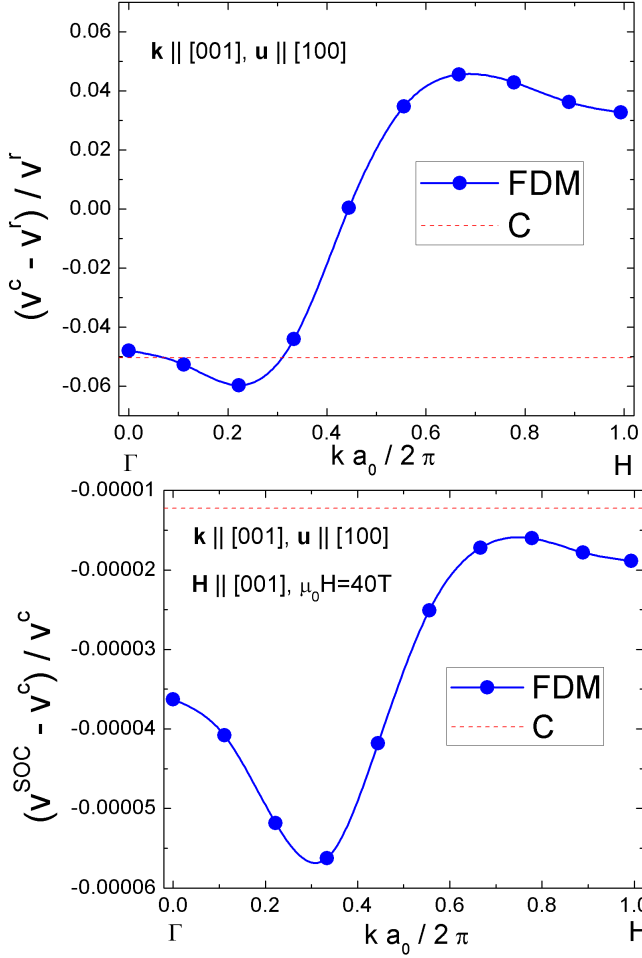
FIG. 10. Fractional change in group velocity of phonons versus phonon's momentum along \mathbf{k} \parallel [001] with polarization \mathbf{u} \parallel [100] . (Top) Fractional change in velocity of the collinear state (including only exchange interaction) with respect to the paramagnetic state with randomly oriented magnetic moments in 3D. (Bottom) Fractional change in velocity of the collinear state (including both exchange interaction and SOC) with respect to collinear state including only exchange interaction. The calculations are performed using the FDM. Red dash line represents the calculation with the corrections to the elastic constants given by Eqs.A21 and A22.
