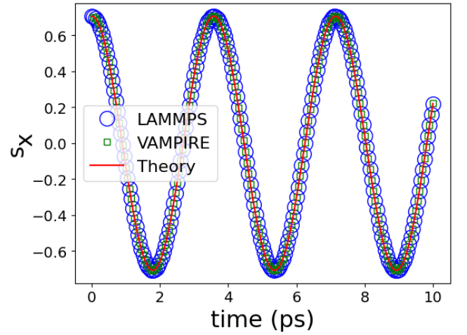
FIG. 12. Test for the correct implementation of the applied magnetic field. Simulated dynamics of the x-component of the normalized magnetic moment s_x with (blue circles) the SPIN package 52 of LAMMPS 46 and (green squares) VAMPIRE code 44 . The red line represents the theoretical solution given by Eq.C2. The initial direction of the normalized magnetic moment is s_x(0) = 1/\sqrt{2} , s_y(0) = 0 , and s_z(0) = 1/\sqrt{2} , while the applied magnetic field is \mu_0 H = 10 \text{ T} .
