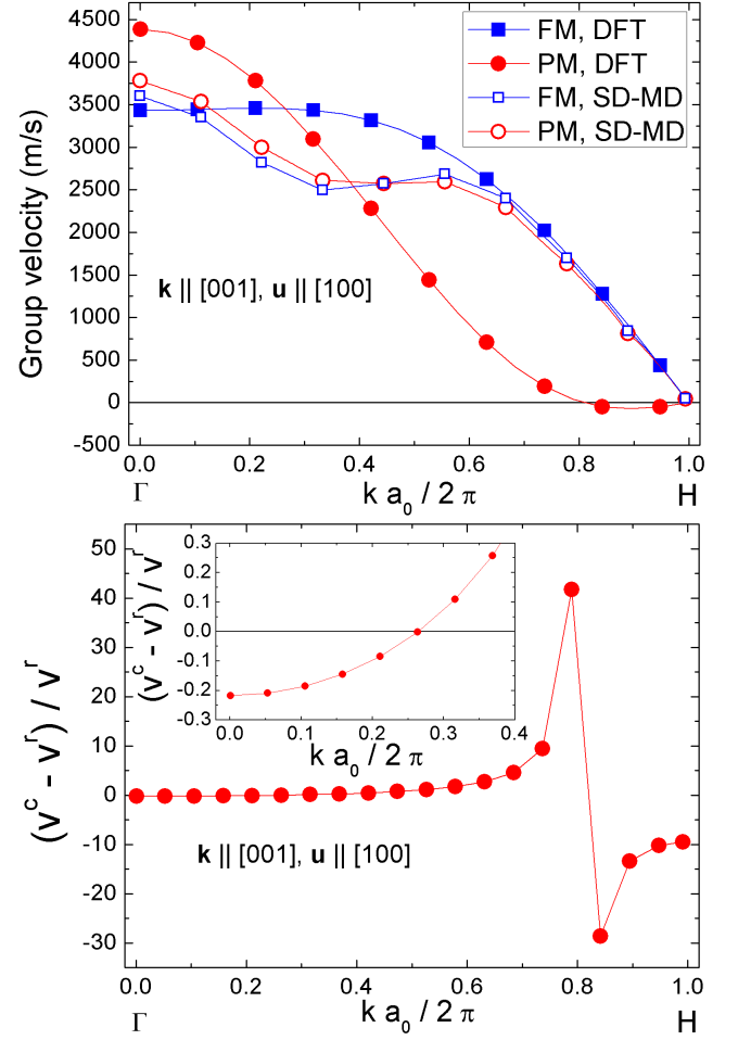
FIG. 11. (Top) Group velocity of phonons versus phonon's momentum along \mathbf{k} \parallel [001] with polarization \mathbf{u} \parallel [100] at ferromagnetic (FM, v^c ) and paramagnetic (PM, v^r ) state calculated with (solid symbols) DFT and (open symbols) SD-MD. (Bottom) Fractional change in group velocity of the collinear state (including only exchange interaction) with respect to the PM state given by DFT calculation. In the inset we zoom in the low phonon momentum regime ( ka_0/2\pi < 0.4 ). The DFT calculation was obtained by reproducing the work done by Ikeda et al. 79 using SQS within the FDM.
