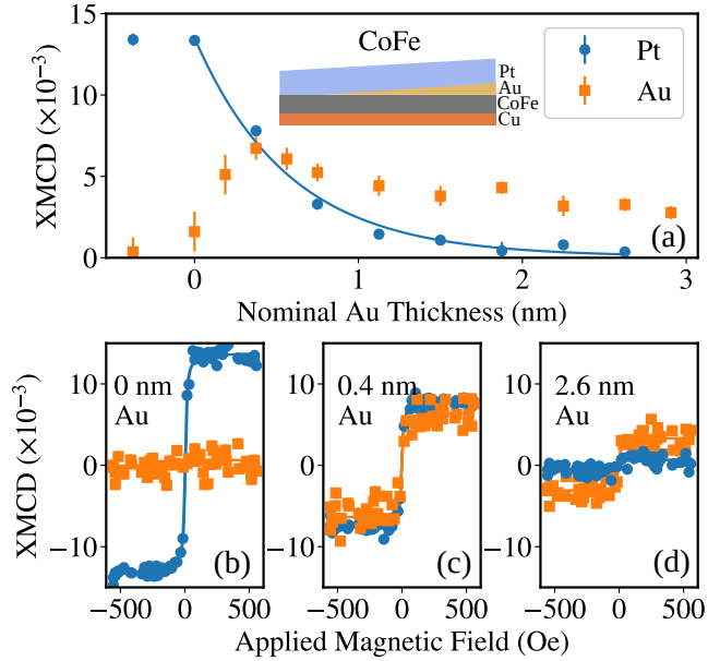
FIG. 11: (a) Measured XMCD as a function of Au spacer thickness at both the Pt (blue) and Au (orange) L_3 edges, with element specific hysteresis loops at three positions across the wedge, for (b-d) Cu(2 nm)/CoFe(7 nm)/Au/Pt(4 nm). Solid lines in (a) are best fitting exponential functions.
