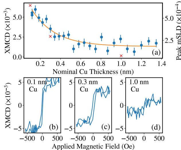
FIG. 4: (a) Measured XMCD peak intensity at Pt L_3 edge as a function of Cu SL thickness (blue dots) in the Cu/CoFe(7nm)/Cu( t )/Pt(10nm) system. The solid line shows the best fitting exponential function and red crosses show the peak mSLD data for comparison. (b,c,d) Pt hysteresis loops taken at three Cu thicknesses.
