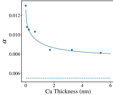
FIG. 2: Gilbert damping parameter as a function of Cu SL thickness for the Cu/CoFe(7nm)/Cu( t )/Pt(10nm) system. The horizontal dashed line represents the damping in native CoFe. The solid line is a best fitting exponential function.
