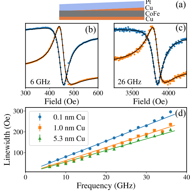
FIG. 1: (a) Schematic showing the sample structure with the Cu spacer layer thickness wedge. (b,c) Examples of the fitted FMR signals as a function of applied magnetic field at 6 GHz and 26 GHz for a 1 nm Cu SL thickness and (d) representative frequency dependence of FMR field linewidth with linear fits for three Cu spacer layer thicknesses.
