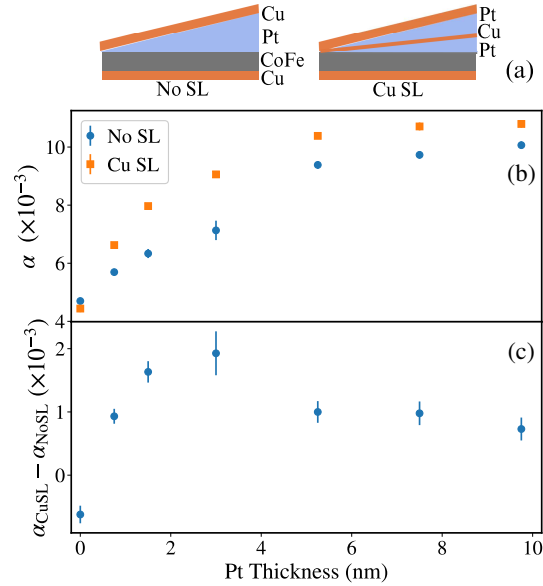
FIG. 6: (a) Schematic of systems with and without a Cu SL within the Pt. (b) Measured damping parameter from the FMR linewidth for Cu(2 nm)/CoFe (7 nm)/Pt ( t nm) and Cu(2 nm)/CoFe (7 nm)/Pt ( t/2 nm)/Cu(5 nm)/Pt ( t/2 nm) systems. (c) Difference in the damping parameter between the two systems.
