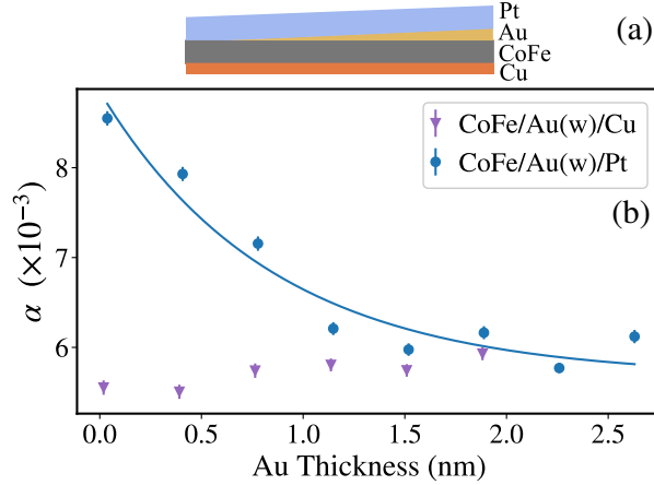
FIG. 7: (a) Schematic illustration of Cu/CoFe/Au( t )/Pt structure. (b) Intrinsic damping contribution, \alpha , as a function of Au thickness for the multilayers detailed in the legend.
