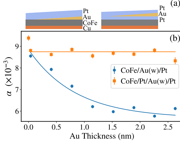
FIG. 13: (a) Schematic illustration of Au SL structure. (b) Intrinsic damping contribution, \alpha , to the FMR linewidth as a function of Au thickness for multilayer detailed in the legend. The solid blue line is a best fitting exponential.
