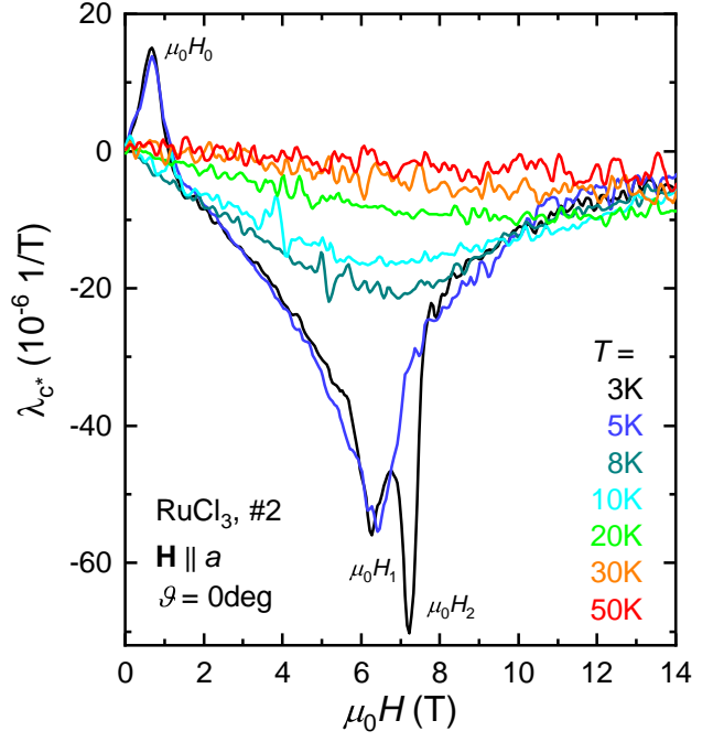
FIG. 2. (Color online) Magnetic field dependence of the \lambda_{c^*} linear magnetostriction coefficient at selected temperatures. The \Delta L length change was measured along the c^* axis and \mathbf{H} \parallel a magnetic field was applied, perpendicular to one of the Ru-Ru bonds.
