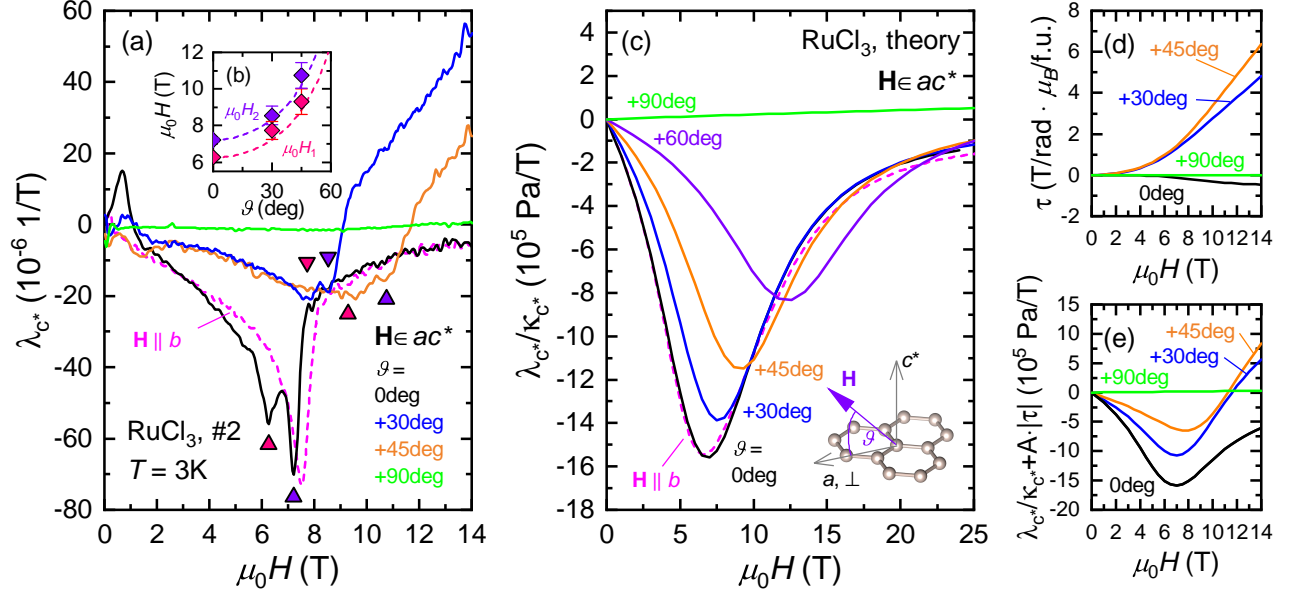
FIG. 3. (Color online) (a) Field dependence of the linear magnetostriction coefficient \lambda_{c^*} at T=3 \text{ K} . The magnetic field was applied along the main crystallographic axes, as well as canted out of the ab plane with projection perpendicular to the bond ( \mathbf{H} \in ac^* ). The \vartheta=0^\circ and 90^\circ angles correspond to the a and c^* axes, respectively. The two peaks in the \lambda_{c^*} data correspond to (\mu_0 H_1) a phase transition between different zigzag interplane orderings and (\mu_0 H_2) a transition into the field-induced quantum paramagnetic phase. The \mu_0 H_1 and \mu_0 H_2 phase boundaries are indicated by triangles, respectively. (b) Angular dependence of the \mu_0 H_1 and \mu_0 H_2 phase transition fields. The dashed lines indicate the \sim 1/\cos \vartheta field dependence. (c) The field dependence of the \lambda_{c^*}/\kappa_{c^*} magnetostriction calculated for H field canted out of the ab plane with \vartheta angle, \mathbf{H} \in ac^* . The inset defines the field angle \vartheta . Note, that panels (a) and (c) are shown for different field scales. (d) Magnetic field dependence of the calculated \tau magnetic torque for selected \vartheta canting angles, \mathbf{H} \in ac^* . (e) The effect of magnetic torque on the field-dependence of the magnetostriction is modelled with the \lambda_{c^*}/\kappa_{c^*} + A \cdot |\tau| relation with the same A=2.2 \cdot 10^5 \text{ Pa} \cdot \text{Rad} / (\text{T}^2 \cdot \mu_B/\text{f.u.}) parameter fitted for each curve.
