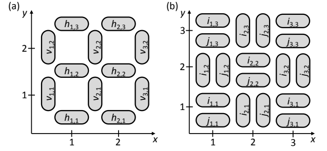
FIG. 7. Numbering of the islands in the a) square and b) quadrupolar lattices, using which the AF, FQ, and AFQ order parameters are calculated as described in the Appendix.
