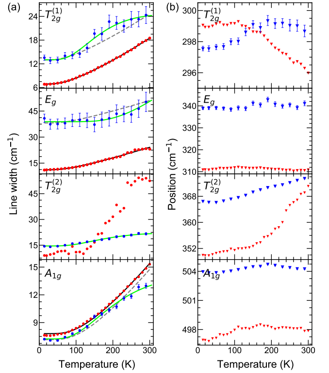
FIG. 5. Temperature dependence of (a) line widths and (b) positions for \text{Pr}_2\text{Zr}_2\text{O}_7 (blue) and \text{Pr}_2\text{Ir}_2\text{O}_7 (red). Black lines are fits of line width of \text{Pr}_2\text{Zr}_2\text{O}_7 phonons with extended Klemens model. Dashed lines show the same temperature dependence with \Gamma_0 increased for \text{Pr}_2\text{Ir}_2\text{O}_7 . Green lines are the fits of line width of \text{Pr}_2\text{Ir}_2\text{O}_7 phonons by the phonon-electron scattering model. Note that the temperature dependence for \text{Pr}_2\text{Ir}_2\text{O}_7 phonons is best fit by phonon-electron scattering.
