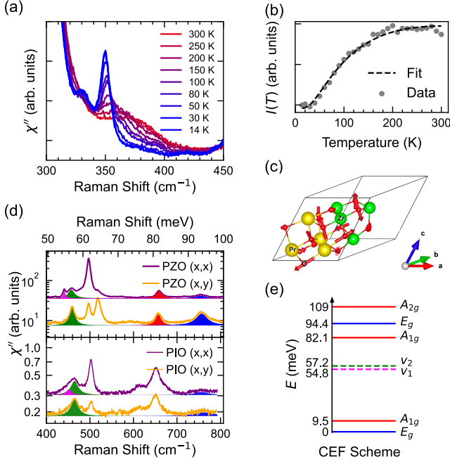
FIG. 4. (a) Temperature dependence of Raman scattering spectra of \text{Pr}_2\text{Zr}_2\text{O}_7 in the region of A_{1g} \rightarrow E_g crystal electric field transitions in (x, y) channel. (b) Temperature dependence of spectral weight I(T) = \int_{430}^{330} \chi''(\omega) d\omega . (c) Atomic displacement of T_{2g}^{(2)} phonon mode. (d) Raman spectra of \text{Pr}_2\text{Zr}_2\text{O}_7 (upper panel) and \text{Pr}_2\text{Ir}_2\text{O}_7 (lower panel) at 14 K in (x, x) and (x, y) channel on a log scale. Crystal field excitations are marked in different colors. Note the double feature of the excitation at about 450 \text{ cm}^{-1} for both materials. (e) Crystal field scheme of \text{Pr}^{3+} ions in D_{3d} crystal environment. Energy values are provided for \text{Pr}_2\text{Zr}_2\text{O}_7 .
