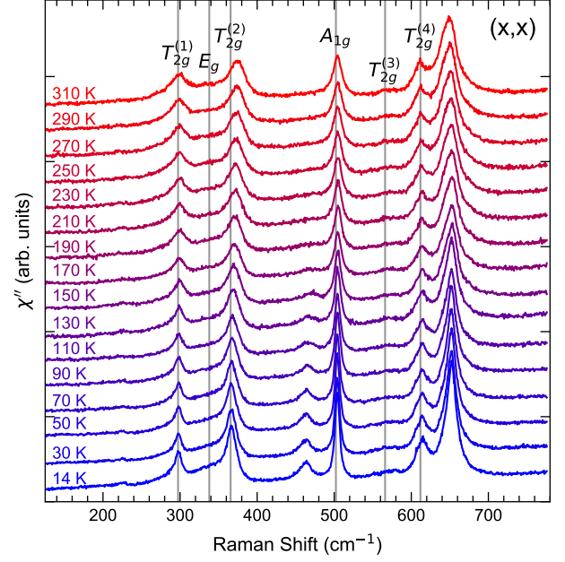
FIG. 3. Temperature dependence of the Raman scattering spectra of \text{Pr}_2\text{Ir}_2\text{O}_7 in (x, x) channel.
