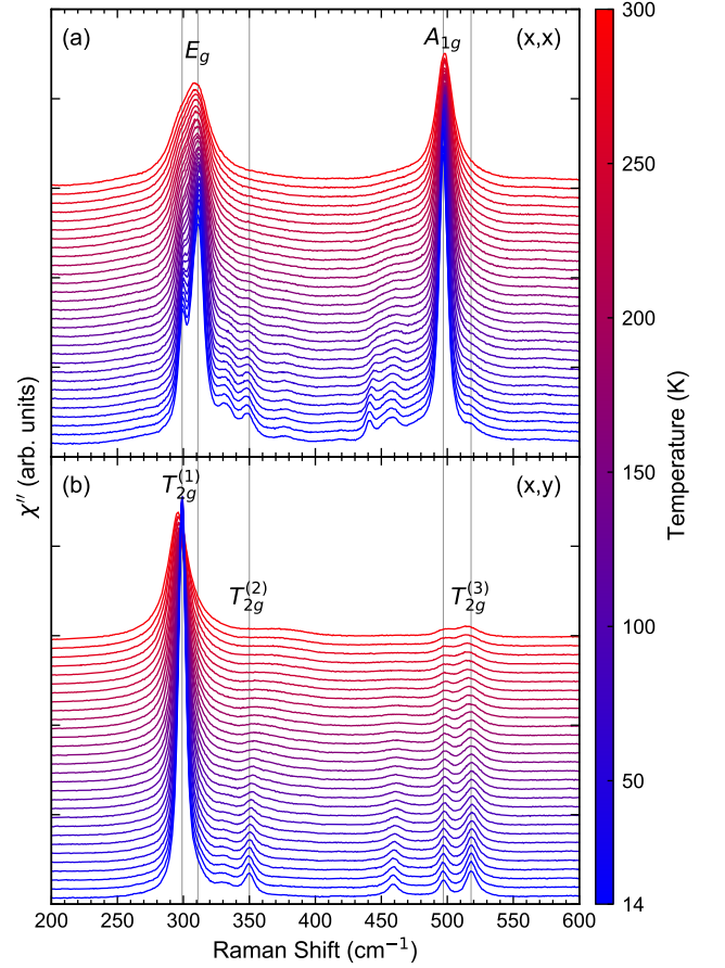
FIG. 2. Temperature dependence of the Raman scattering spectra of Pr 2 Zr 2 O 7 in (a) (x,x) channel and (b) (x,y) channel.
