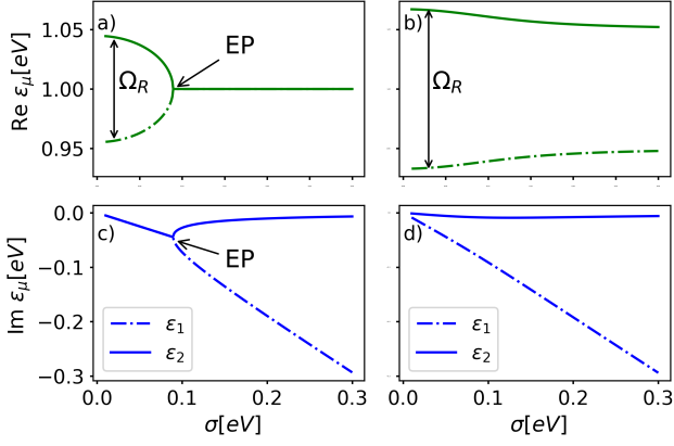
FIG. 2. (a,b) real and (c,d) imaginary parts of the eigenenergies in Eq. (15) of the effective non-Hermitian Hamiltonian for g = 0.001E_M and N = 2000 . (a,c) depicts the resonant system with E_C = E_M = 1\text{eV} and (b,d) depicts the off-resonant system with E_C = 1.05\text{eV} and E_M = 0.95\text{eV} .
