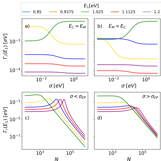
FIG. 6. Resonant transport rate in Eq. (47) as a function of disorder (a,b) and molecule number (c,d). The light-matter coupling is g = 0.001eV in all panels. The specific parameters are (a) E_C = E_M = 1eV, N = 2000 , (b) E_C = 1.05eV, E_M = 0.95eV, N = 2000 , (c) E_C = E_M = 1eV, \sigma = 0.04eV , (d) E_C = 1.05eV, E_M = 0.95eV, \sigma = 0.15eV . The disorder-averaged transport rate \bar{\Gamma} has the same functional dependence as the disorder-averaged relaxation rate \bar{\gamma} in Figs. 4 and 5, i.e., \bar{\Gamma} = \bar{\gamma}/N .
