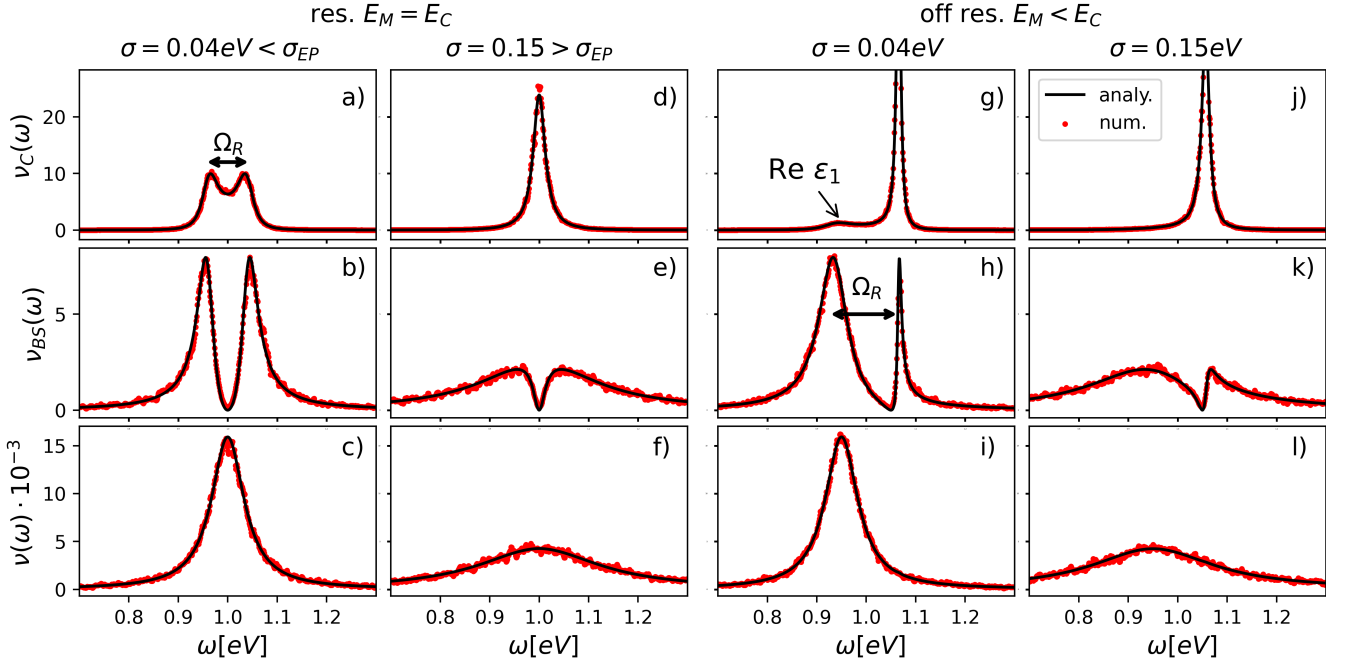
FIG. 3. Analytical and numerical calculations of the cavity LDOS (a,d,g,j), the bright-state LDOS (b,e,h,k), and the total density of states (c,f,i,l) as a function of energy. Overall system parameters are g = 0.001\text{eV} and N = 2000 . Specific parameters are E_C = E_M = 1\text{eV} , \sigma = 0.04\text{eV} < \sigma_{EP} in (a-c), E_C = E_M = 1\text{eV} , \sigma = 0.15\text{eV} > \sigma_{EP} , E_C = 1.05\text{eV} , E_M = 0.95\text{eV} , \sigma = 0.04\text{eV} < \sigma_{EP} in (d-e), E_C = 1.05\text{eV} , E_M = 0.95\text{eV} , \sigma = 0.04\text{eV} in (g-h) and E_C = 1.05\text{eV} , E_M = 0.95\text{eV} , \sigma = 0.15\text{eV} in (j-l). The LDOS in all panels are depicted in units of 1/\text{eV} .
