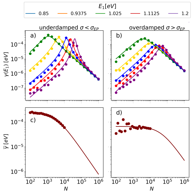
FIG. 5. Same as in Fig. 4 but as a function for molecule number N . The disorder in (a,c) is \sigma = 0.04eV and in (b,d) \sigma = 0.15eV .
