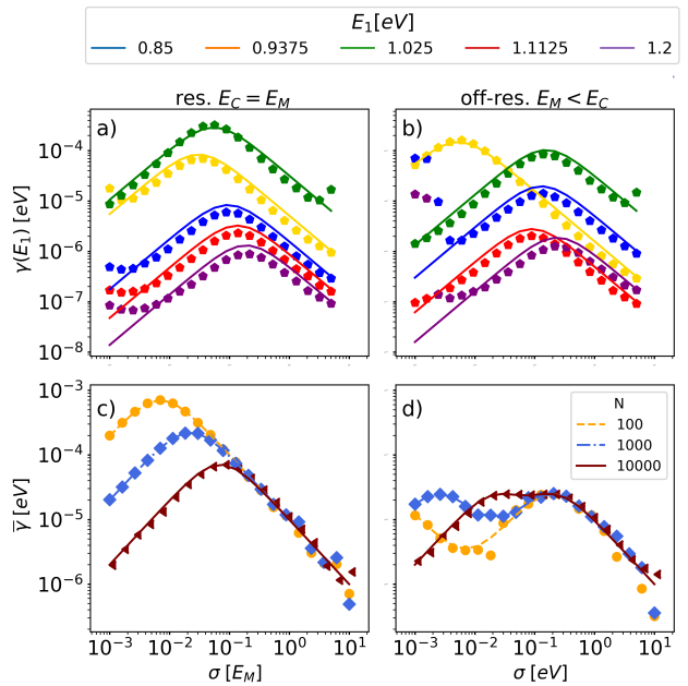
FIG. 4. (a,b) Energy-resolved relaxation rate \gamma(E_1) for the resonant system E_C = E_M = 1eV (a), and for the off-resonant system E_C = 1.05eV, E_M = 0.95eV (b). In both (a) and (b), g = 0.001eV and N = 2000 . (c,d) Disorder-averaged relaxation rate \bar{\gamma} for the same parameters as in (a,b) for different molecule numbers. Symbols represent the finite-size simulation to verify the analytical treatment, where the number of disorder samples M_S is such that M_S \cdot N = 10^6 .
