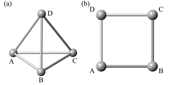
FIG. 4. Four-sublattice clusters in the shapes of (a) a tetrahedron and (b) a square.
