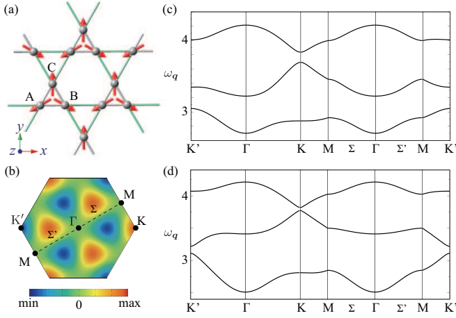
FIG. 8. (a) Breathing kagome lattice structure in the absence of the horizontal mirror plane under the polar point group C_{3v} . The arrows represent the magnetic moments to form the 120^\circ antiferromagnetic ordering. (b) The first Brillouin zone in (a). The color plot represents angle dependence of nonreciprocal magnons characterized by q_x(q_x^2 - 3q_y^2) , which is the same as that in Fig. 5(b). (c, d) The magnon band structures under the 120^\circ antiferromagnetic ordering for D' = 0.2 and J'^a = 0 (c) and D' = 0 and J'^a = 0.2 (d). The other parameters are set as J^\perp = 1 , J^z = 0.8 , D = -0.2 , J^a = 0.5 , and \gamma = 0.5 .
