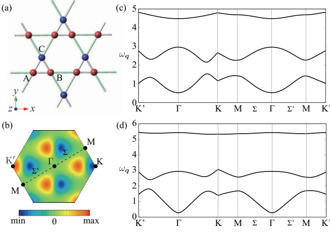
FIG. 7. Breathing kagome lattice structure under the point group D_{3h} . The red (blue) spheres represent the up (down) spins along the z direction. (b) The first Brillouin zone in (a). The color plot represents angle dependence of nonreciprocal magnons characterized by a linear combination of q_x(q_x^2 - 3q_y^2) and q_x(q_x^2 - q_y^2)(q_x^2 - 3q_y^2) . (c, d) The magnon band structures under the up-up-down magnetic ordering for D = 0.2 , J^a = 0 , and J^\parallel = -2 (c) and D = 0 , J^a = 0.5 , and J^\parallel = -2.4 (d). The other parameters are set as J^\perp = 0.9 , J^z = 1 , and \gamma = 0.5 .
