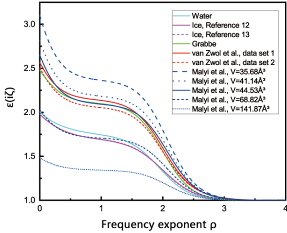
Figure 2. Permittivities of water (Cyan), ice (Magenta) and different silica materials (green, red and blue for Grabbe, 62 van Zwol et al. 60 and Malyi et al., 59 respectively) as functions of frequency exponent \rho . The frequency (in units of rad/s) \zeta is related to the exponent \rho = \log_{10} \zeta / \zeta_T , in which \zeta_T = 2\pi T is the n = 1 Matsubara frequency at the temperature of the triple-point of water, 273.16 K. The static dielectric constants for ice and water are, respectively, 91.5 and 88.2 as in Ref. 31, while for \text{SiO}_2 materials, their static values are 4.97, 4.32, 3.90, 2.62, and 1.69 from Ref. 59 for average volumes per \text{SiO}_2 V = 35.68, 41.14, 44.53, 68.82 , and 141.87 \text{ \AA}^3 , respectively, 3.80 for Grabbe, 62 and 3.90 for data set 1 and data set 2 of van Zwol et al. 60 The UV contributions of the ice dielectric function are modeled according to Refs. 72 and 73, which are, respectively, Reference 12 and Reference 13 quoted in Ref. 31.
