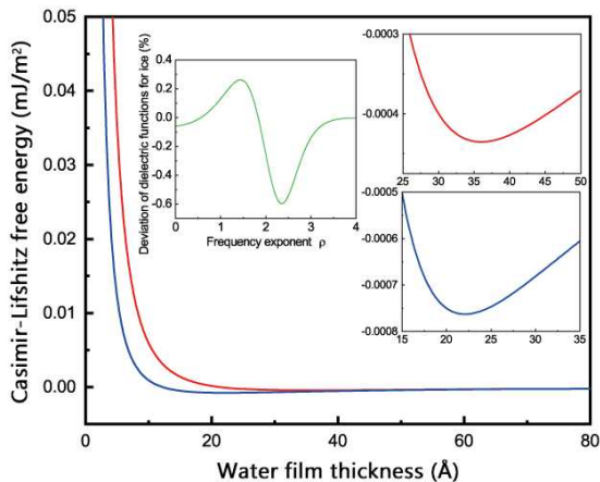
Figure 4. The Casimir-Lifshitz free energy of ice-water-vapor system as a function of water layer thickness. The results are obtained based on the data used by Elbaum and Schick in Ref. 31. The Casimir-Lifshitz free energies are plotted with the UV models for the ice dielectric function given by Reference 12 (red) and Reference 13 (blue) cited in Ref. 31, respectively. The behavior near the minima is shown in the right insets. The deviation between the dielectric functions for ice with different UV models, denoted \varepsilon_{12} and \varepsilon_{13} , is defined as (\varepsilon_{13} - \varepsilon_{12})/\varepsilon_{12} . Its dependence on the frequency exponent \rho is given in the middle inset.
