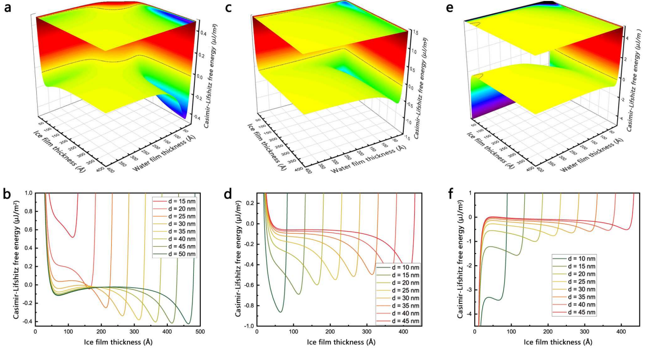
Figure 5. The Casimir-Lifshitz interaction free energy of silica-ice-water-vapor system at T = 273.16\text{K} with the average volume per \text{SiO}_2 being V = 35.68 \text{ \AA}^3 (a and b), V = 68.82 \text{ \AA}^3 (c and d) and V = 141.87 \text{ \AA}^3 (e and f). The dielectric functions for ice and water from Elbaum and Schick 31,32 are employed. For subfigures a, c and e (the corresponding projection of each 3D surface is given at the top), the dependence of free energy on the thicknesses of ice and water films are demonstrated. For subfigures b, d and f, the dependence of free energy as the function of ice film thickness, with the total thickness of ice and water layers fixed as d , are given.
