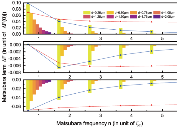
Figure 10. The Matsubara term as a function of the sum d of the water d_2 and ice d_3 thickness with d = 2d_2 . The systems investigated in Fig. 7 are studied in detail. Red triangles and blue circles are, respectively, plotted with overall scale adjusted for characteristic indices \eta and \tilde{\eta} defined in Eq. (8) and Eq. (9), with d = 2d_2 = 0.25\mu\text{m} .
