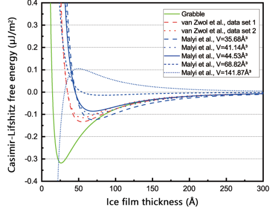
Figure 3. The Casimir-Lifshitz free energy per unit area for silica-ice-water configuration at the triple-point of water as a function of the thickness of ice layer. Its dependence on silica permittivities, thus the nanoporosities, is shown.
