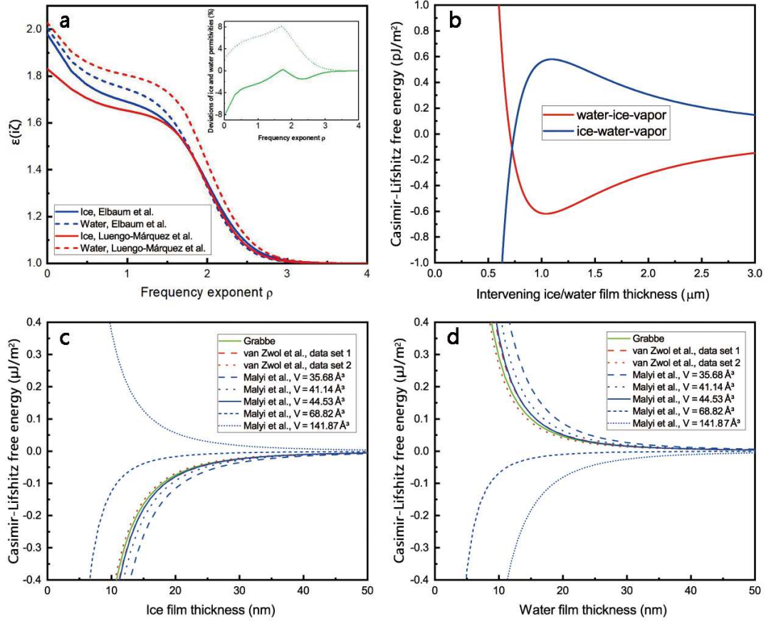
Figure 6. Previous work revisited with the latest dielectric functions for ice and water 55,56 near the triple point of water. (a) A comparison between the latest dielectric functions 55,56 (LM) and those used by Elbaum and Schick 31,32 (ES). The error between them is defined as (\varepsilon_{\text{LM}} - \varepsilon_{\text{ES}})/\varepsilon_{\text{LM}} . The dependence of errors on the frequency exponent \rho for ice (solid green) and water (dashed green) are given in the inset. (b) The Casimir-Lifshitz interaction free energies of ice-water-vapor and water-ice-vapor configurations evaluated with the latest data. Utilizing the new data, (c) and (d) demonstrate the dependences of free energy on ice and water films in the silica-ice-water and silica-water-ice configurations, respectively.
