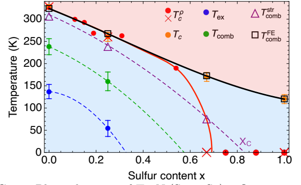
FIG. 3. Phase diagram of \text{Ta}_2\text{Ni}(\text{Se}_{1-x}\text{S}_x)_5 . Orange points: the symmetry breaking transition temperature T_c(x) obtained from the onset of phonon intensity 'leakage', Fig. 2(a). Red points and crosses: T_c^p(x) adapted from transport studies Refs. [19, 38]. For low sulfur concentration x , the soft excitonic mode, Fig. 2(b), would drive the transition at temperature T_{ex}(x) (blue points), that is enhanced to T_{comb}(x) by coupling to inert optical phonons (green points), and is further enhanced to T_{comb}^{str}(x) by coupling to the B_{2g} strain (purple triangles). For large x , the excitonic softening is suppressed, while a ferroelastic instability leads to a finite T_{FE}^{comb}(x) (black squares). In the absence of the lattice instability, a lattice-shifted electronic QPT would have occurred at x_c (dashed purple line). Additionally, in the same proximity, the band structure undergoes semimetal-to-semiconductor Lifschitz transition (see text).
