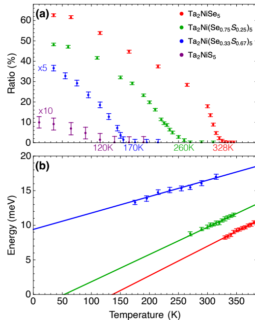
FIG. 2. The parameters deduced from the Raman response data, Fig. 1. (a) Integrated 'leakage' intensity into ac scattering geometries of the lowest-energy A_g phonon mode labeled in panels Fig. 1(e-h), normalized by the intensity in the dominant aa geometry. The mode's appearance in the ac scattering geometry below T_c implies the onset of symmetry breaking. (b) Excitonic energy \Omega_e(T) , Eq. (1) obtained from the Fano fits to the lineshapes in Fig. 1. Lines represent linear fits to the points.
