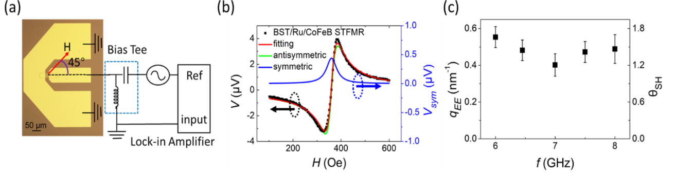
Fig. 3. Room temperature ST-FMR (a) Schematic of ST-FMR measurement for a BST/Ru/CoFeB system. (b) ST-FMR signal for the BST/Ru/CoFeB at 6.5 GHz which could be fitted well by a symmetric part (refer to the right axis) plus an anti-symmetric part. (c) Charge-to-spin conversion efficiency q_{EE} (defined in 2D) and \theta_{SH} (defined in 3D) are almost independent of frequency. \theta_{SH} > 1 at all frequencies, which suggests the 3D model can not explain the data.
