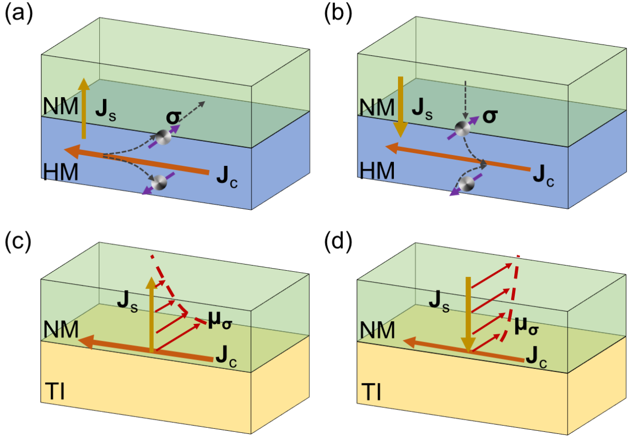
Fig. 1. (a) and (b) Schematics for the spin Hall effect (SHE) and inverse spin Hall effect (ISHE) in a heavy metal (HM) attached to another nonmagnetic metal (NM). SHE and ISHE are both based on spin-dependent scattering. When electrons with spin polarization \sigma get a velocity due to electrical or spin potential, they will be scattered into the orthogonal direction. (c) and (d) Schematic for the Edelstein effect (EE) and inverse Edelstein effect (IEE) in a topological insulator (TI) attached to a NM. Spin-momentum locked surface states in TI lead to a one-to-one correspondence between charge current J_c in TI and spin potential at the TI interface \mu_\sigma . Spin current J_s are related to \mu_\sigma by scattering and diffusion processes. Therefore, EE and IEE could be understood by two independent steps: intrinsic spin-momentum locking and extrinsic spin diffusion.
