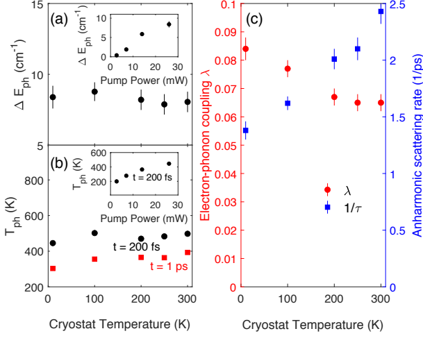
FIG. 4. Dependence on pump power, P , and T_{cryo} . (a) Phonon hardening at 200 fs ( E_{ph}(200 \text{ fs}) - E_{ph}(-1000 \text{ fs}) ) as a function of T_{cryo} at P = 27 \text{ mW} . Inset: Phonon hardening at T_{cryo} = 10 \text{ K} as a function of P . (b) Phonon temperature at 200 fs and 1 ps as a function of T_{cryo} at P = 27 \text{ mW} (fluence of 1.4 \text{ mJ/cm}^2 ). Note that T_{el} = T_{ph} at 1 ps. Inset: T_{ph} at 200 fs at T_{cryo} = 10 \text{ K} as a function of P . (c) Electron-phonon coupling constant \lambda together with the anharmonic scattering rate 1/\tau . See Supplementary Notes 2 and 3 for details on how \tau and \lambda were calculated [41]
