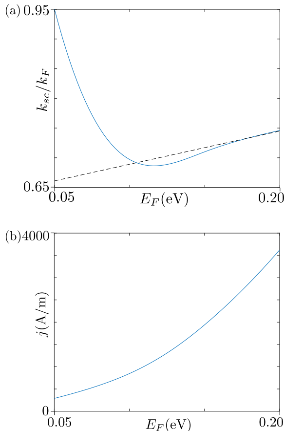
FIG. 5. (a) The critical value k_{sc} of the shift of the Fermi surface center vs. the Fermi energy E_F (eV). k_{sc} is defined as the minimum shift in which the angle of depletion \delta\theta > \pi/2 . The dashed line is the best linear fit of the large E_F dependence, given in the text. (b) The critical current j_{sc} vs. the Fermi energy E_F . The values of j_{sc} are obtained from k_{sc} according to Eq. (16).
