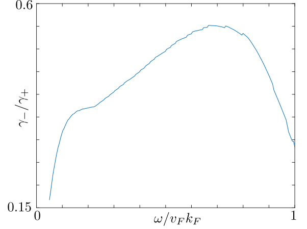
FIG. 3. Ratio of the damping factor \gamma of the redshifted ( \gamma_- ) and blueshifted ( \gamma_+ ) plasmon branches for E_F = 0.2 eV, k_s = 0.6 k_F , and \kappa = 1 .
