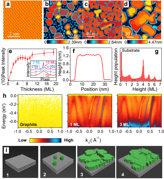
FIG. 1. Film growth and formation of magic-height islands. (a-d) STM images of clean graphite substrate (a) and Yb films with increasing nominal coverages: 2.5 ML (b), 6 ML (c), 9.5 ML (d). (e) The (1,0) peak intensity from RHEED as a function of film coverage, showing a slope change near 3 ML. Inset is a line cut of RHEED intensity, implying possibly a small lattice change between 2 ML and 15 ML. (f) Height profile of a 4 ML magic island along the dashed line shown in Fig. 1(b). (g) The island height distribution for a film with 2.5 ML coverage. (h) ARPES spectra for the substrate, and Yb films with 1 and 3 ML nominal coverages. (i) Cartoons illustrating different stages of film growth (stages 1-4).
