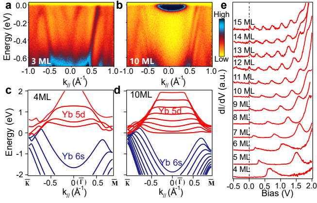
FIG. 2. Thickness-driven Lifshitz transition in Yb films. (a,b) ARPES spectra of a 3 ML film (a, the magic-height islands) and a 10 ML film (b, thick film). Here the 3 ML data is displayed, as the 4 ML data contains slight admixture from higher-thickness films due to inevitable roughness [27]. (c,d) The calculated band structures for 4 ML (c) and 10 ML (d) film along two high-symmetry directions, obtained from slab calculations. (e) The dI/dV curves of Yb films with different thicknesses, from STM measurements.
