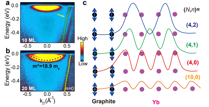
FIG. 4. The thickness ( N ) and subband ( n ) dependence of interfacial EPC coupling strength \lambda . (a,b) ARPES spectra for 10 ML (a) and 20 ML (b) film near E_F . The dispersion of the n = 0 QWS subband is extracted and highlighted. A yellow arrow indicates a possible kink for the 10 ML film. A parabolic fitting to the heavy electron band right below E_F is shown for the 20 ML film. (c) Simple drawings of the probability density of QWSs (labelled by (N, n) ) near the Yb/graphite interface. The probability density is shown as curves, with their zero positions offset vertically for clarity.
