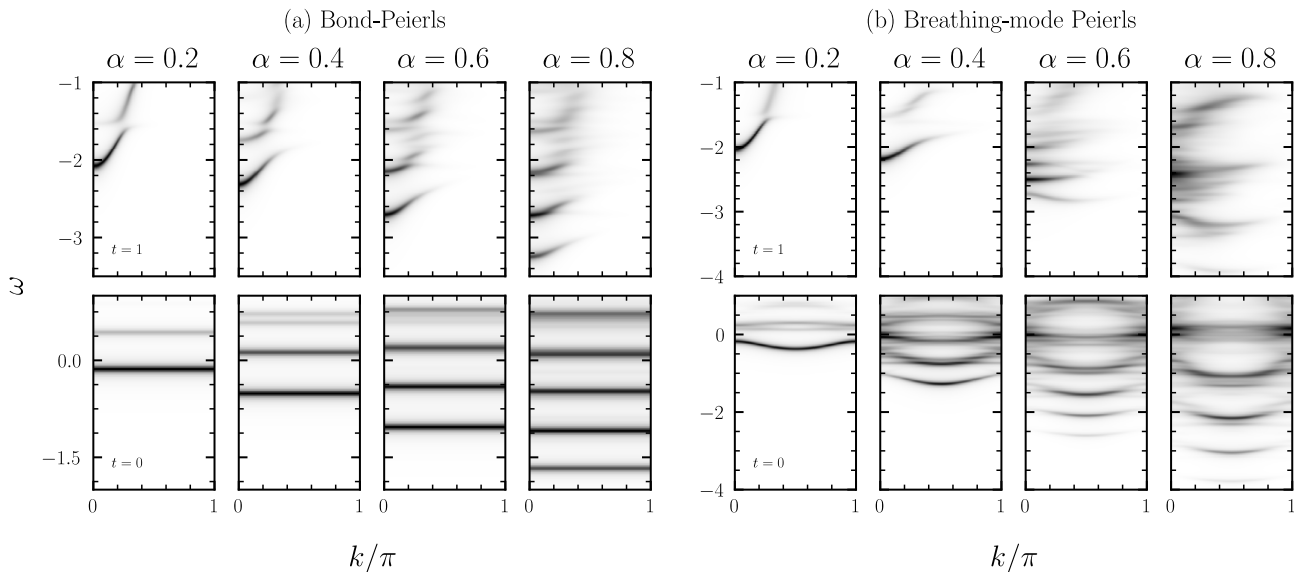
FIG. 3. Spectral functions for \Omega = 0.5 and broadening factor \eta = 0.04 of the (a) Bond- and (b) Breathing-Mode Peierls models with dispersionless phonons at t = 1 (top row) and t = 0 (bottom row) for a variety of different coupling strengths \alpha .
