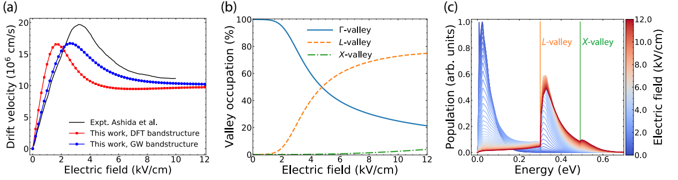
FIG. 3. (a) Velocity-field curve in GaAs at 300 K computed with DFT and GW band structures and compared with experimental data [66]. (b) Electronic valley occupations in GaAs as a function of applied electric field. The Brillouin zone regions defining the valleys are obtained from a 0.75 eV energy cutoff above the conduction band minimum. (c) Steady-state electron occupations as a function of conduction band energy and applied electric field. The L - and X -valley minima are shown with vertical lines.
