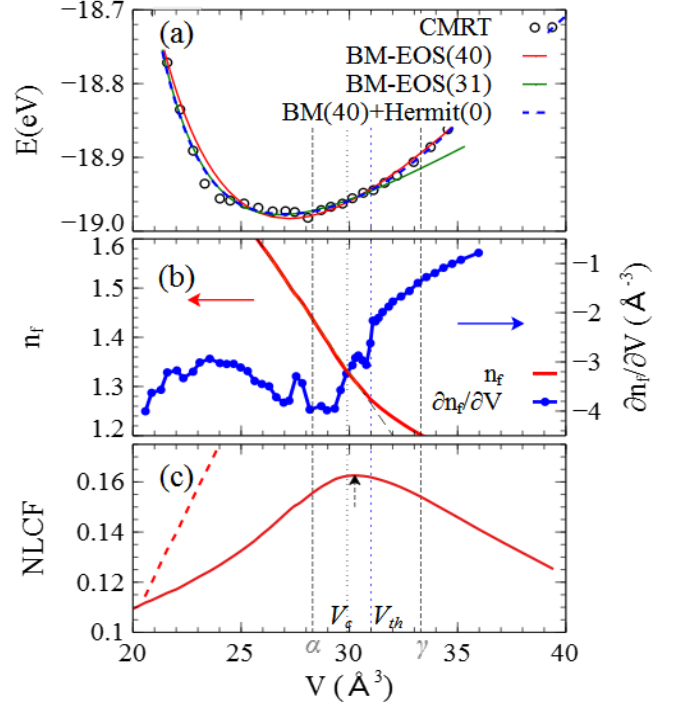
FIG. 3. (a) CMRT E-V curve and its different EOS fits, including a BM(40)+Hermit(0) fit over the whole volume range within 40\text{\AA}^3 and two BM-EOS fits in solid red over the same volume range and solid green for less than V_{th} . (b) volume dependence of n_f (solid red, left axis) and \partial n_f/\partial V (dotted solid blue, right axis), as well as a linear fit (dashed black) over part of n_f to show the relevant irregularities in \partial n_f/\partial V are due to error. (c) volume dependence of NLCF (solid red) and its weak interacting limit, 1/n_f (dashed red), down-shifted to give contrast against CMRT. The middle two vertical lines denote V_c and V_{th} respectively and the arrow in Panel (c) denotes V_{TP} .
