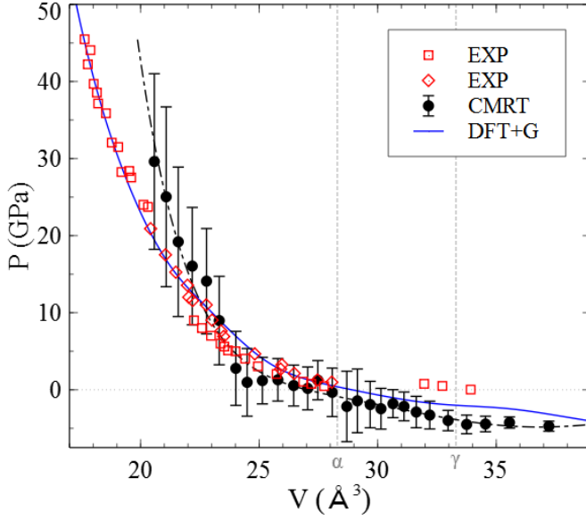
FIG. 2. The P-V data obtained from CMRT are compared against experiments[32, 33]. DFT+G at U=6\text{eV} with SOC[23] is also included as the 0K pressure reference. Error-bars of CMRT pressure are derived from those in total energy calculation.
