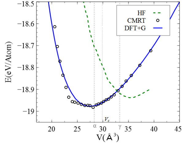
FIG. 1. E-V curves on fcc Ce calculated with nonmagnetic HF, DFT+G with U = 6 eV (upper right panel of Fig 1 in Ref [23]), and CMRT. Taking CMRT energy as the reference, arbitrary energy shifts are applied to HF and DFT+G for a best comparison with CMRT.
